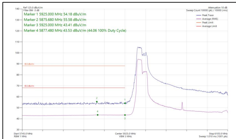
Figure 249 - 802.11ax HE160, RU 106-53P, SISO, Core 1 - 6025 MHz Band Edge Frequency 5925 MHz
