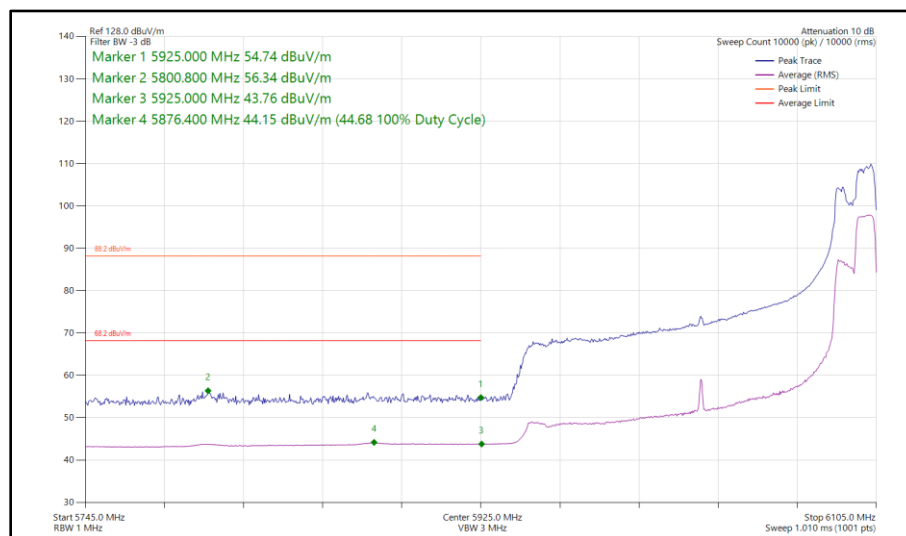
Figure 245 - 802.11ax HE160, RU 106-60S, SISO, Core 0 - 6025 MHz Band Edge Frequency 5925 MHz
