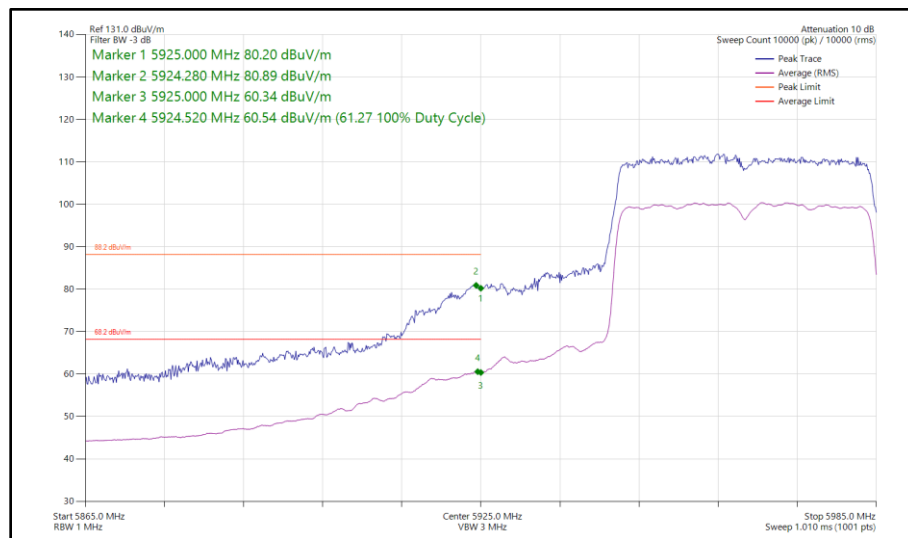
Figure 220 - 802.11ax HE40, SU, SDM, Core 0 - Core 1 - 5965 MHz Band Edge Frequency 5925 MHz
