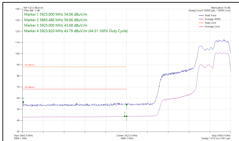
Figure 217 - 802.11ax HE40, RU 106-56, CDD, Core 0 - Core 1 - 5965 MHz Band Edge Frequency 5925 MHz
