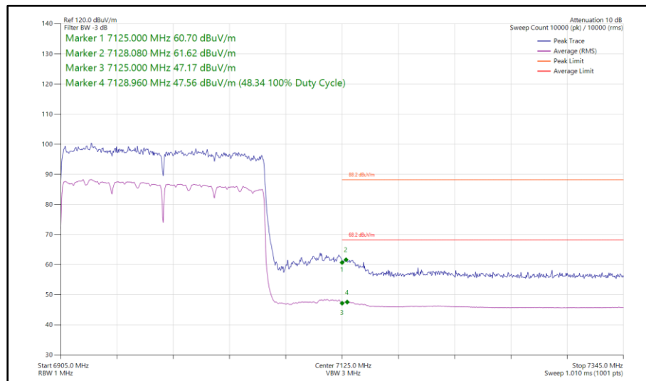
Figure 250 - 802.11ax HE160, SU, SISO, Core 1 - 6985 MHz Band Edge Frequency 7125 MHz
