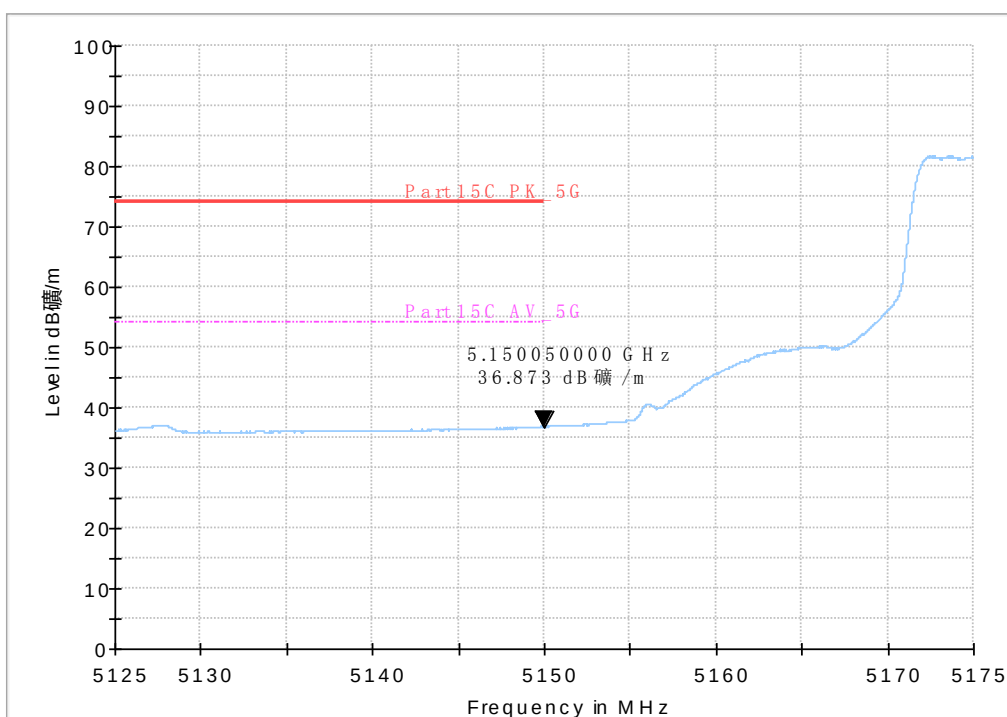
Fig. 31 Band Edges (802.11a, 5180MHz)
