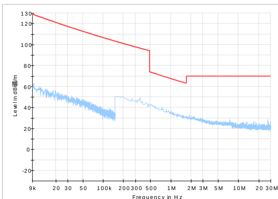
Fig. 52 Radiated Spurious Emission (9kHz-30MHz)
