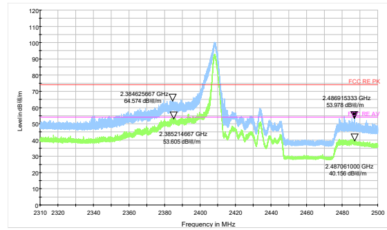
802.11ax HE40-Channel 4 Peak & Average
