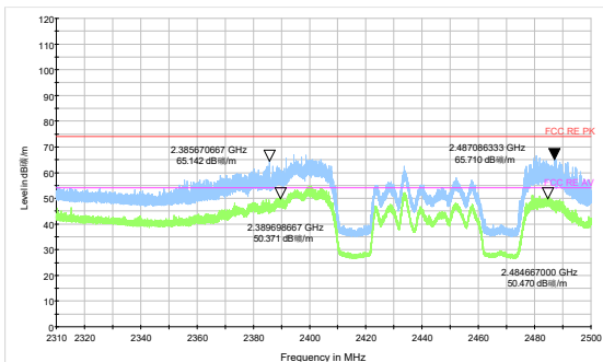
802.11ax HE40-Channel 7 Peak & Average
