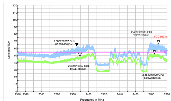
802.11ax HE40-Channel 8 Peak & Average
