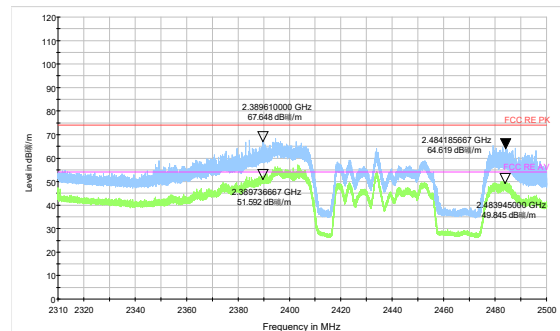
802.11ax HE40-Channel 6 Peak & Average
