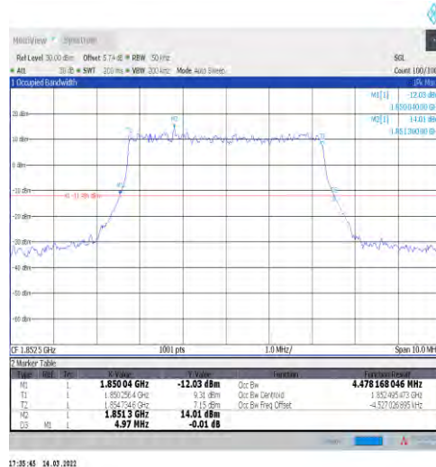
1-N2-15-5-L-2-DFT-PI2BPSK-Outer_Full-25@0-Ant1 -4.478-4.970-≤5-PASS
