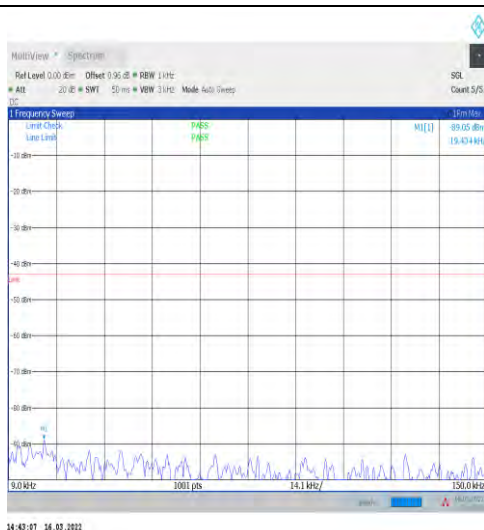
1-N2-15-20-H-1-DFT-PI2BPSK-Inner_1RB_Left-1@ 1-0.009-0.15-Ant1--89.05--43-PASS
