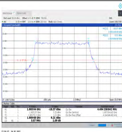
1-N2-15-5-H-5-DFT-256QAM-Outer_Full-25@0-Ant1 -4.494-5.070-≤5-PASS
