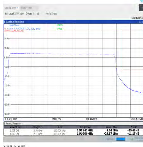
1-N2-15-5-H-6-CP-QPSK-Outer_Full-25@0-Ant1-seegraph-PASS-see graph
