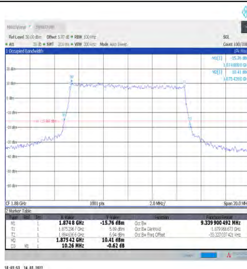
1-N2-15-10-M-8-CP-64QAM-Outer_Full-52@0-Ant1- 9.34-10.260-≤10-PASS
