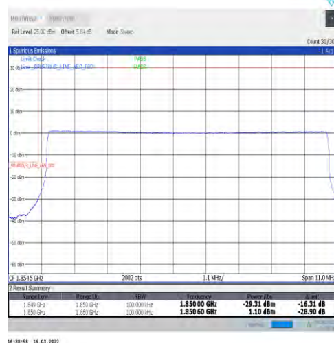
1-N2-15-10-L-6-CP-QPSK-Outer_Full-52@0-Ant1-seegraph-PASS-see graph
