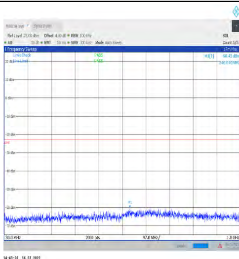
1-N2-15-20-H-1-DFT-PI2BPSK-Inner_1RB_Left-1@ 1-30-1000-Ant1--60.43--23-PASS
