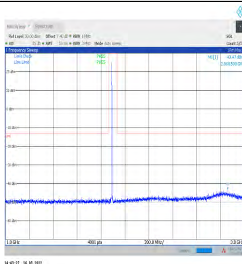
1-N2-15-20-H-1-DFT-PI2BPSK-Inner_1RB_Left-1@ -1000-3000-Ant1--43.47--13-PASS
