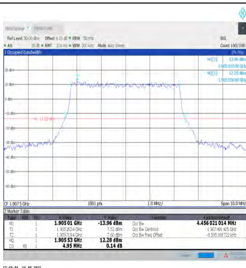
1-N2-15-5-H-3-DFT-16QAM-Outer_Full-25@0-Ant1- 4.456-4.950-≤5-PASS
