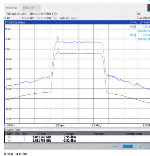
1-N2-15-20-L-2-CP-256QAM-Outer_Full-106@0-Ant 1-11.77-100%-0.00-11.77-PASS-≤13
