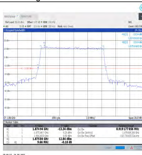
1-N2-15-10-M-2-DFT-PI2BPSK-Outer_Full-50@0-An t1-8.919-9.660-≤10-PASS
