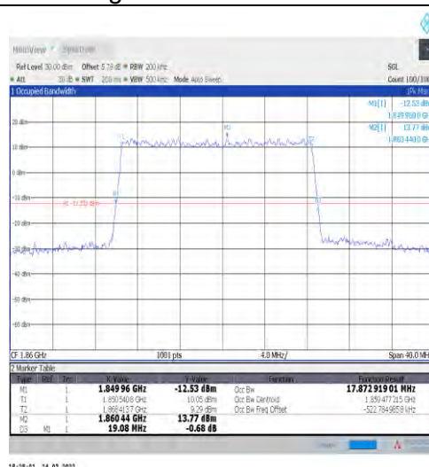
1-N2-15-20-L-1-DFT-QPSK-Outer_Full-100@0-Ant1- 17.873-19.080-≤20-PASS
