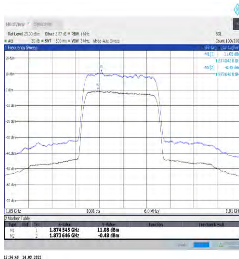
1-N2-15-20-M-1-DFT-256QAM-Outer_Full-100@0-A nt1-11.56-100%-0.00-11.56-PASS-≤13
