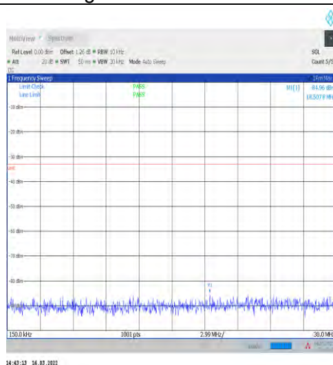
1-N2-15-20-H-1-DFT-PI2BPSK-Inner_1RB_Left-1@ -0.15-30-Ant1--84.96--33-PASS
