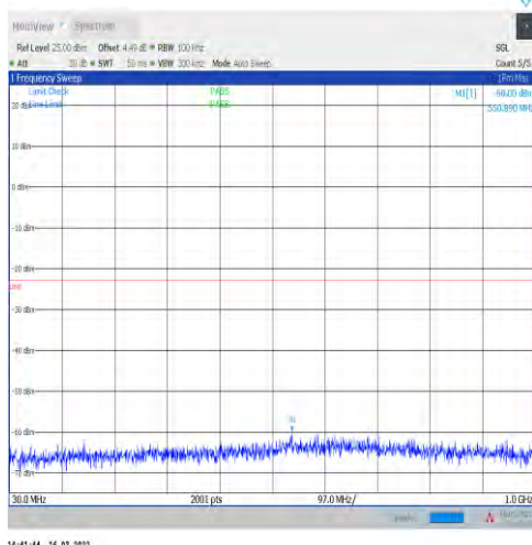
1-N2-15-20-M-1-DFT-PI2BPSK-Inner_1RB_Left-1@ 1-30-1000-Ant1--60.00--23-PASS
