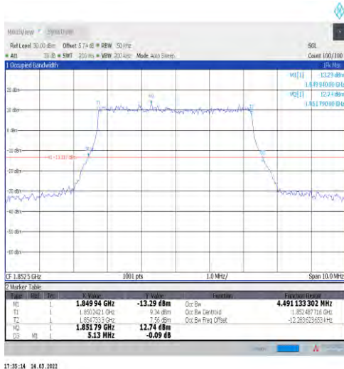
1-N2-15-5-L-1-DFT-QPSK-Outer_Full-25@0-Ant1-4. 491-5.130-≤5-PASS
