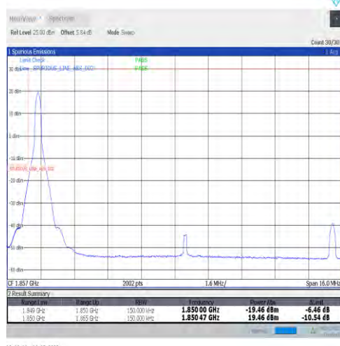
1-N2-15-15-L-4-CP-QPSK-Edge_1RB_Left-1@0-Ant1-seegraph-PASS-see graph
