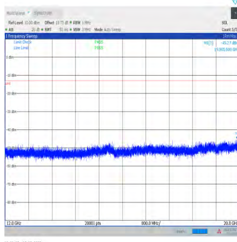
1-N2-15-20-M-1-DFT-PI2BPSK-Inner_1RB_Left-1@1 -12000-20000-Ant1--45.27--13-PASS
