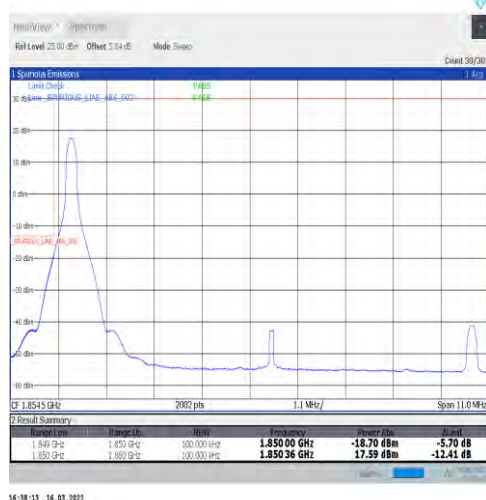
1-N2-15-10-L-4-CP-QPSK-Edge_1RB_Left-1@0-Ant1-seegraph-PASS-see graph
