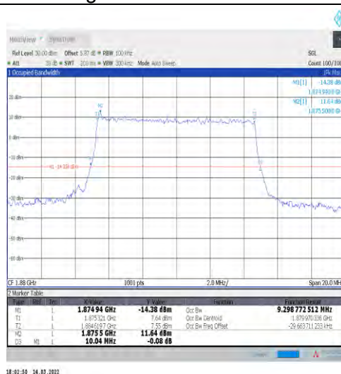
1-N2-15-10-M-6-CP-QPSK-Outer_Full-52@0-Ant1-9. 299-10.040-≤10-PASS
