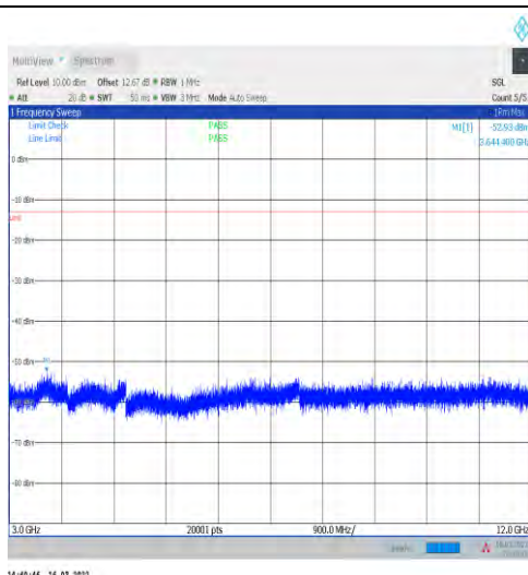
1-N2-15-20-L-1-DFT-PI2BPSK-Inner_1RB_Left-1@1 -3000-12000-Ant1--52.93--13-PASS
