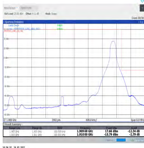
1-N2-15-5-H-5-CP-QPSK-Edge_1RB_Right-1@24-Ant1-seegraph-PASS-see graph
