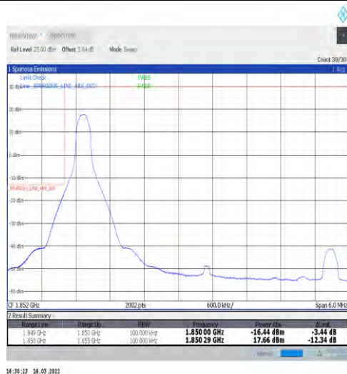
1-N2-15-5-L-4-CP-QPSK-Edge_1RB_Left-1@0-Ant1-seegraph-PASS-see graph
