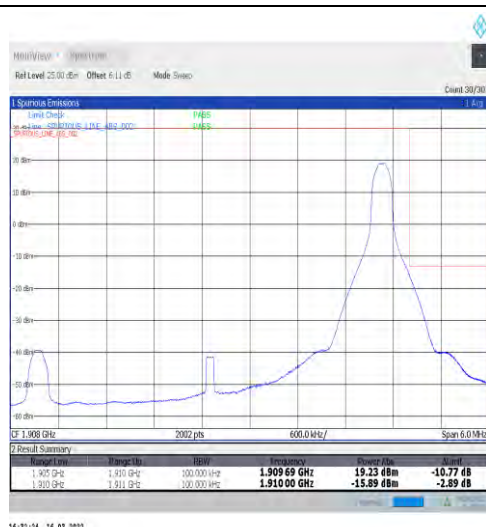
1-N2-15-5-H-2-DFT-PI2BPSK-Edge_1RB_Right-1@24-Ant1-seegraph-PASS-see graph
