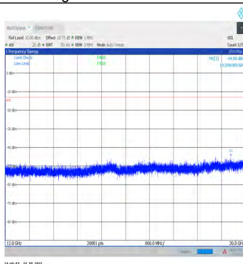
1-N2-15-20-L-1-DFT-PI2BPSK-Inner_1RB_Left-1@1 12000-20000-Ant1--44.90--13-PASS
