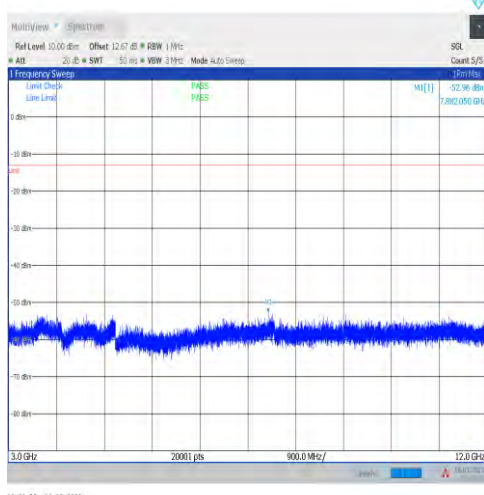
1-N2-15-20-M-1-DFT-PI2BPSK-Inner_1RB_Left-1@ 1-3000-12000-Ant1--52.96--13-PASS
