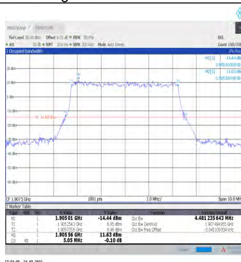
1-N2-15-5-H-4-DFT-64QAM-Outer_Full-25@0-Ant1- 4.481-5.050-≤5-PASS
