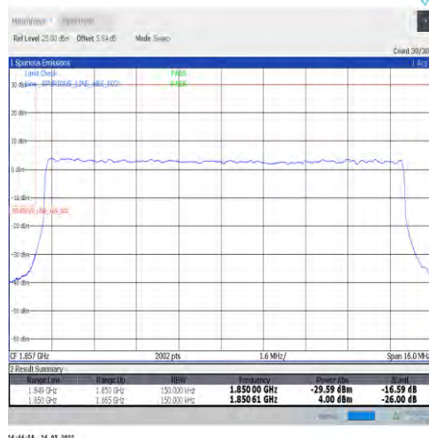
1-N2-15-15-L-3-DFT-PI2BPSK-Outer_Full-75@0-Ant1-seegraph-PASS-see graph
