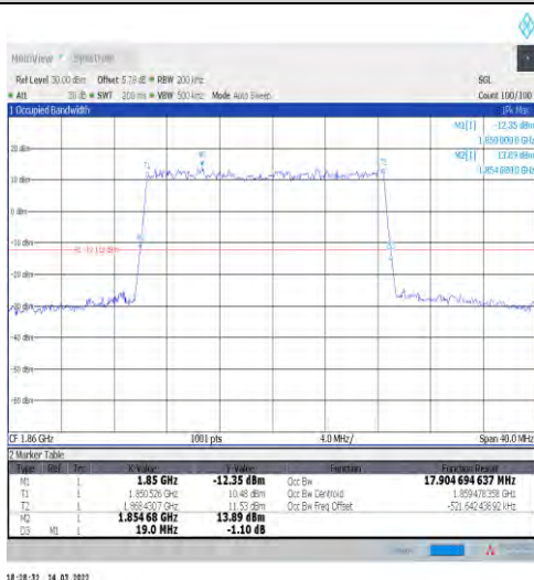
1-N2-15-20-L-2-DFT-PI2BPSK-Outer_Full-100@0-Ant1- 17.905-19.000-≤20-PASS
