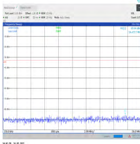
1-N2-15-20-M-1-DFT-PI2BPSK-Inner_1RB_Left-1@1 -0.15-30-Ant1--85.06--33-PASS
