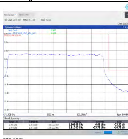
1-N2-15-5-H-3-DFT-PI2BPSK-Outer_Full-25@0-Ant1-seegraph-PASS-see graph
