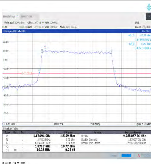
1-N2-15-10-M-7-CP-16QAM-Outer_Full-52@0-Ant1- 9.288-10.080-≤10-PASS
