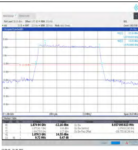
1-N2-15-10-M-1-DFT-QPSK-Outer_Full-50@0-Ant1- 8.937-9.720-≤10-PASS
