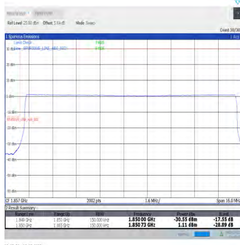
1-N2-15-15-L-6-CP-QPSK-Outer_Full-79@0-Ant1-seegraph-PASS-see graph
