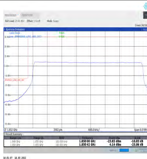
1-N2-15-5-L-6-CP-QPSK-Outer_Full-25@0-Ant1-seegraph-PASS-see graph
