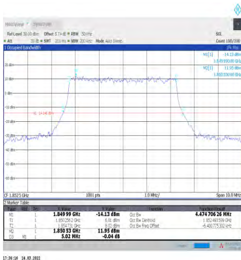
1-N2-15-5-L-3-DFT-16QAM-Outer_Full-25@0-Ant1- 4.475-5.020-≤5-PASS
