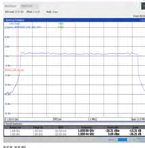
1-N2-15-10-L-3-DFT-PI2BPSK-Outer_Full-50@0-Ant1-seegraph-PASS-see graph
