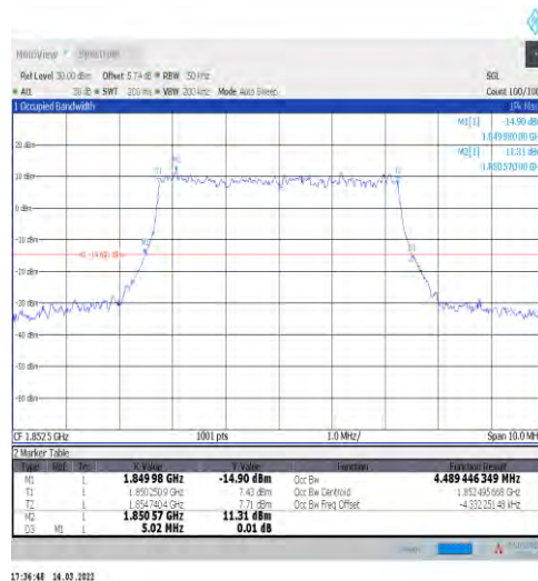
1-N2-15-5-L-4-DFT-64QAM-Outer_Full-25@0-Ant1-4 .489-5.020-≤5-PASS
