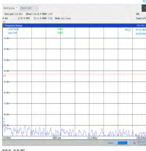
1-N2-15-20-M-1-DFT-PI2BPSK-Inner_1RB_Left-1@1 1-0.009-0.15-Ant1--87.35--43-PASS
