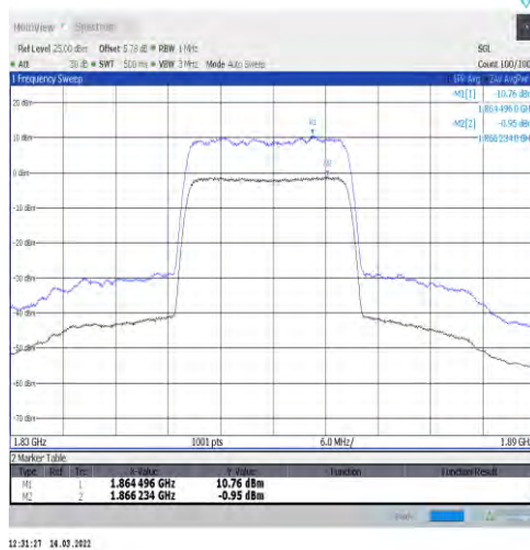
1-N2-15-20-L-1-DFT-256QAM-Outer_Full-100@0-Ant t1-11.71-100%-0.00-11.71-PASS-≤13
