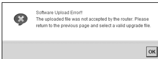
Figure 136 Error Message
