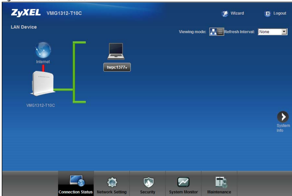
Figure 6 Connection Status
