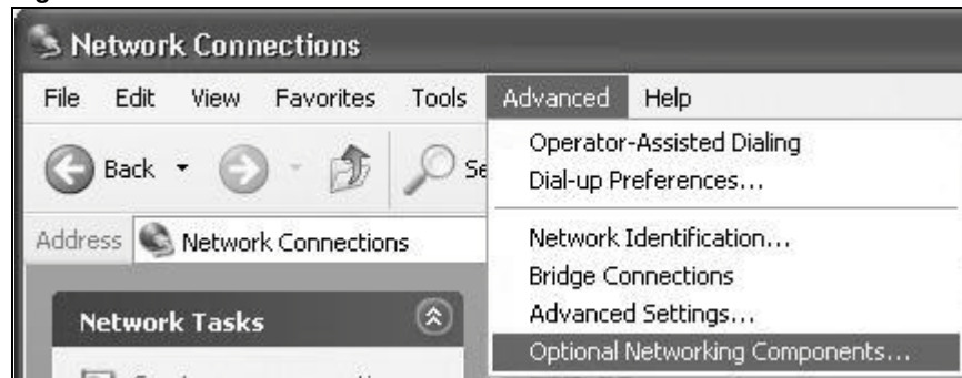
Figure 62 Network Connections
