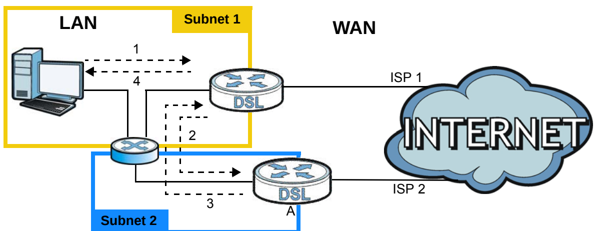
Figure 115 IP Alias
