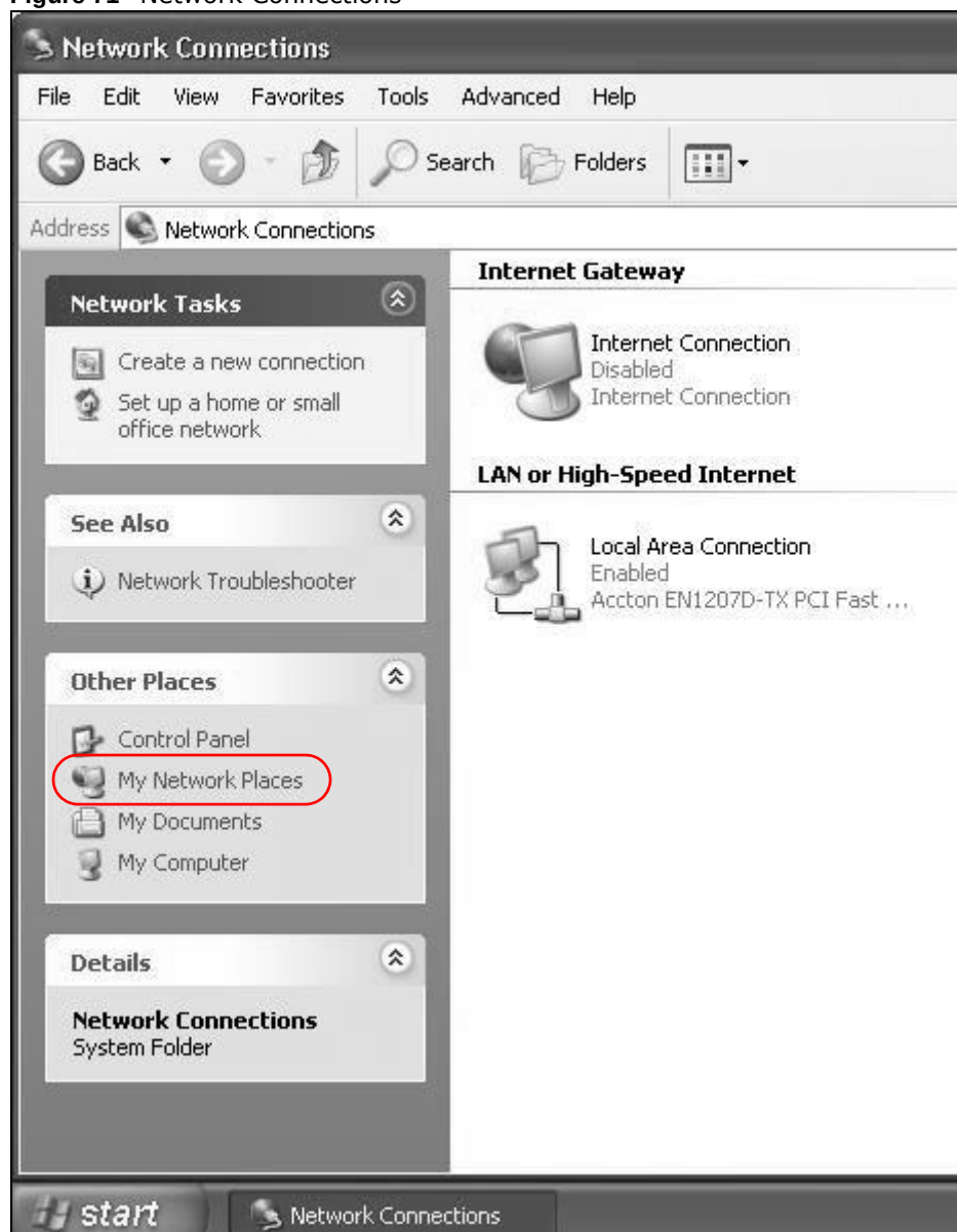
Figure 71 Network Connections
