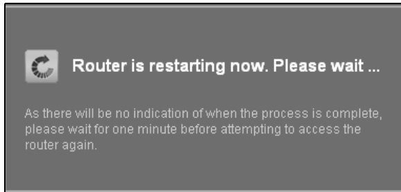
Figure 134 Firmware Uploading
