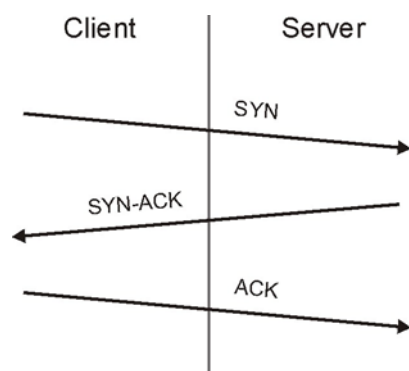
Figure 111 Three-Way Handshake
