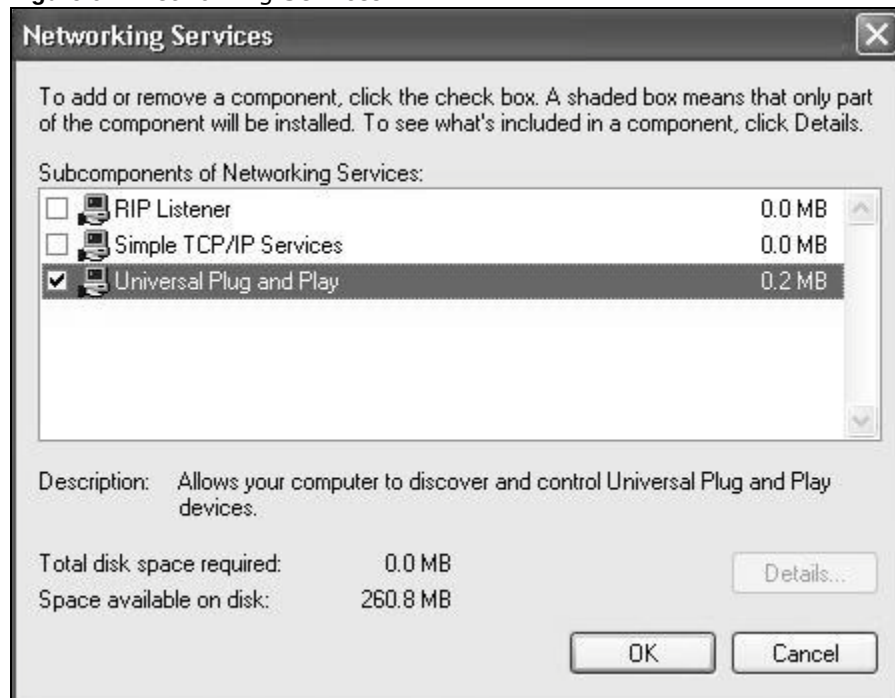
Figure 64 Networking Services
