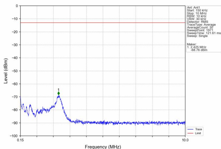
Band25 3MHz 16QAM LCH 1851.5MHz RB 1 0 NTV
