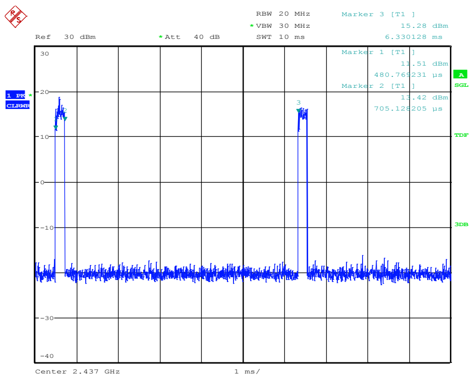
Plot 5: Duty Cycle-WLAN 2.4 GHz-g Mode | 20 MHz | 54Mbit | Ch 6 (2437 MHz)
