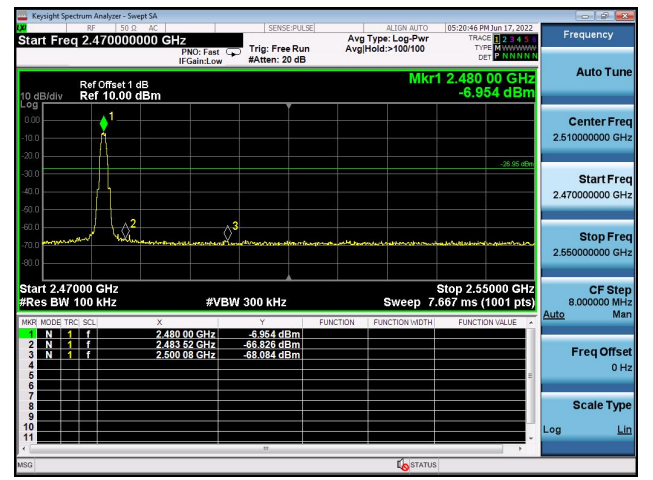
Right bandedge
