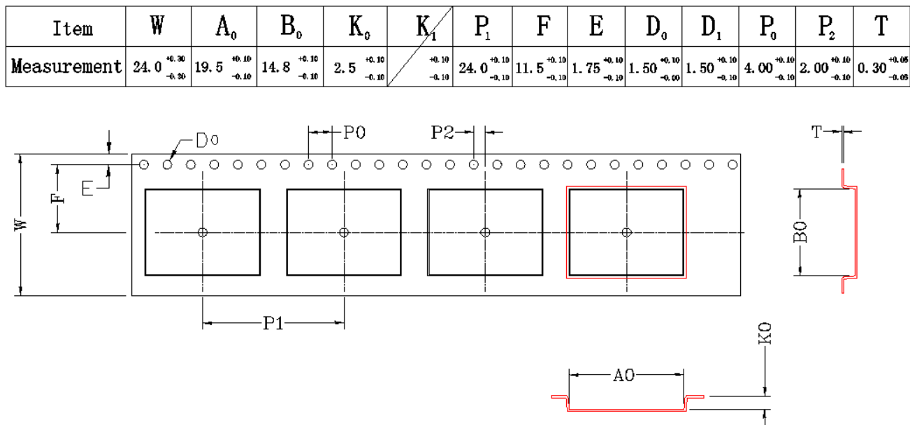
Figure 10. CYBLE-2X20XX-X1 Tape Dimensions
