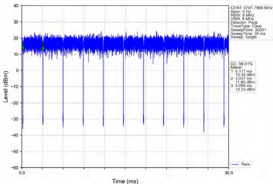
802.11ax(HE20)_MCH_5785MHz_RU52_Mid_Ant2_NTNV
