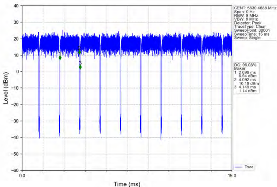
802.11ax(HE20)_HCH_5825MHz_RU106_Right_Ant2_NTNV
