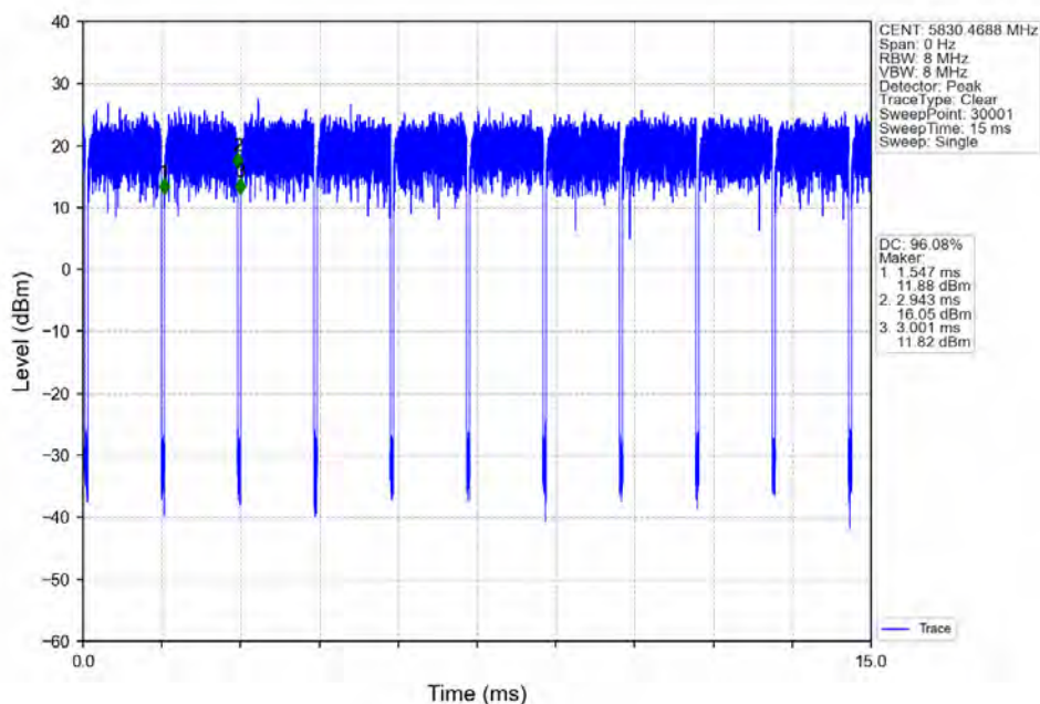
802.11ax(HE20)_HCH_5825MHz_RU106_Right_Ant1_NTNV
