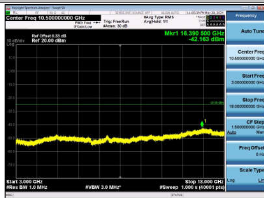
7-7-20MHz-20MHz-QPSK-QPSK-21152-21350-1RB#0-0R B#0-3000~18000MHz-PASS
