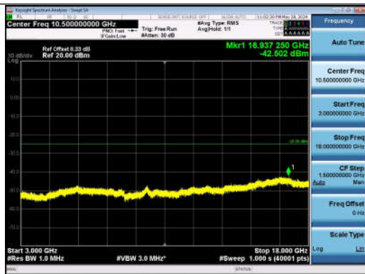
7-7-20MHz-20MHz-QPSK-QPSK-21001-21199-1RB#0-0R B#0-3000~18000MHz-PASS
