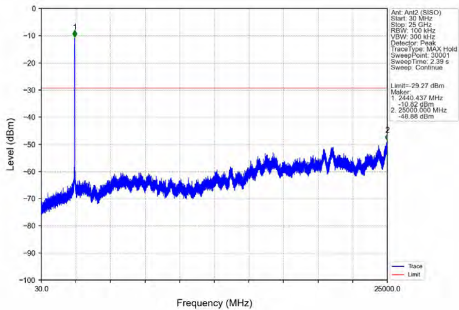
802.11ax(HEW40)_MCH_2437MHz_Ant2 (SISO)_NTNV
