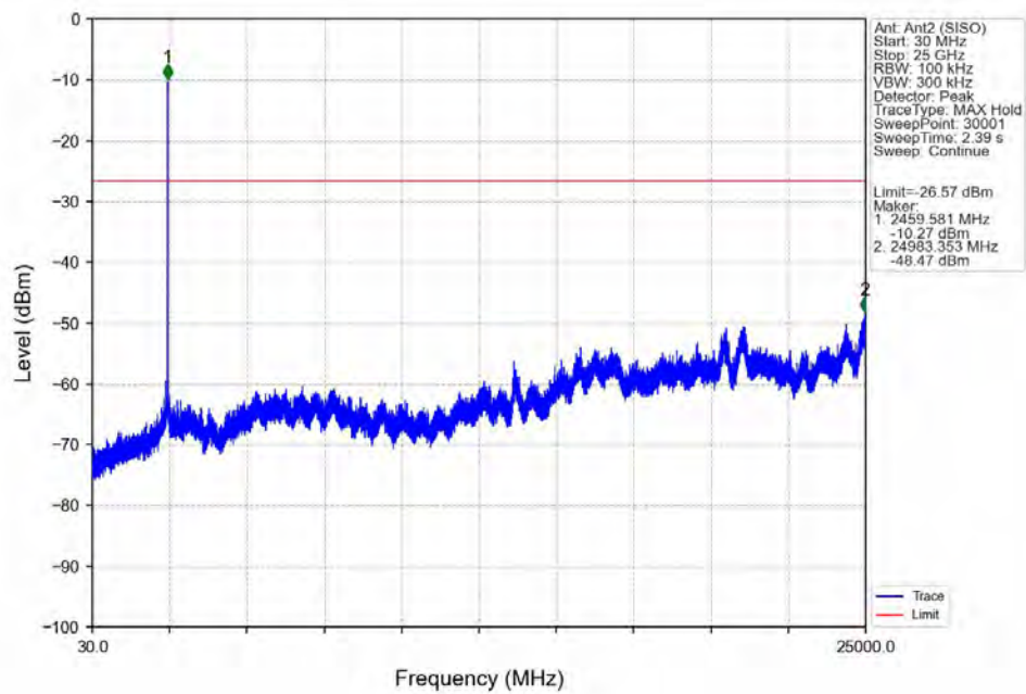
802.11ax(HEW20)_HCH_2462MHz_Ant2 (SISO)_NTNV
