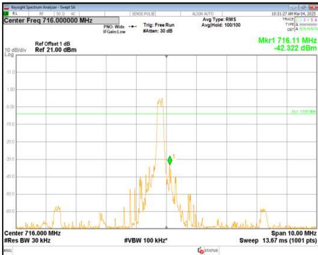
Band12 QPSK Channel=23178 nTones=1@11 Spacing=15kHz
