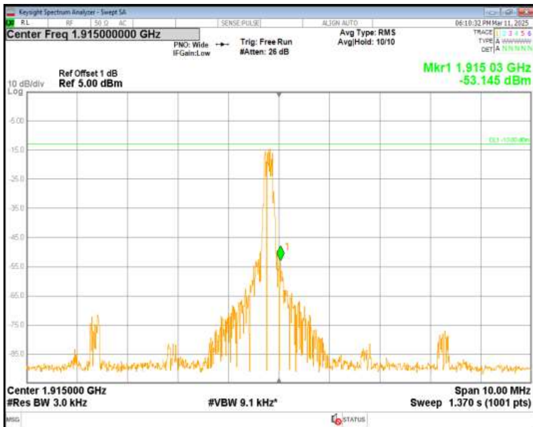
Band25 QPSK Channel=26688 nTones=1@11 Spacing=15kHz
