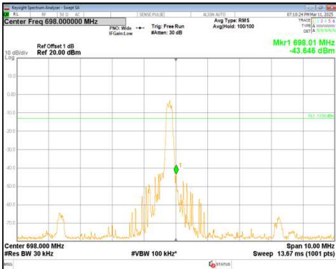
Band71 QPSK Channel=133470 nTones=1@11 Spacing=15kHz
