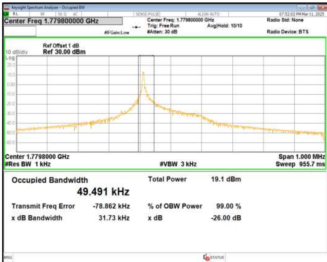
Band66 QPSK Channel=131974 nTones=1@0 Spacing=3.75kHz
