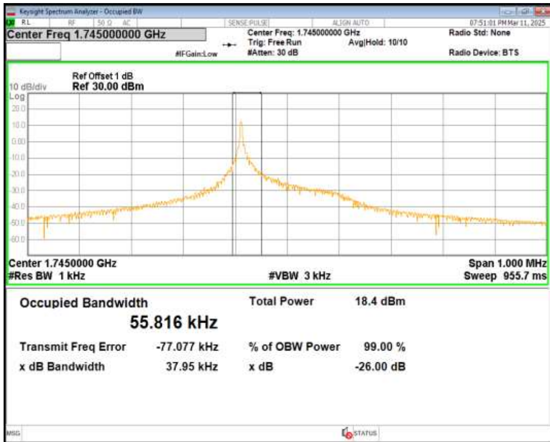
Band66 BPSK Channel=132670 nTones=1@0 Spacing=3.75kHz
