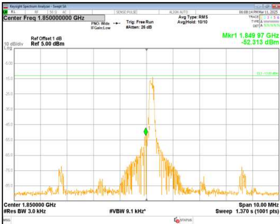
Band25 QPSK Channel=26042 nTones=1@0 Spacing=15kHz
