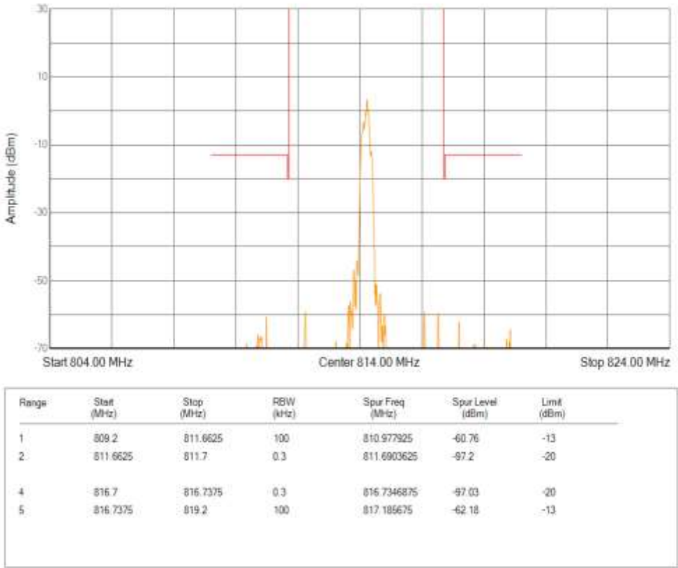
Band26 QPSK Channel=26692 nTones=1@0 Spacing=15kHz
