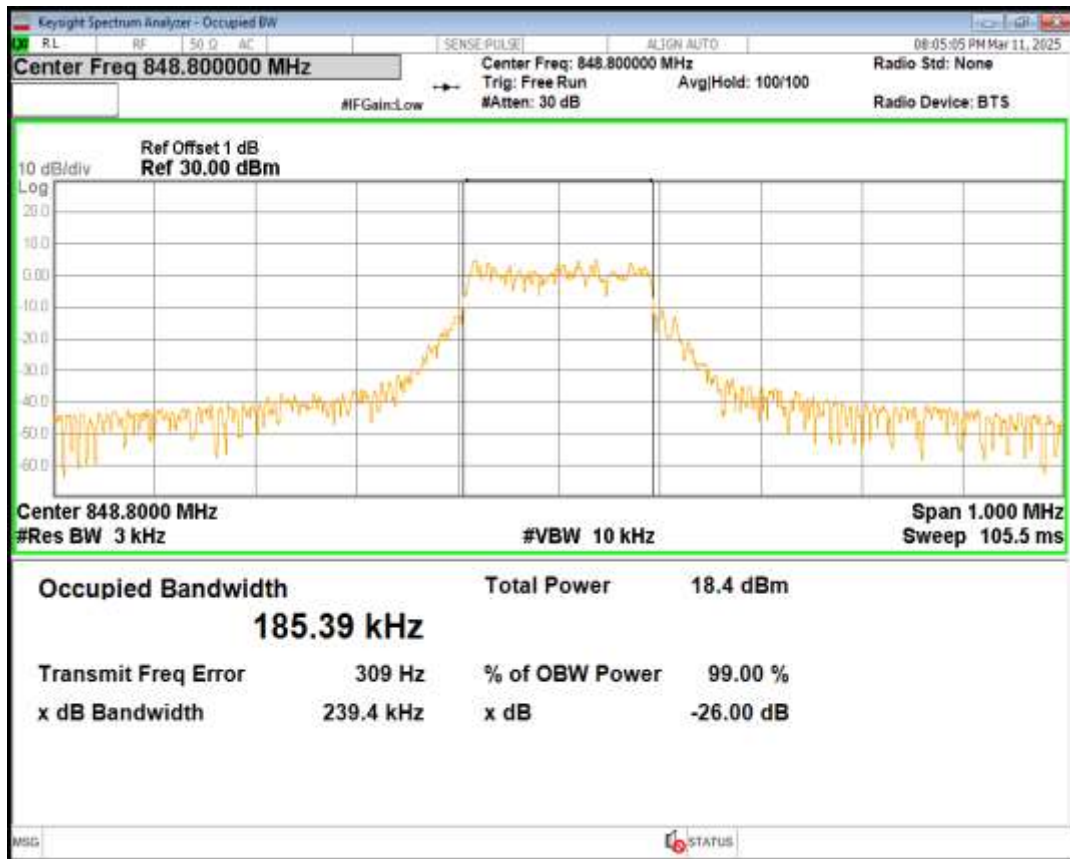
Band26 QPSK Channel=27038 nTones=1@0 Spacing=15kHz
