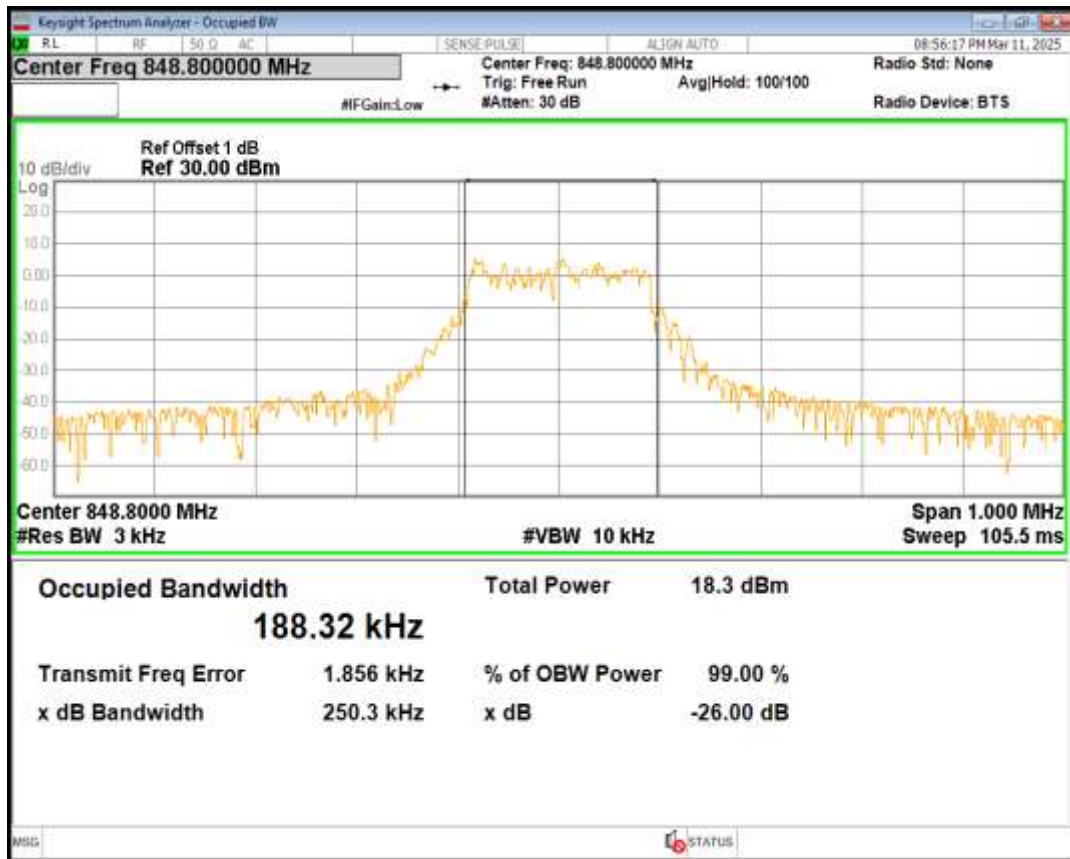
Band5 QPSK Channel=20648 nTones=1@0 Spacing=15kHz
