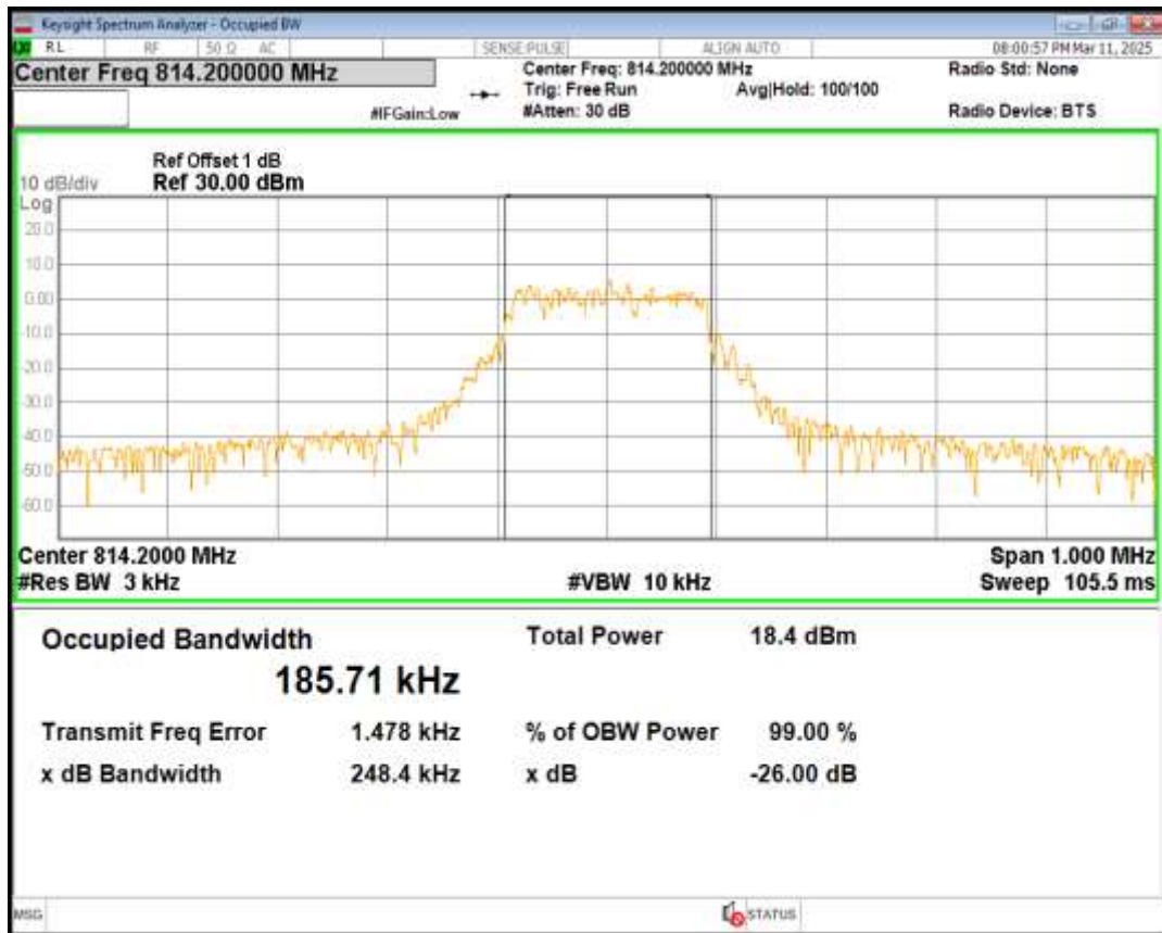
Band26 QPSK Channel=26692 nTones=1@0 Spacing=15kHz
