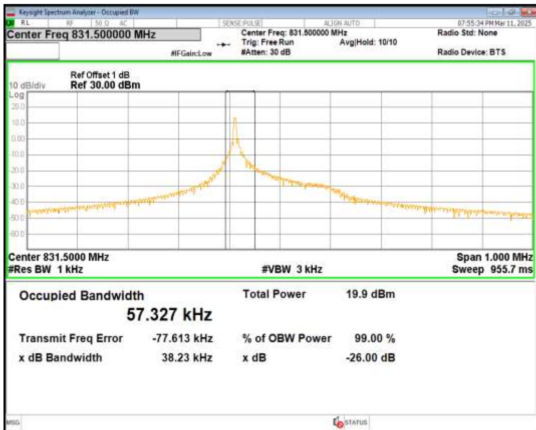
Band26 BPSK Channel=27038 nTones=1@0 Spacing=3.75kHz
