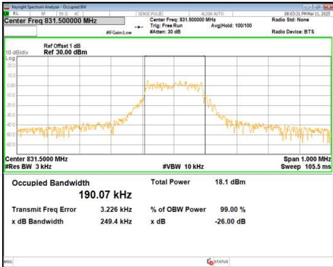
Band26 QPSK Channel=26865 nTones=1@0 Spacing=15kHz
