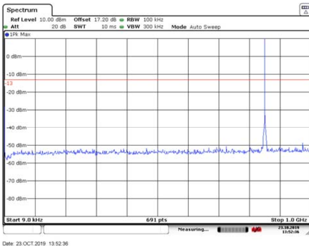
GSM 850 CH-High 9KHz ~ 1GHz
