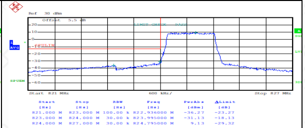
FDD26(PART 22)LowRange_1.4MHz_QPSK_FullRB_LowRange
