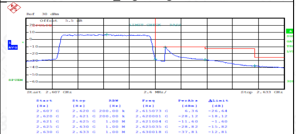
TDD38HighRange_10MHz_QPSK_FullRB _HighRange
