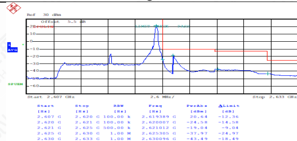
TDD38HighRange_10MHz_QPSK_1RB_HighRan ge
