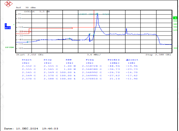
TDD38LowRange_20MHz_QPSK_1RB_LowRange
