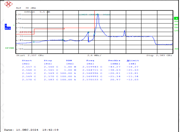
TDD38LowRange_15MHz_QPSK_1RB_LowRange
