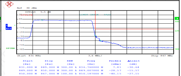
FDD26(PART 22)HighRange_15MHz_QPSK_FullRB_HighRange
