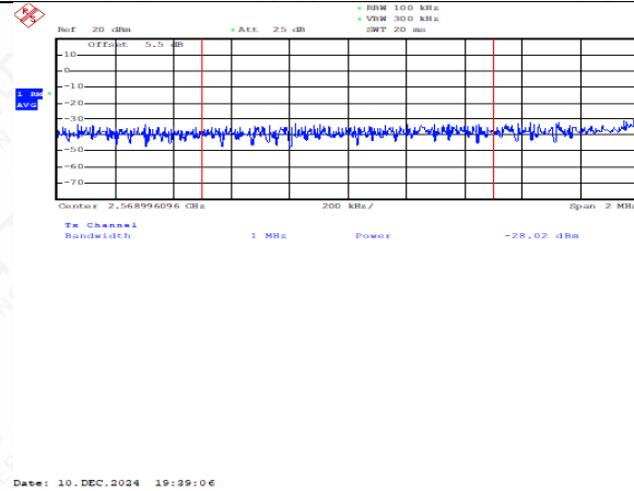
TDD38LowRange_10MHz_QPSK_FullRB _LowRange
