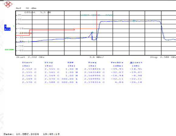
TDD38LowRange_15MHz_QPSK_FullRB _LowRange
