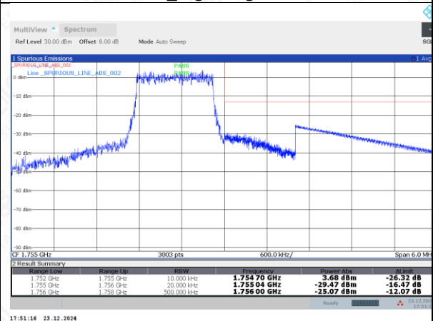
FDD04HighRange_1.4MHz_QPSK_FullRB_HighRange
