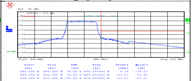
FDD26(PART 22)HighRange_1.4MHz_QPSK_FullRB_HighRange
