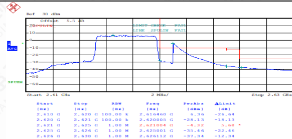
TDD38HighRange_5MHz_QPSK_FullRB _HighRange
