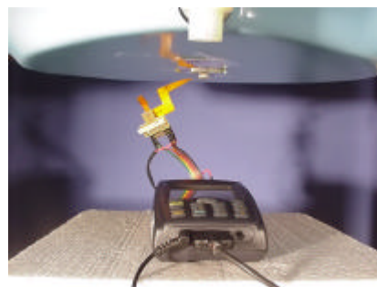
SAR Measurement Test Setup
