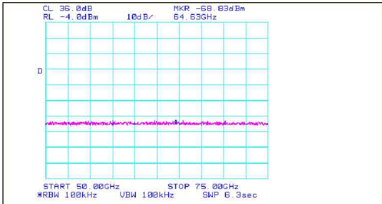
Graph 15. Radiated Spurious Emissions Test Results, 50 GHz to 75 GHz
