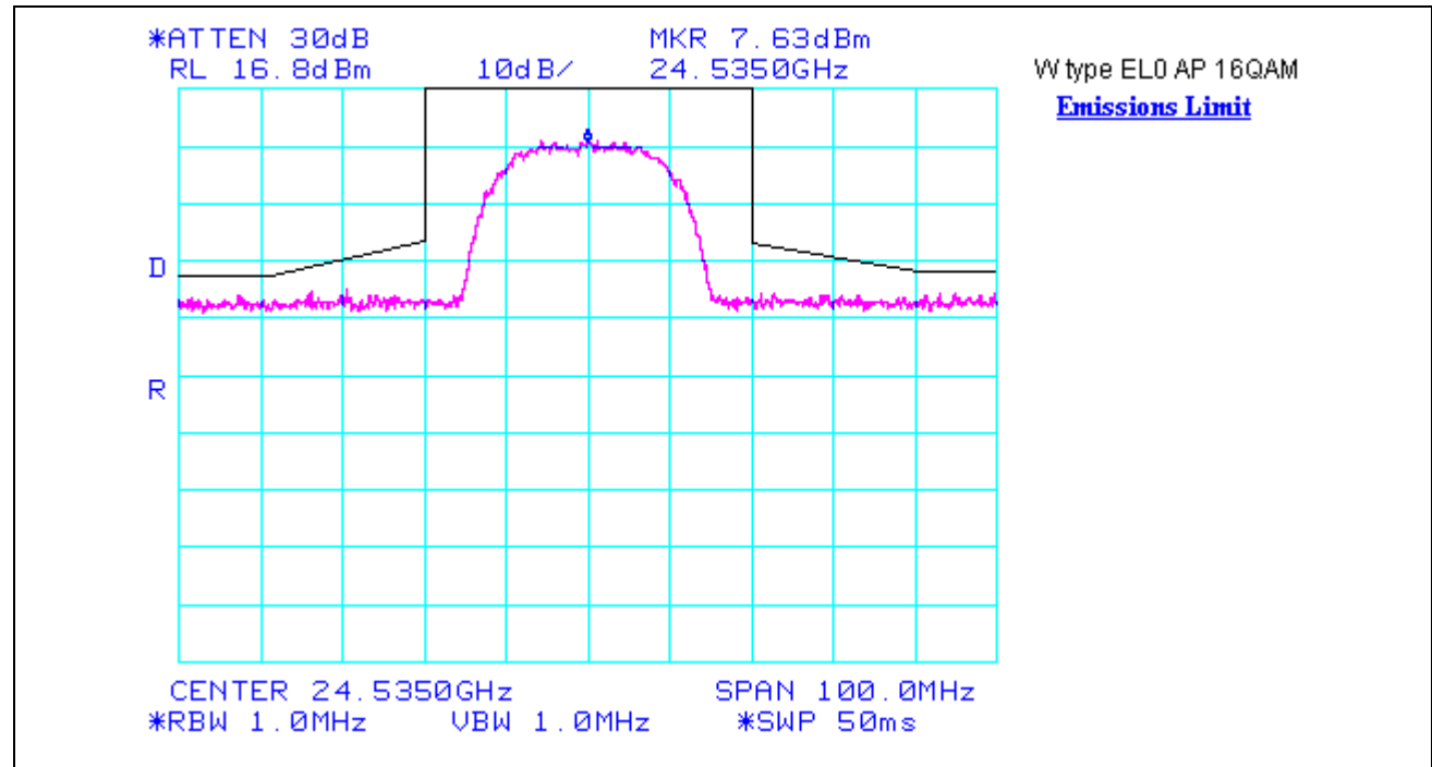
Graph 5. Emissions Limitation Test Result, 16 QAM
