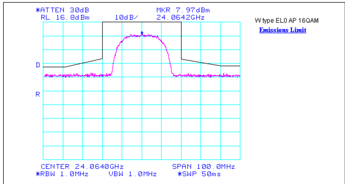
Graph 6. Emissions Limitation Test Result, 16 QAM
