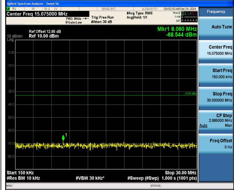
Band2_3MHz_16QAM_19185_1RB#14_0.15~30_0.15~30
