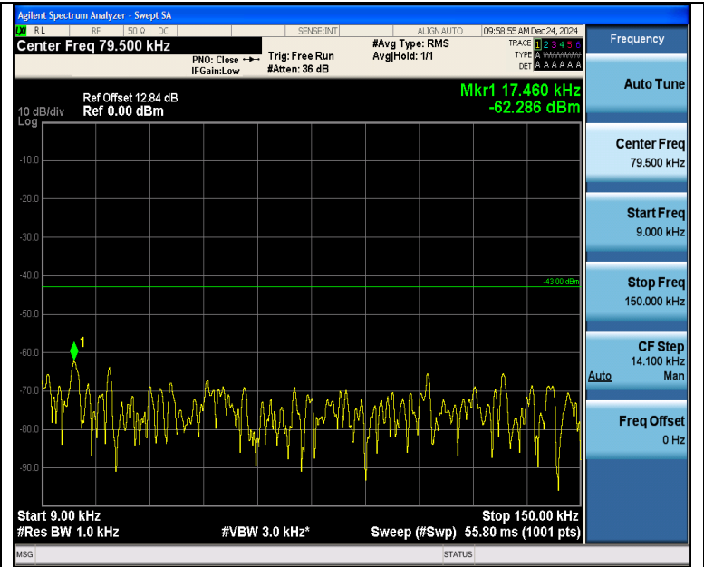
Band2_5MHz_16QAM_18625_1RB#0_0.009~0.15_0.009~0.15
