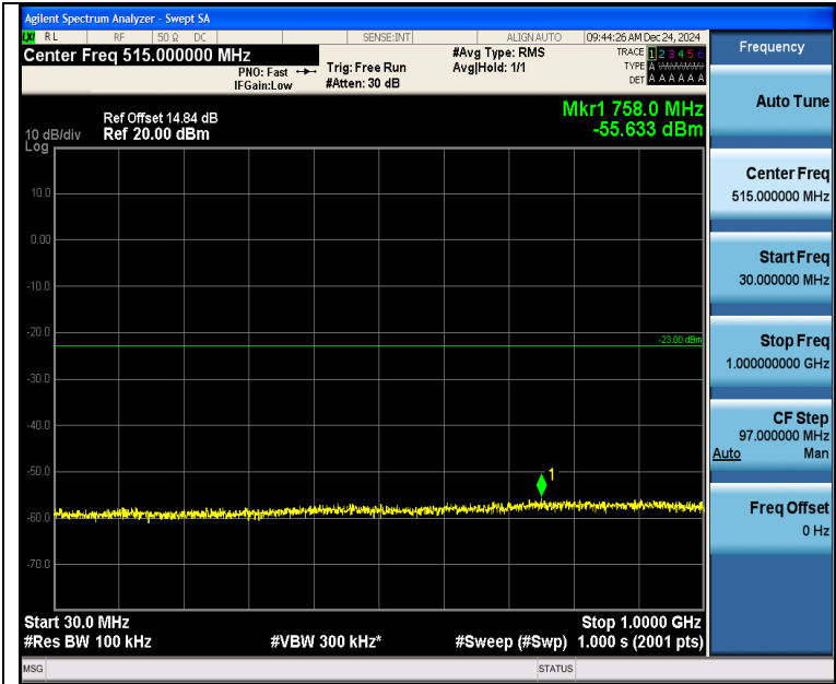
Band2_3MHz_QPSK_18900_1RB#14_30~1000_30~1000
