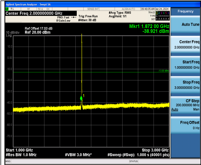
Band2_3MHz_16QAM_18900_15RB#0_1000~3000_1000~3000
