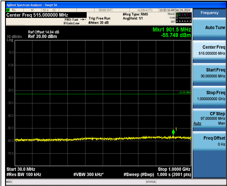
Band2_5MHz_QPSK_18625_1RB#24_30~1000_30~1000
