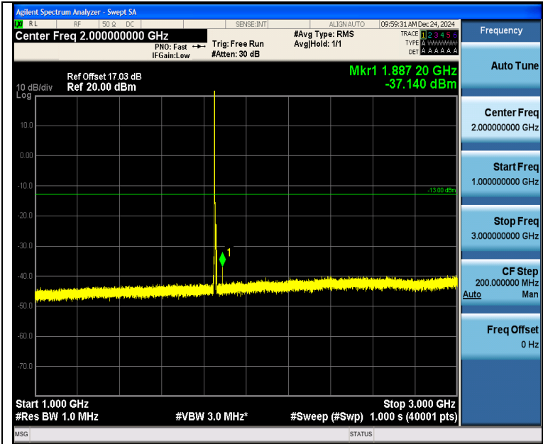
Band2_5MHz_16QAM_18625_1RB#0_1000~3000_1000~3000
