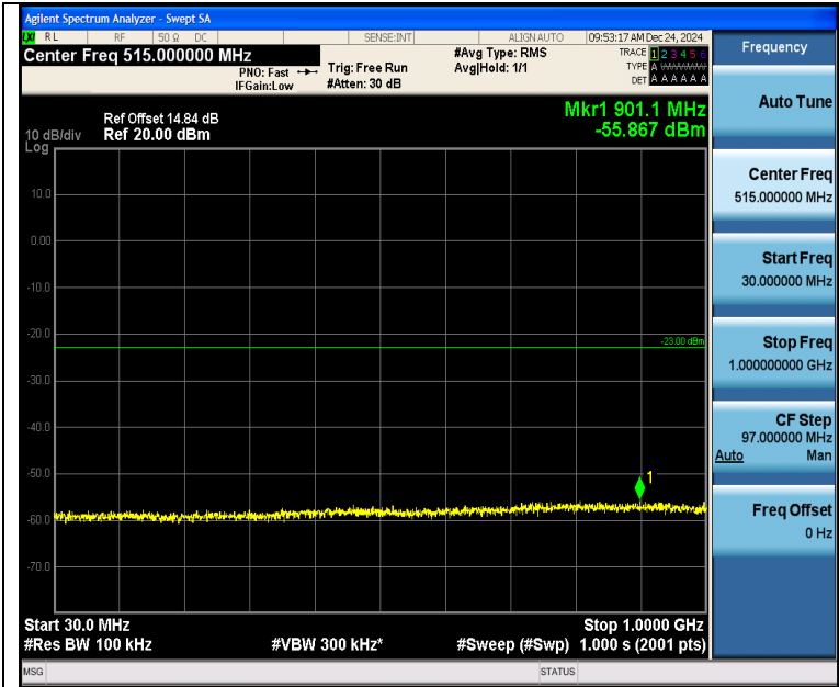
Band2_3MHz_QPSK_19185_15RB#0_30~1000_30~1000
