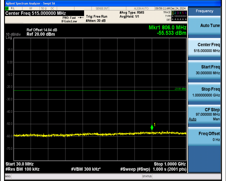
Band2_5MHz_16QAM_18625_1RB#0_30~1000_30~1000
