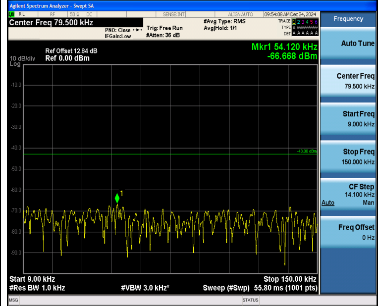
Band2_3MHz_16QAM_19185_15RB#0_0.009~0.15_0.009~0.15
