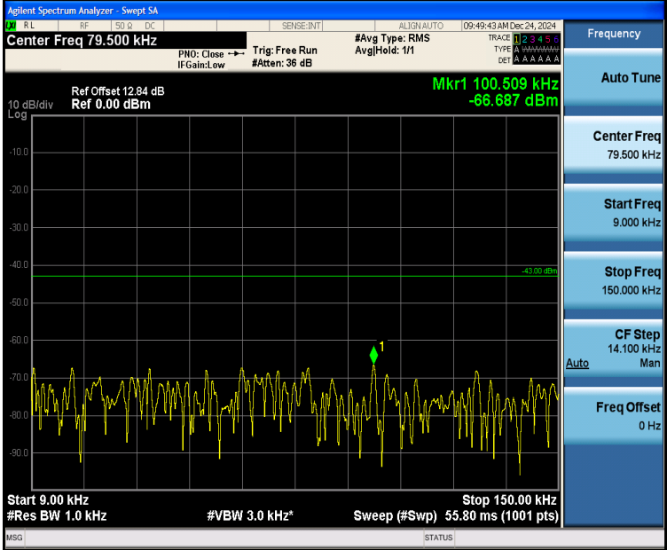
Band2_3MHz_16QAM_19185_1RB#0_0.009~0.15_0.009~0.15
