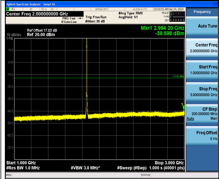
Band2_5MHz_16QAM_18625_25RB#0_1000~3000_1000~3000
