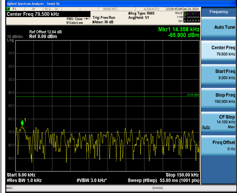
Band2_5MHz_QPSK_18900_25RB#0_0.009~0.15_0.009~0.15
