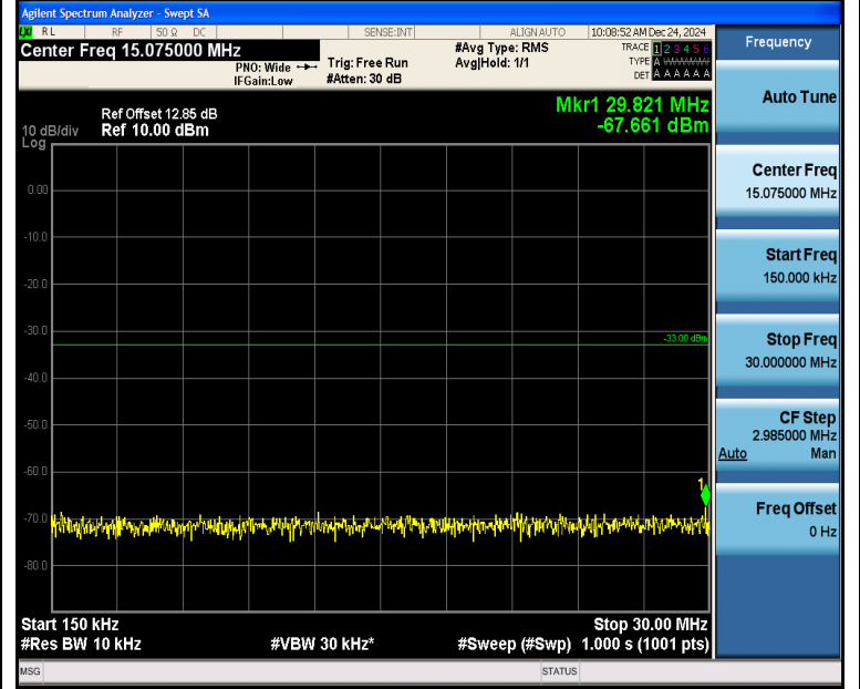
Band2_5MHz_QPSK_18900_25RB#0_0.15~30_0.15~30
