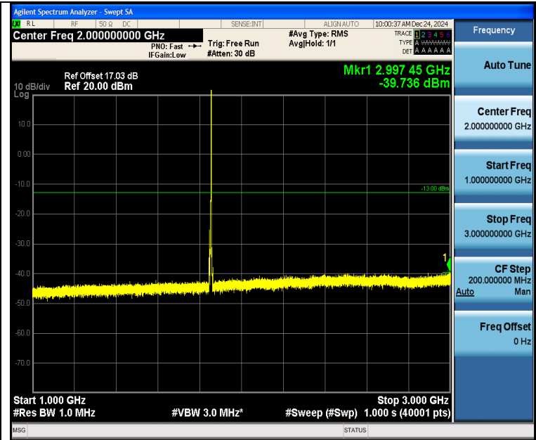
Band2_5MHz_QPSK_18625_1RB#24_1000~3000_1000~3000
