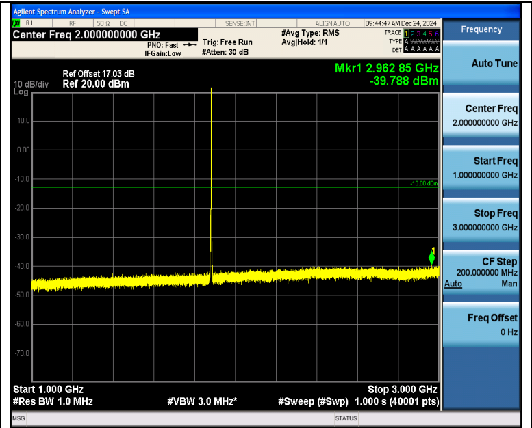
Band2_3MHz_QPSK_18900_1RB#14_1000~3000_1000~3000
