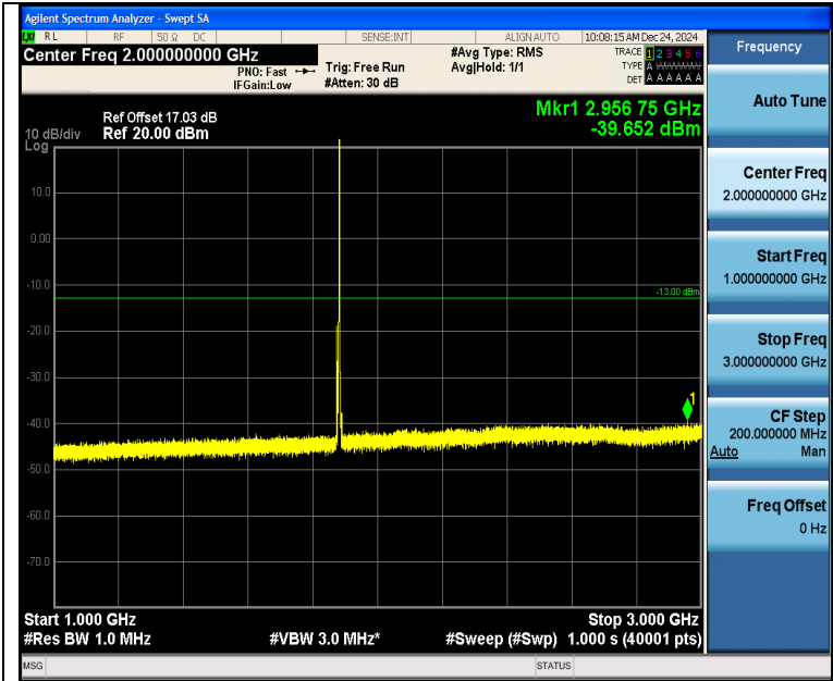
Band2_5MHz_16QAM_18900_1RB#24_1000~3000_1000~3000
