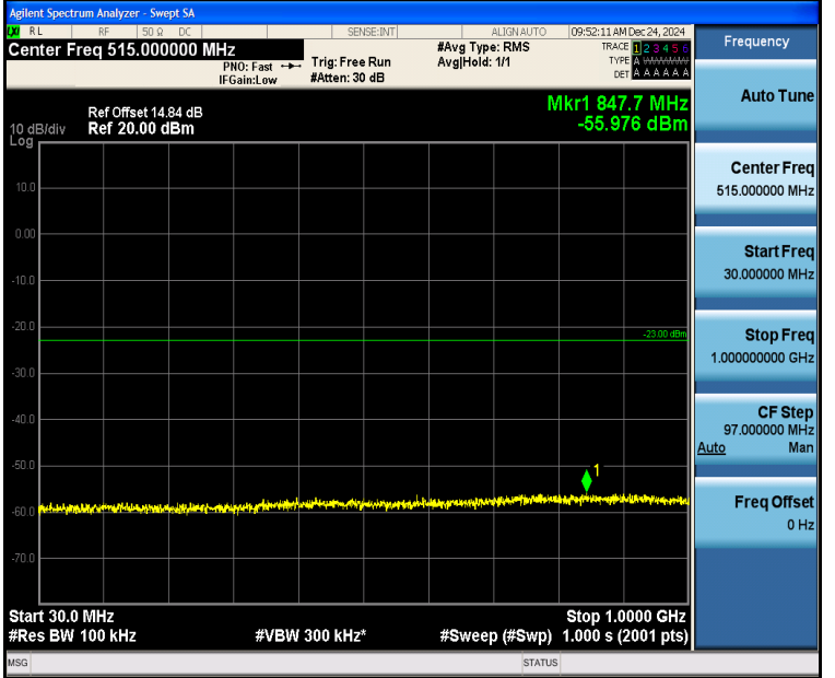
Band2_3MHz_16QAM_19185_1RB#14_30~1000_30~1000
