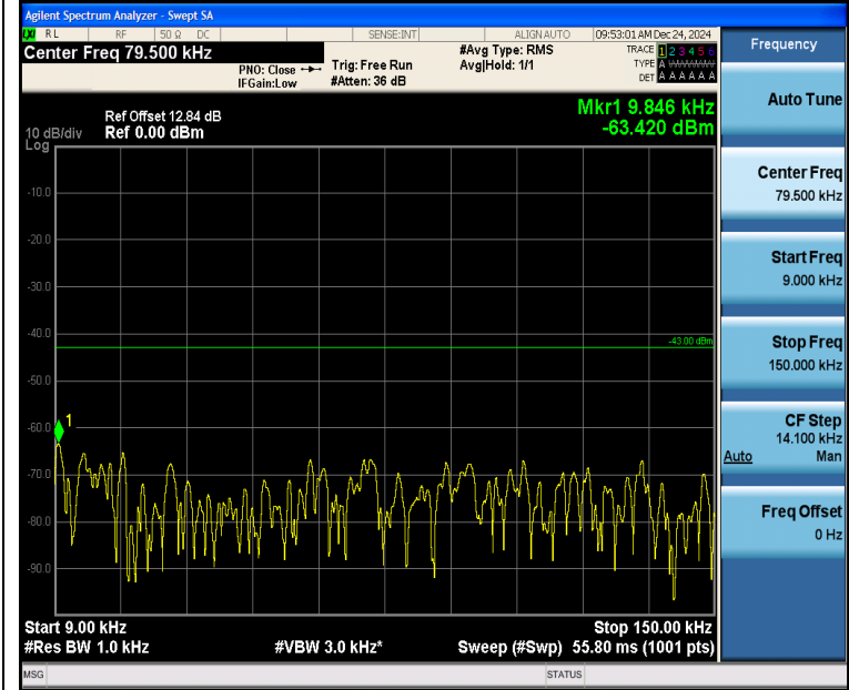
Band2_3MHz_QPSK_19185_15RB#0_0.009~0.15_0.009~0.15
