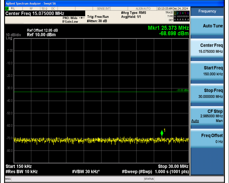
Band2_5MHz_QPSK_19175_1RB#24_0.15~30_0.15~30
