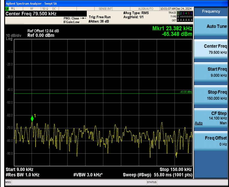
Band2_5MHz_16QAM_18625_1RB#24_0.009~0.15_0.009~0.15
