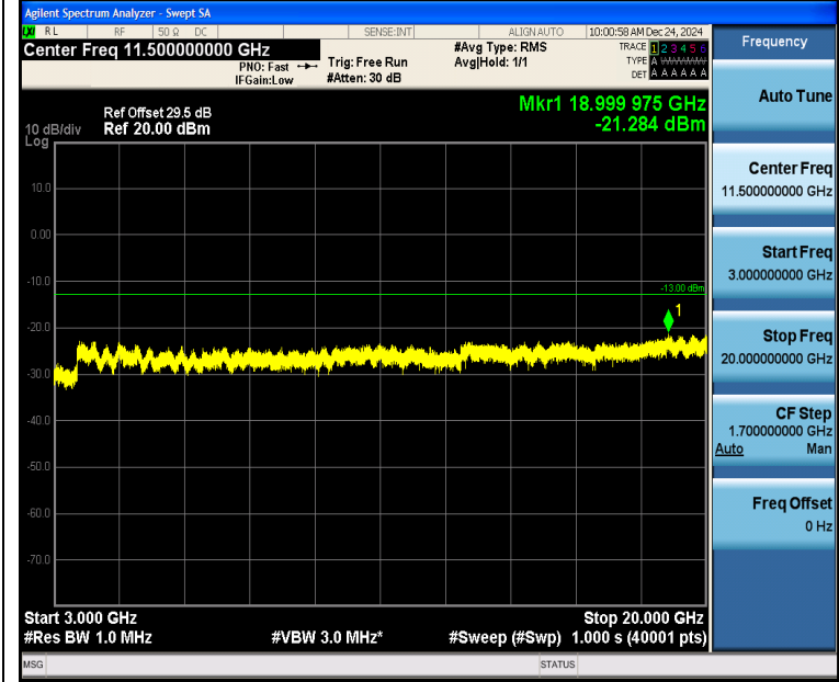
Band2_5MHz_QPSK_18625_1RB#24_3000~20000_3000~20000
