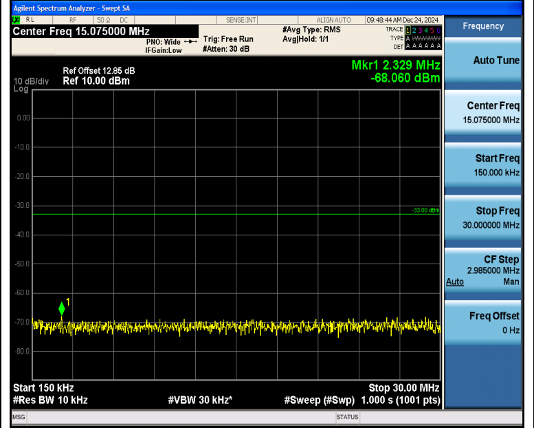
Band2_3MHz_QPSK_19185_1RB#0_0.15~30_0.15~30
