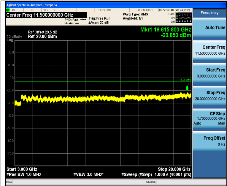
Band2_5MHz_QPSK_18625_1RB#0_3000~20000_3000~20000
