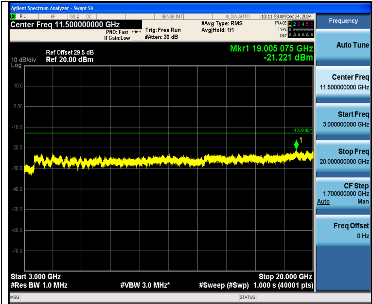
Band2_5MHz_QPSK_19175_1RB#0_3000~20000_3000~20000
