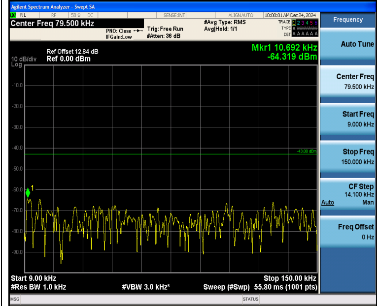
Band2_5MHz_QPSK_18625_1RB#24_0.009~0.15_0.009~0.15
