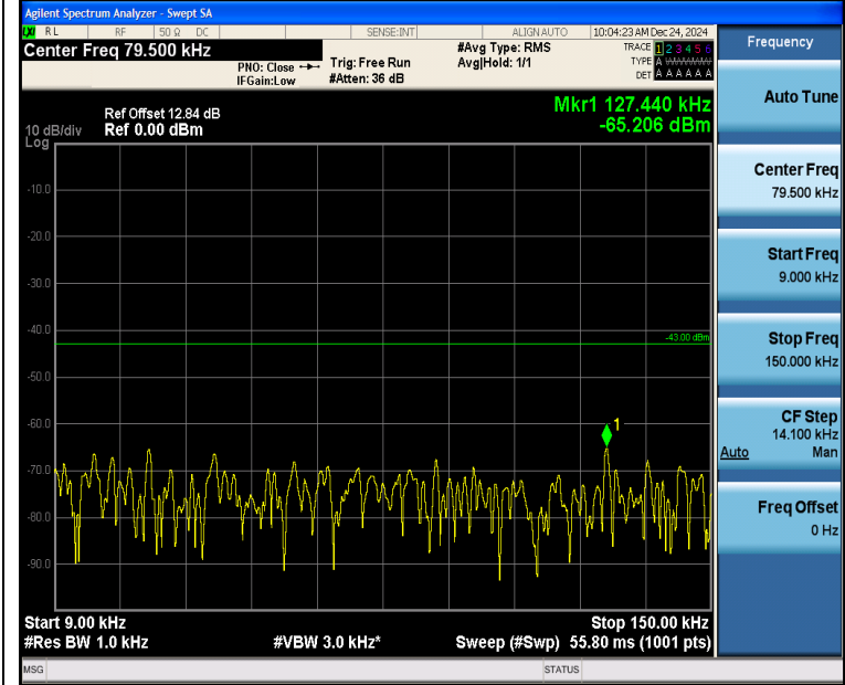
Band2_5MHz_QPSK_18900_1RB#0_0.009~0.15_0.009~0.15
