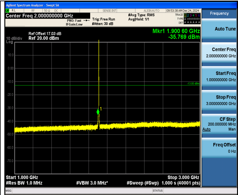
Band2_3MHz_QPSK_19185_15RB#0_1000~3000_1000~3000
