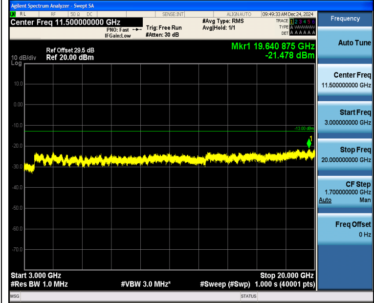
Band2_3MHz_QPSK_19185_1RB#0_3000~20000_3000~20000
