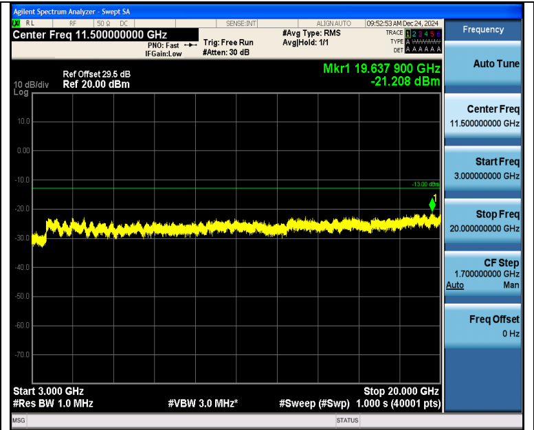
Band2_3MHz_16QAM_19185_1RB#14_3000~20000_3000~20000
