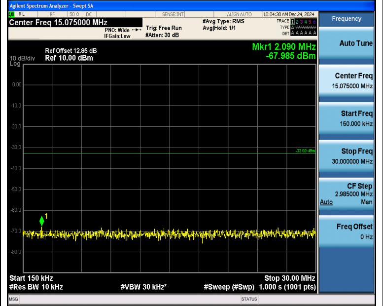
Band2_5MHz_QPSK_18900_1RB#0_0.15~30_0.15~30
