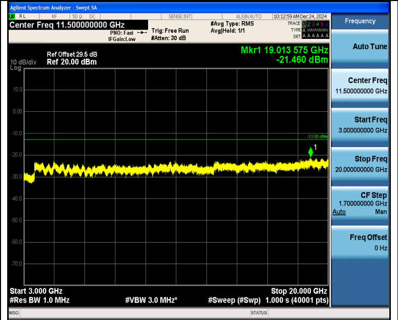
Band2_5MHz_16QAM_19175_1RB#0_3000~20000_3000~20000
