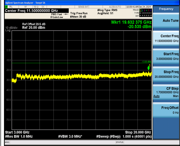
Band2_5MHz_QPSK_18900_25RB#0_3000~20000_3000~20000
