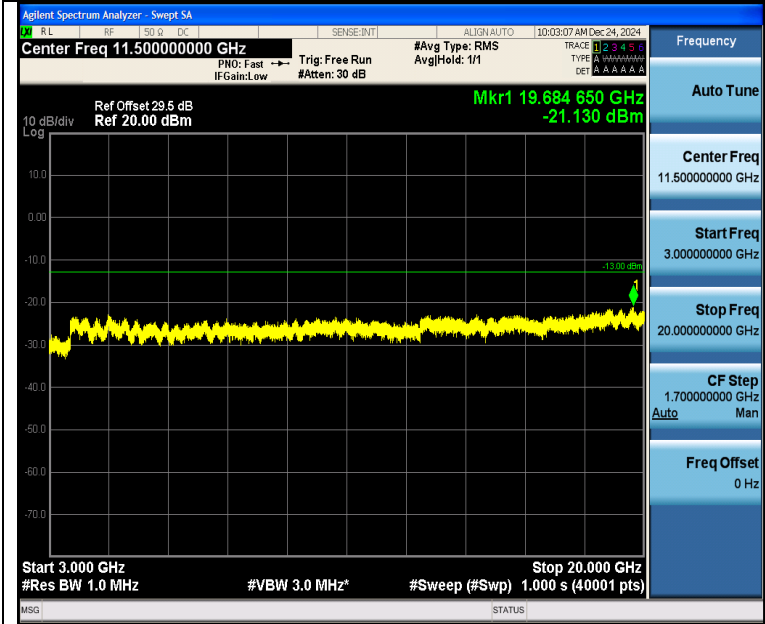
Band2_5MHz_QPSK_18625_25RB#0_3000~20000_3000~20000
