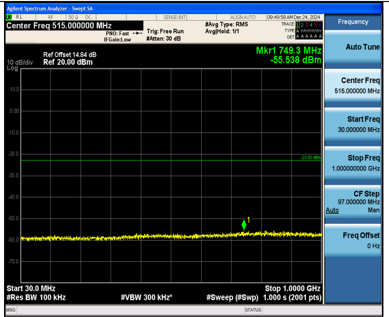
Band2_3MHz_16QAM_19185_1RB#0_30~1000_30~1000
