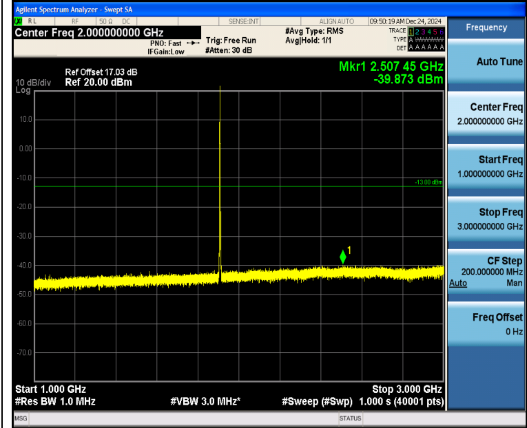
Band2_3MHz_16QAM_19185_1RB#0_1000~3000_1000~3000
