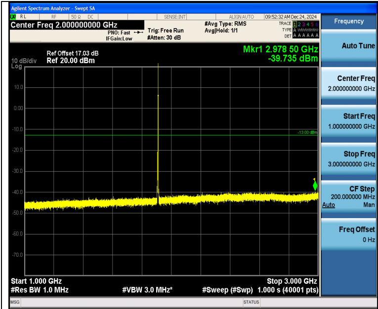
Band2_3MHz_16QAM_19185_1RB#14_1000~3000_1000~3000
