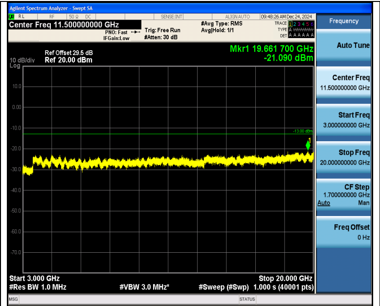
Band2_3MHz_16QAM_18900_15RB#0_3000~20000_3000~20000
