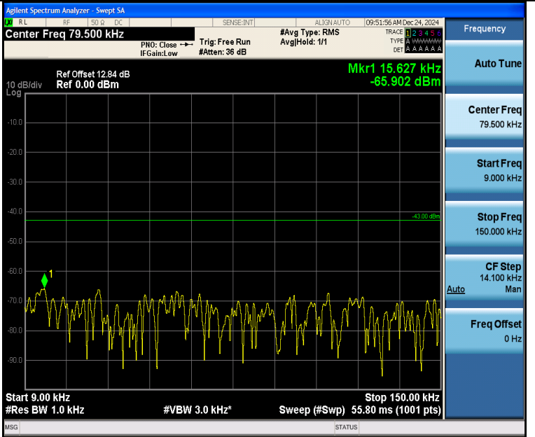
Band2_3MHz_16QAM_19185_1RB#14_0.009~0.15_0.009~0.15
