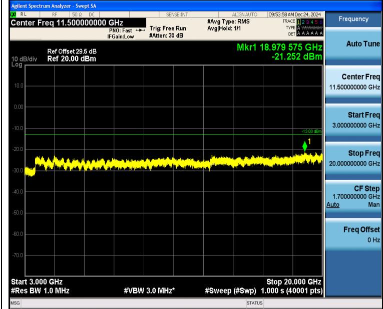
Band2_3MHz_QPSK_19185_15RB#0_3000~20000_3000~20000
