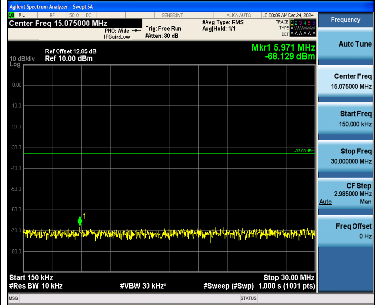
Band2_5MHz_QPSK_18625_1RB#24_0.15~30_0.15~30
