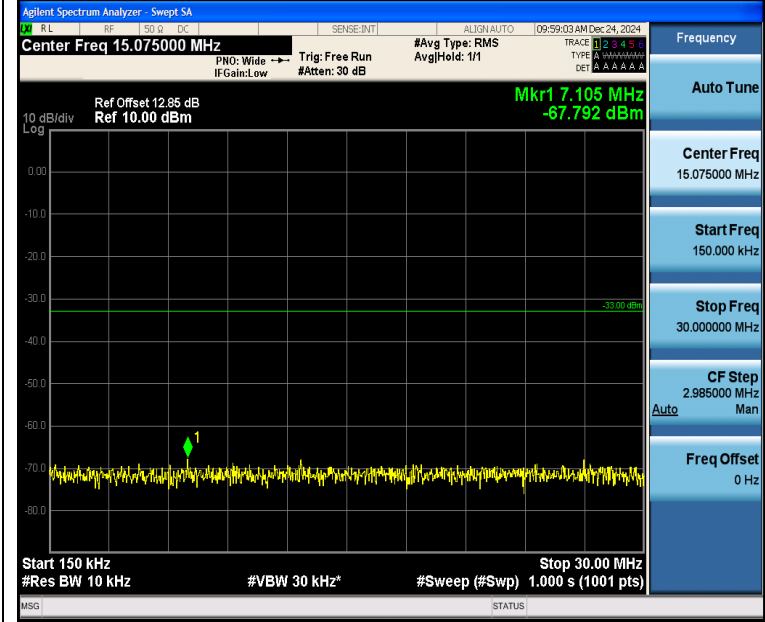
Band2_5MHz_16QAM_18625_1RB#0_0.15~30_0.15~30
