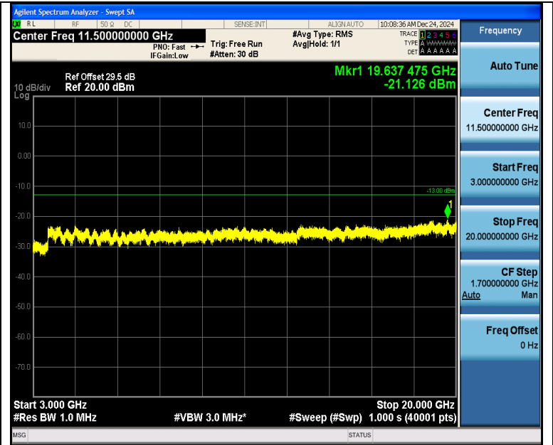
Band2_5MHz_16QAM_18900_1RB#24_3000~20000_3000~20000
