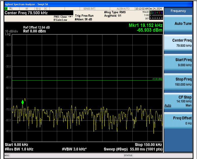
Band2_5MHz_16QAM_19175_1RB#0_0.009~0.15_0.009~0.15
