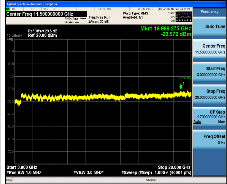
Band2_3MHz_QPSK_18900_1RB#14_3000~20000_3000~20000
