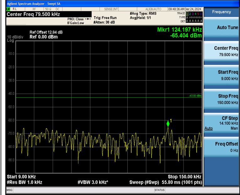
Band2_3MHz_QPSK_19185_1RB#0_0.009~0.15_0.009~0.15
