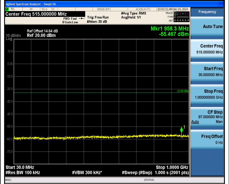
Band2_5MHz_16QAM_18625_25RB#0_30~1000_30~1000
