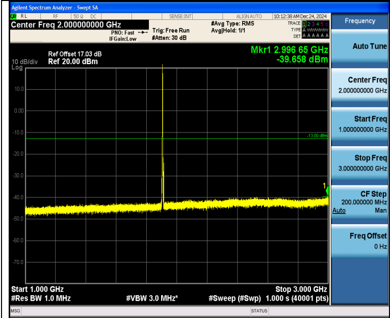
Band2_5MHz_16QAM_19175_1RB#0_1000~3000_1000~3000
