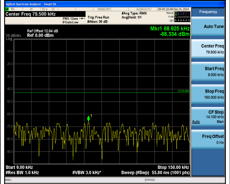
Band2_3MHz_16QAM_18900_1RB#14_0.009~0.15_0.009~0.15
