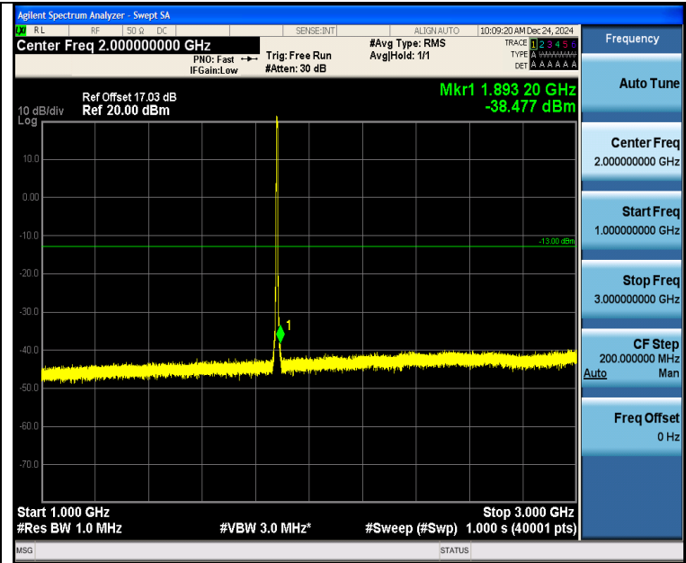
Band2_5MHz_QPSK_18900_25RB#0_1000~3000_1000~3000
