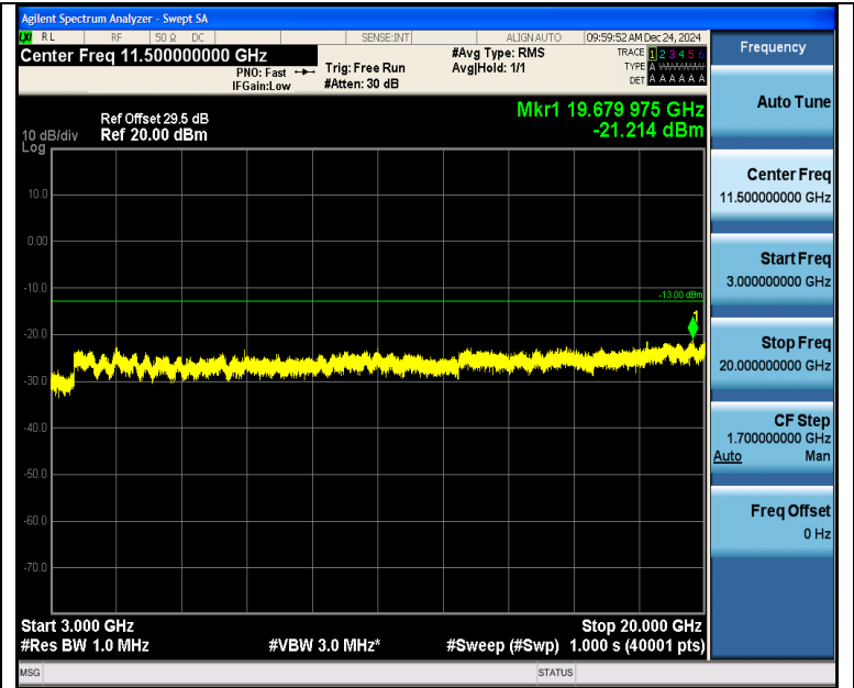
Band2_5MHz_16QAM_18625_1RB#0_3000~20000_3000~20000
