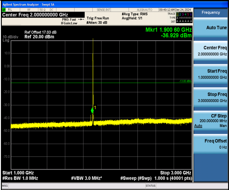
Band2_3MHz_QPSK_19185_1RB#0_1000~3000_1000~3000
