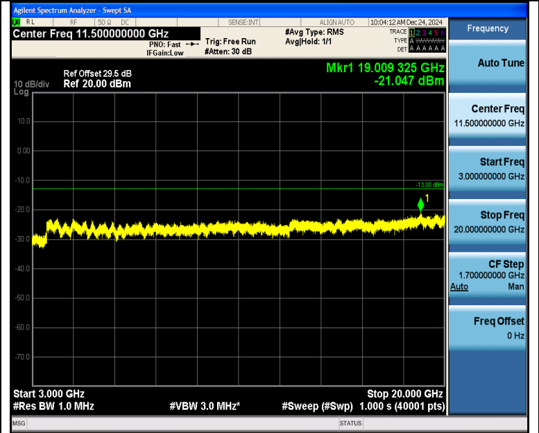
Band2_5MHz_16QAM_18625_25RB#0_3000~20000_3000~20000
