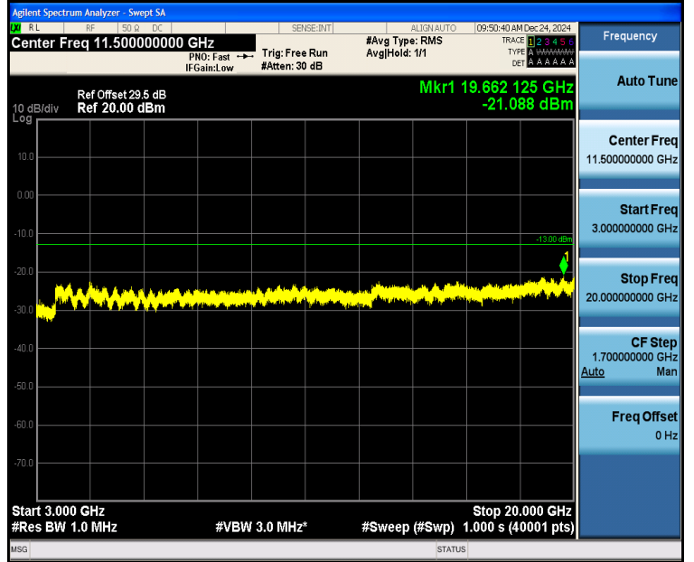
Band2_3MHz_16QAM_19185_1RB#0_3000~20000_3000~20000
