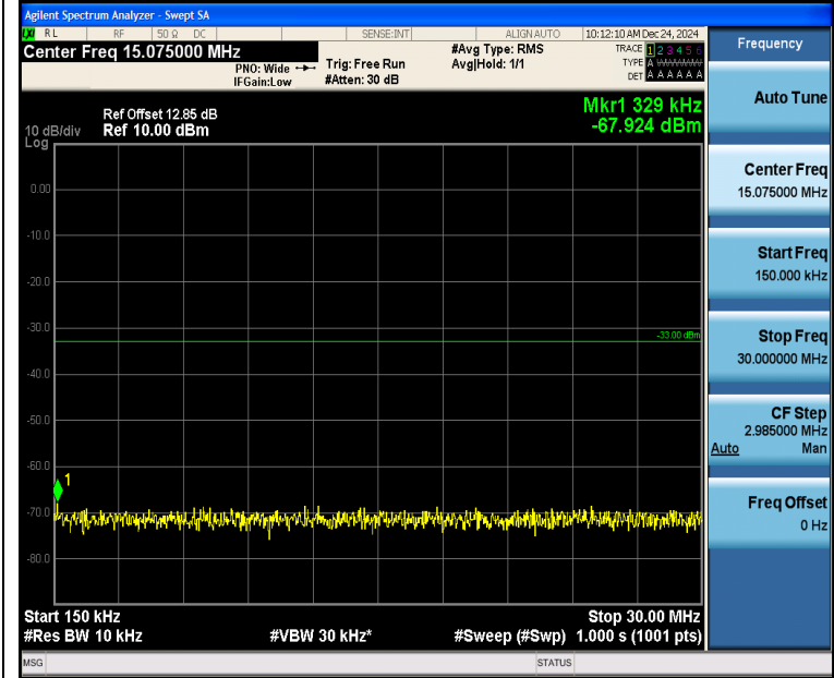
Band2_5MHz_16QAM_19175_1RB#0_0.15~30_0.15~30
