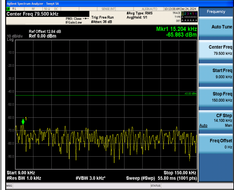
Band2_5MHz_QPSK_19175_1RB#24_0.009~0.15_0.009~0.15
