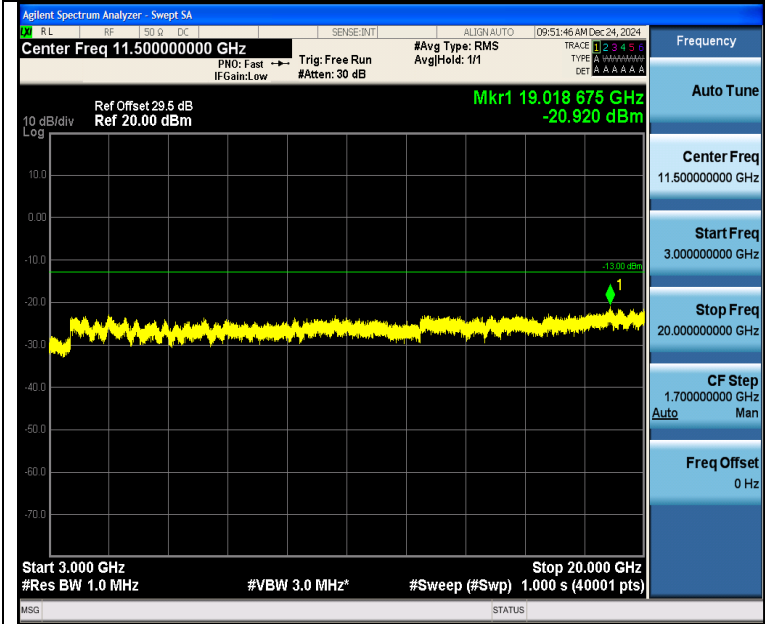
Band2_3MHz_QPSK_19185_1RB#14_3000~20000_3000~20000
