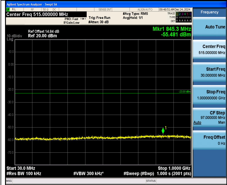
Band2_3MHz_QPSK_19185_1RB#0_30~1000_30~1000
