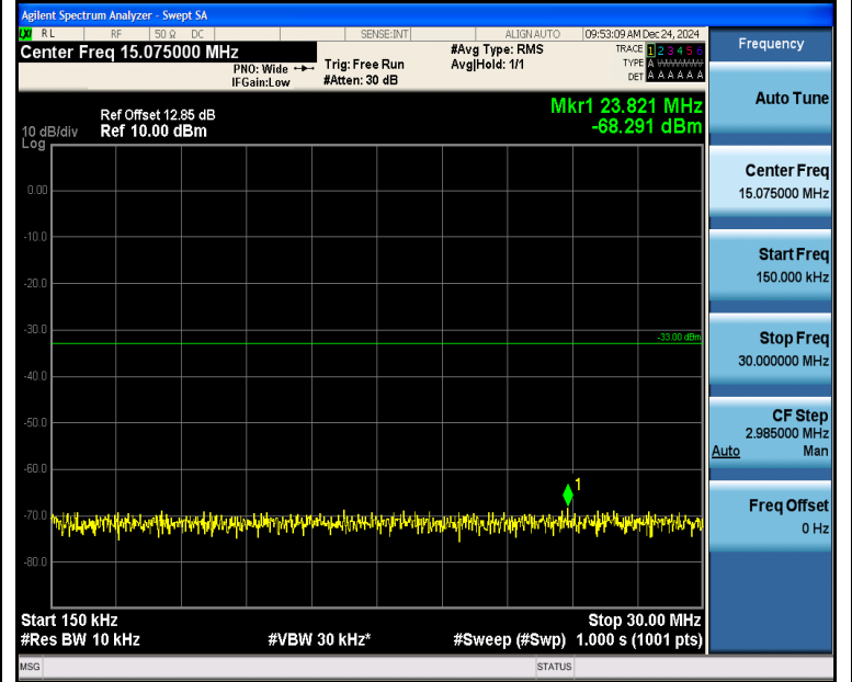
Band2_3MHz_QPSK_19185_15RB#0_0.15~30_0.15~30
