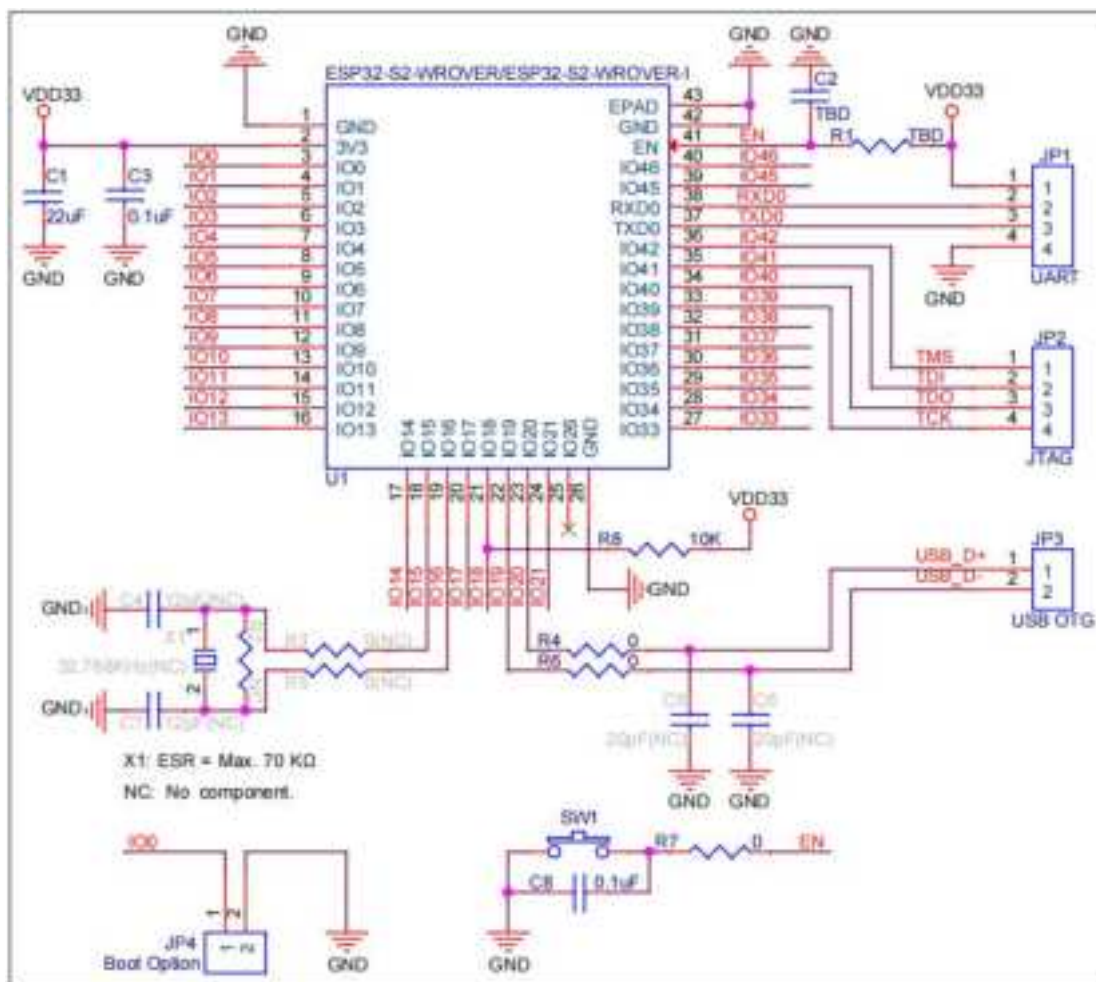
Figure 5 Module Schematics
