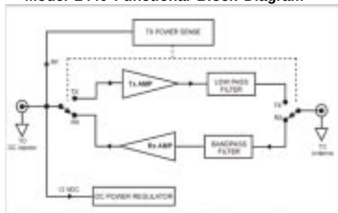
Model 2440 Functional Block Diagram
