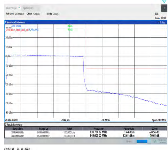
1-N5-PC3-15-10-H-6-CP-QPSK-Outer_Full-52@0-Ant1-1-seegraph-PASS-see graph
