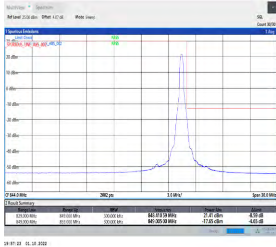
1-N5-PC3-15-20-H-2-DFT-PI2BPSK-Edge_1RB_Right-1@105-Ant1-1-seegraph-PASS-see graph
