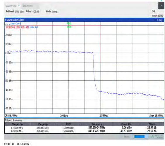
1-N5-PC3-15-15-H-3-DFT-PI2BPSK-Outer_Full-75@0-Ant1-1-seegraph-PASS-see graph
