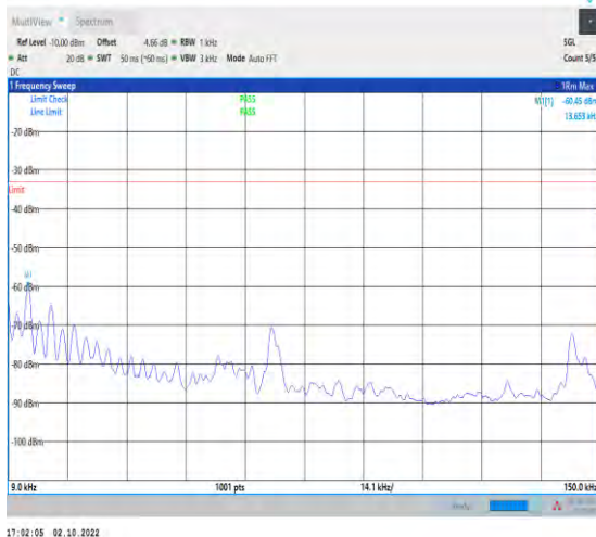
1-N5-PC3-15-20-H-1-DFT-PI2BPSK-Inner_1RB_Left -1@1-0.009-0.15-Ant1-0.01--60.45--33-PASS
