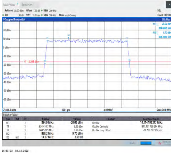
1-N5-PC3-15-15-H-9-CP-256QAM-Out_ Full-79@0-Ant1-14.114-14.970-≤15-PASS
