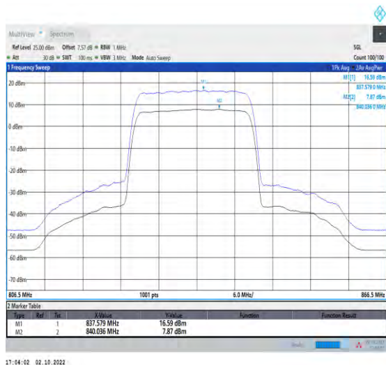
1-N5-PC3-15-20-M-1-DFT-256QAM-Outet_Full-100 @0-Ant1-8.72-100%-0.00-8.72-PASS-≤13
