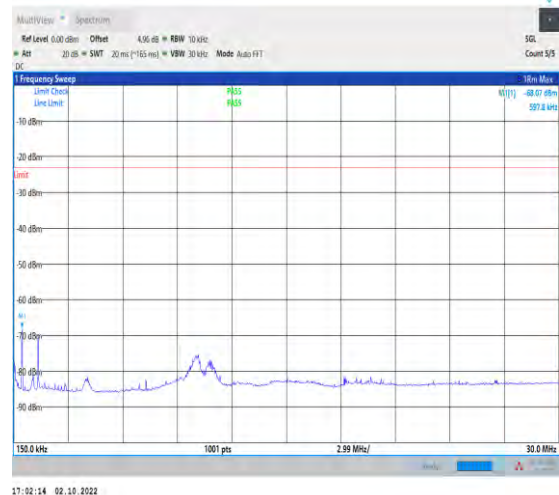
1-N5-PC3-15-20-H-1-DFT-PI2BPSK-Inner_1RB_Left -1@1-0.15-30-Ant1-0.60--68.07--23-PASS
