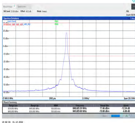
1-N5-PC3-15-10-H-5-CP-QPSK-Edge_1RB_Right-1@51-Ant1-1-seegraph-PASS-see graph
