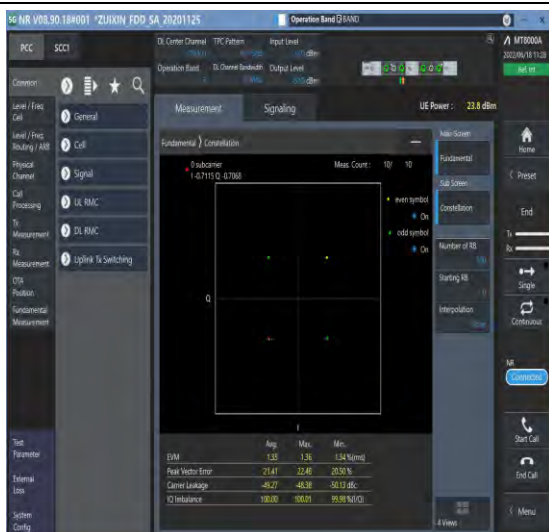
1-N5--15-20-M-1-DFT-PI2BPSK-Outer_Full-100@0-A nt1-see graph-PASS
