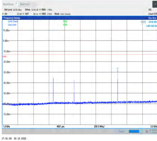
1-N5-PC3-15-20-M-1-DFT-PI2BPSK-Inner_1RB_Left -1@1-1000-3000-Ant1-2481.50--29.83--13-PASS
