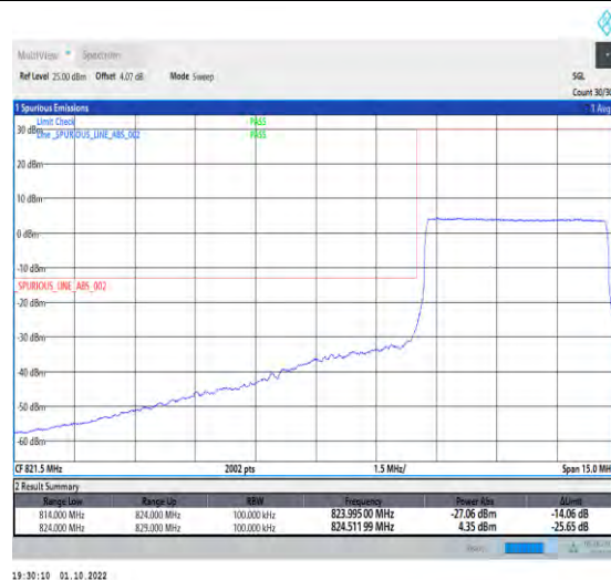
1-N5-PC3-15-5-L-6-CP-QPSK-Outer_Full-25@0-A nt1-1-seegraph-PASS-see graph
