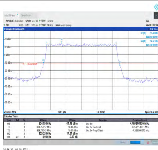
1-N5-PC3-15-5-L-2-DFT-PI2BPSK-Outet_Full-25@0 -Ant1-4.47-4.900-≤5-PASS
