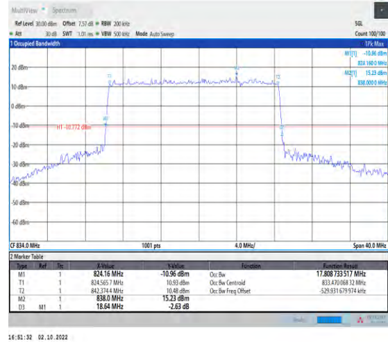
1-N5-PC3-15-20-L-1-DFT-QPSK-Out_ Full-100@0-Ant1-17.809-18.640-≤20-PASS
