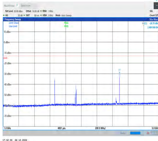
1-N5-PC3-15-20-H-1-DFT-PI2BPSK-Inner_1RB_Left -1@1-1000-3000-Ant1-2489.50--29.70--13-PASS
