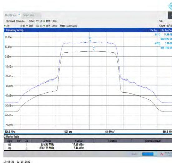
1-N5-PC3-15-20-M-2-CP-256QAM-Outet_Full-106 @0-Ant1-9.45-100%-0.00-9.45-PASS-≤13
