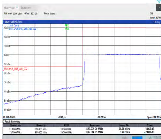
1-N5-PC3-15-10-L-6-CP-QPSK-Outer_Full-52@0- Ant1-1-seegraph-PASS-see graph
