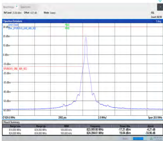
1-N5-PC3-15-10-L-1-DFT-PI2BPSK-Edge_1RB_Left-1 @0-Ant1-1-seegraph-PASS-see graph
