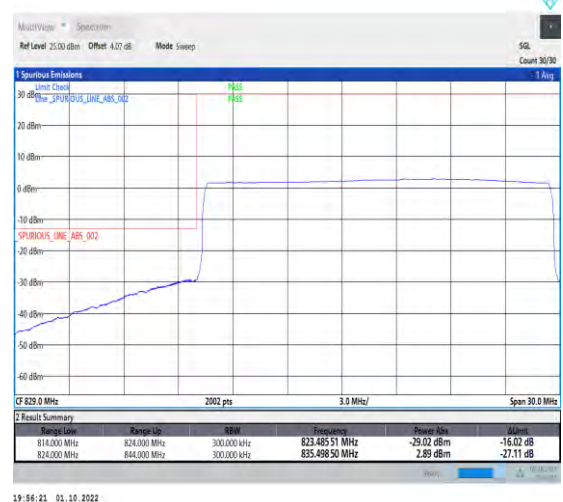
1-N5-PC3-15-20-L-6-CP-QPSK-Outer_Full-106@0- Ant1-1-seegraph-PASS-see graph
