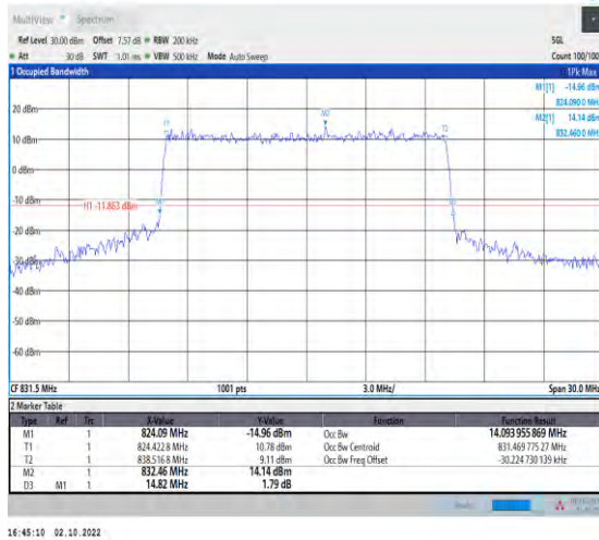
1-N5-PC3-15-15-L-7-CP-16QAM-Outer_Full-79@0-Ant1-14.094-14.820-≤15-PASS
