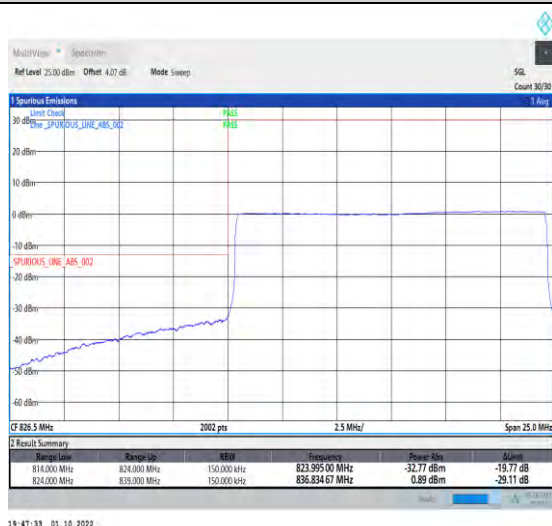
1-N5-PC3-15-15-L-6-CP-QPSK-Outer_Full-79@0- Ant1-1-seegraph-PASS-see graph
