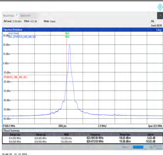
1-N5-PC3-15-15-L-4-CP-QPSK-Edge_1RB_Left-1@0- Ant1-1-seegraph-PASS-see graph
