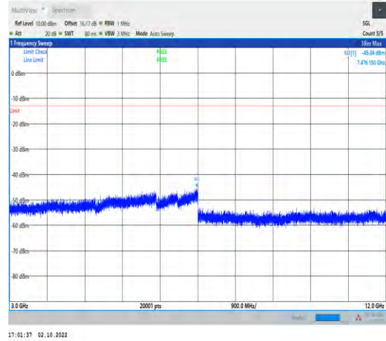
1-N5-PC3-15-20-M-1-DFT-PI2BPSK-Inner_1RB_Left -1@1-3000-12000-Ant1-7476.15--45.04--13-PASS
