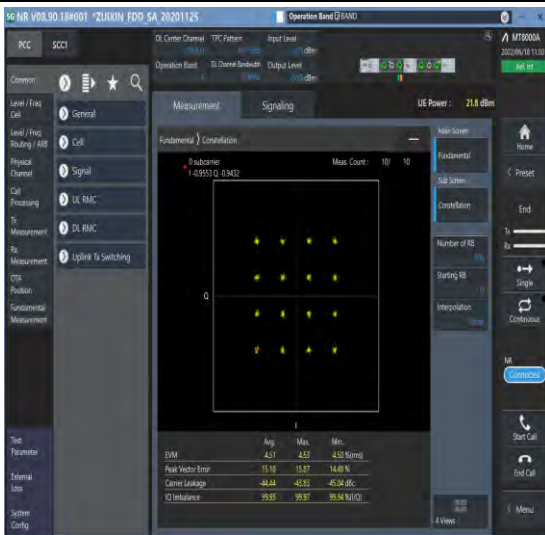
1-N5--15-20-M-7-CP-16QAM-Outer_Full-106@0-Ant1 -see graph-PASS
