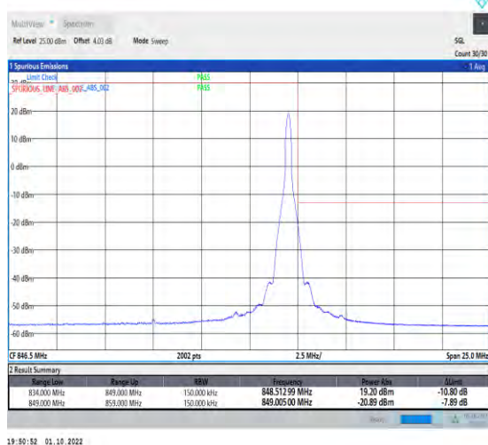
1-N5-PC3-15-15-H-5-CP-QPSK-Edge_1RB_Right-1@78-Ant1-1-seegraph-PASS-see graph
