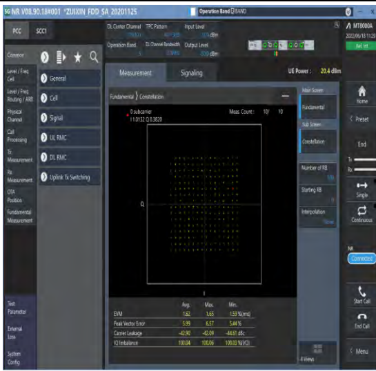
1-N5--15-20-M-5-DFT-256QAM-Outer_Full-100@0-A nt1-see graph-PASS
