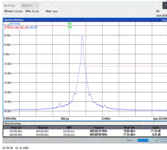
1-N5-PC3-15-10-H-2-DFT-PI2BPSK-Edge_1RB_Right-1@51-Ant1-1-seegraph-PASS-see graph
