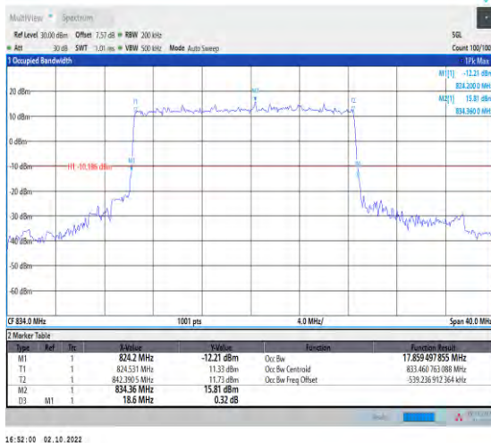
1-N5-PC3-15-20-L-2-DFT-PI2BPSK-Out_ Full-100@0-Ant1-17.859-18.600-≤20-PASS
