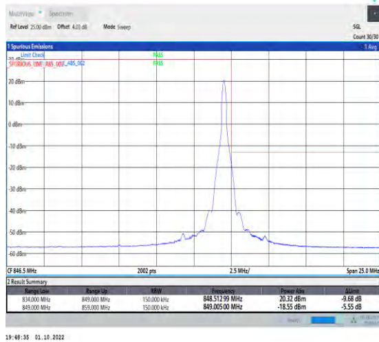
1-N5-PC3-15-15-H-2-DFT-PI2BPSK-Edge_1RB_Right-1@78-Ant1-1-seegraph-PASS-see graph
