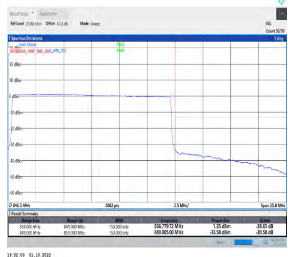
1-N5-PC3-15-15-H-6-CP-QPSK-Outer_Full-79@0-Ant1-1-seegraph-PASS-see graph
