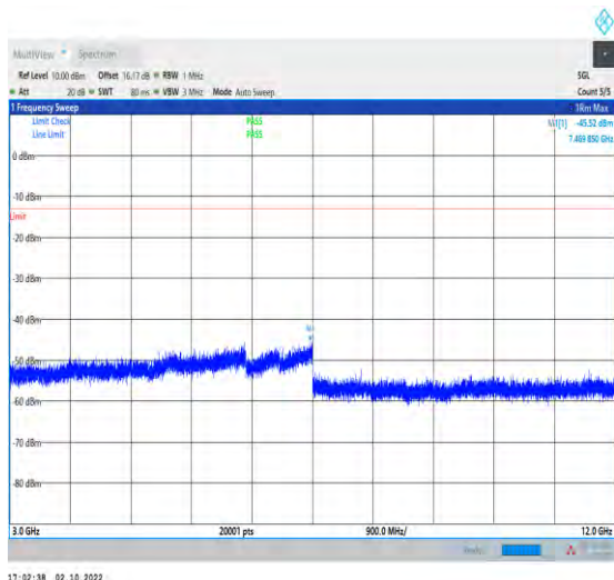
1-N5-PC3-15-20-H-1-DFT-PI2BPSK-Inner_1RB_Left -1@1-3000-12000-Ant1-7469.85--45.52--13-PASS
