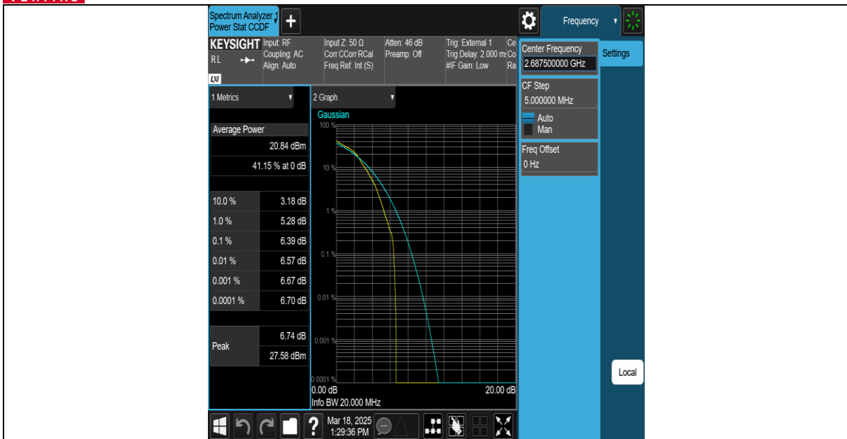
Band41-5MHz-16QAM-41565-25RB#0-PASS
