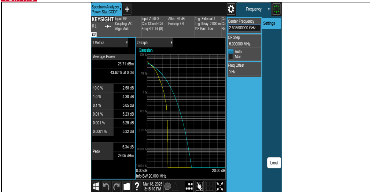
Band41-15MHz-QPSK-39725-75RB#0-PASS
