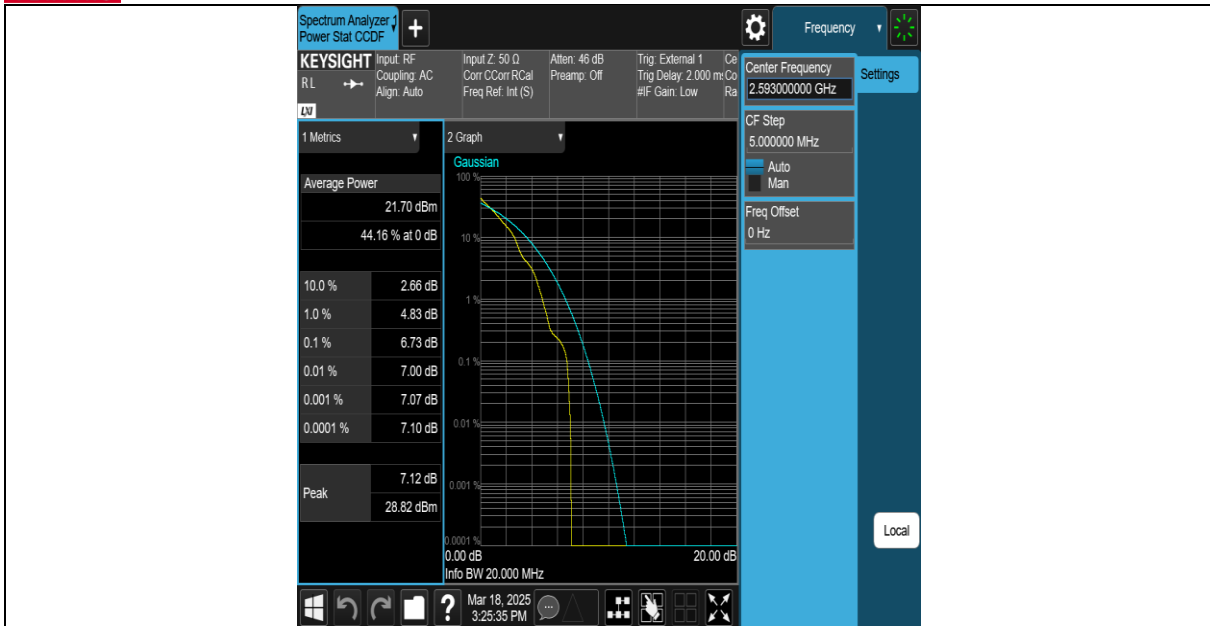
Band41-20MHz-QPSK-40620-100RB#0-PASS
