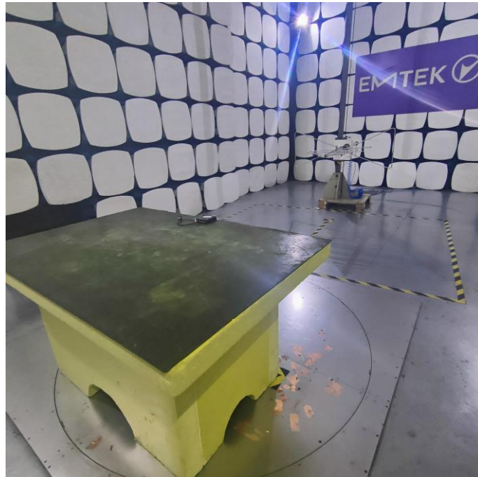
Spurious Emission Test Setup (Below 1GHz)
