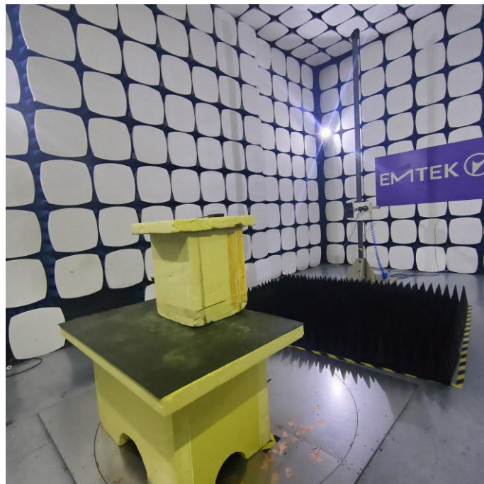
Spurious Emission Test Setup (Above 1GHz)
