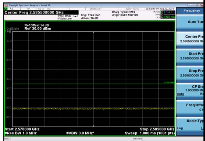
FDD07_5MHz_2502.5_Q16_fullRB_ExtraBan ds_Range_2576~2595
