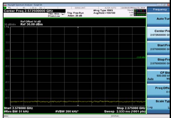
FDD07_10MHz_2505_Q16_fullRB_ExtraBand s_Range_2570~2575
