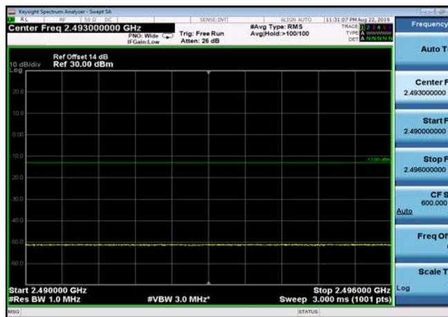
FDD07_15MHz_2562.5_QPSK_OneRB_low _ExtraBands_Range_2490~2496
