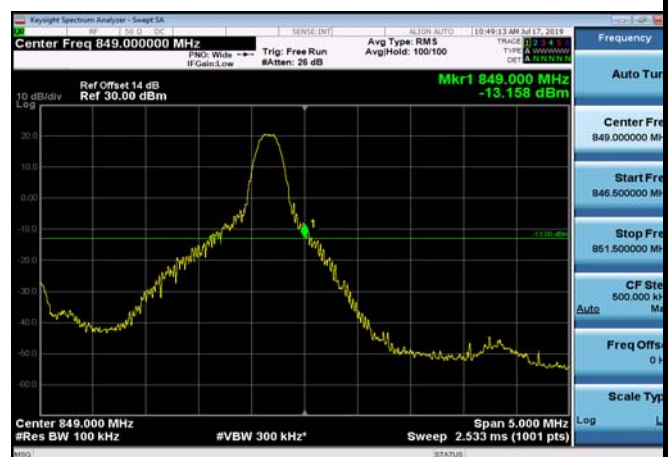
HighRange_FDD05_5MHz_846.5_fullIRB _High_Q16
