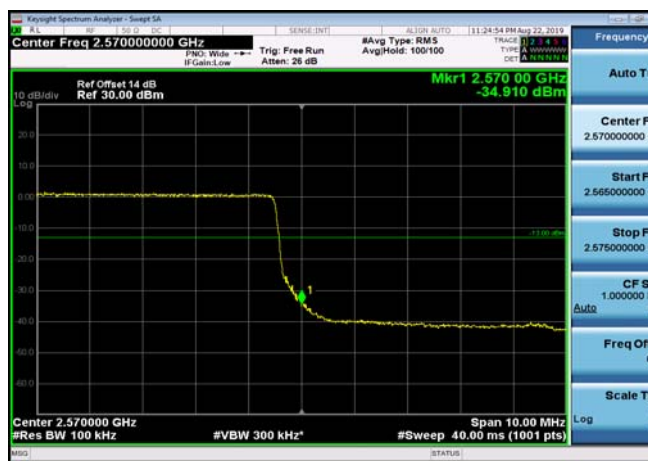
HighRange_FDD07_10MHz_2565_fullRB _High_Q16
