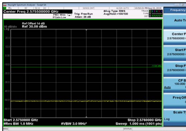
FDD07_5MHz_2502.5_Q16_fullRB_ExtraBan ds_Range_2575~2576
