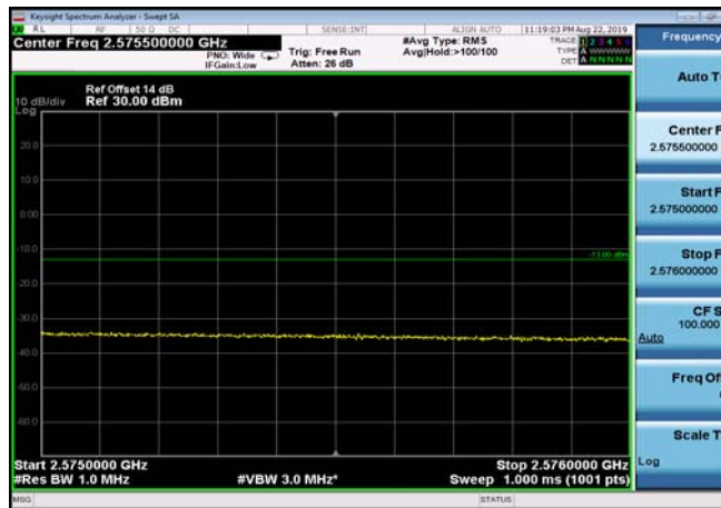
HighRange_FDD07_10MHz_2565_OneRB_high_QPSK
