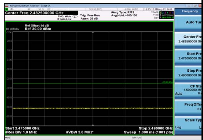
FDD07_10MHz_2565_QPSK_fullRB_ExtraBan ds_Range_2475~2490
