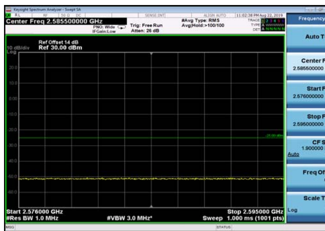
FDD07_15MHz_2507.5_QPSK_OneRB_high ExtraBands_Range_2576~2595
