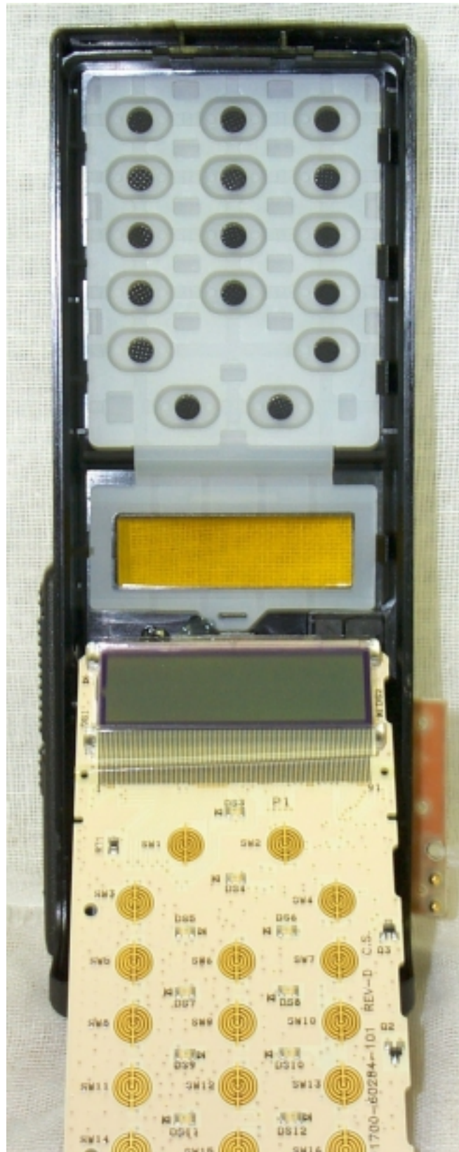
Photo 7. EUT, Keyboard/Display Board
