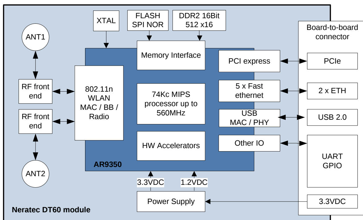
Picture 3: Neratec DT60M Block Diagram
