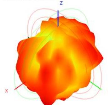
5850.0MHz H+V, Eff: 35.4%
