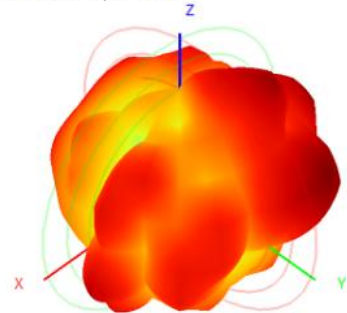
2450.0MHz H+V, Eff: 41.3%
