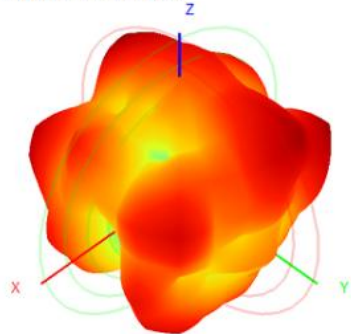
2450.0MHz H+V, Eff: 34.4%
