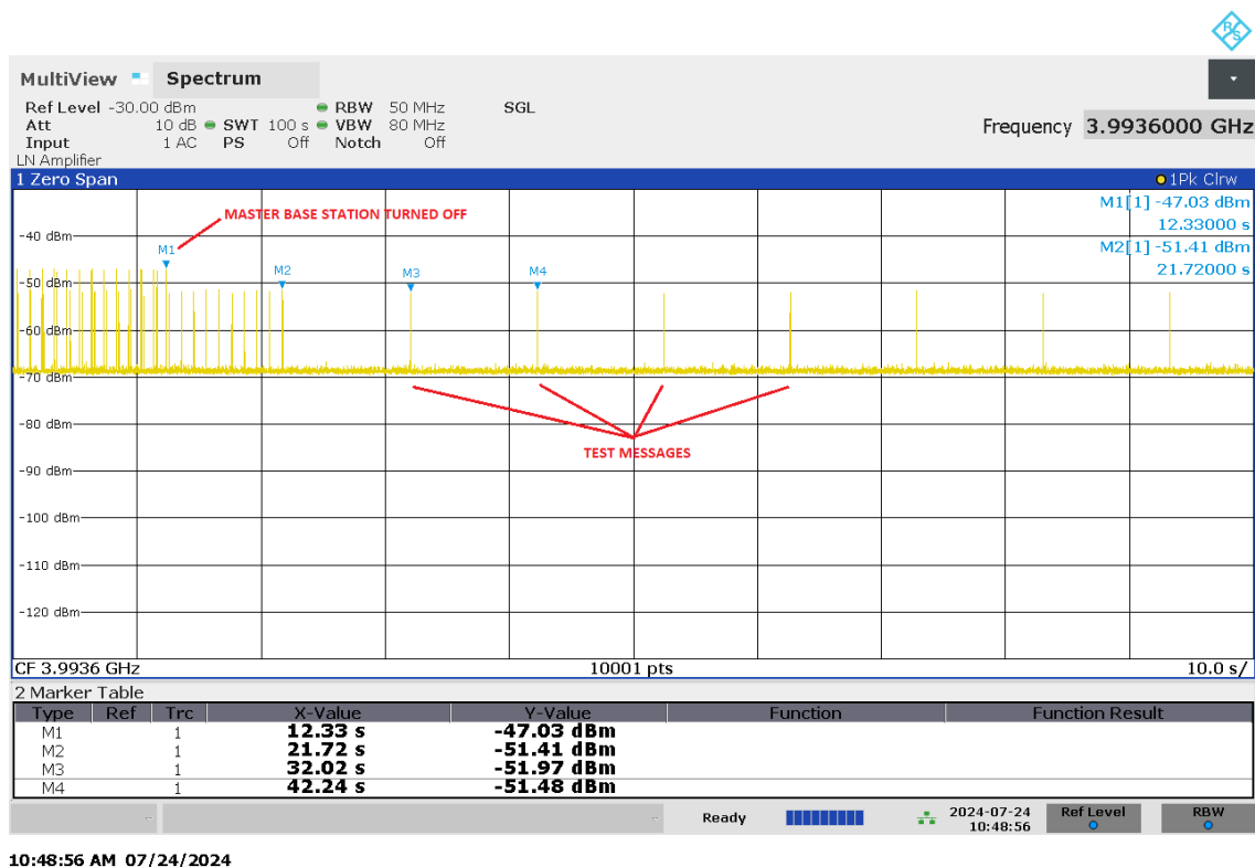
Figure 15: Transmission time
