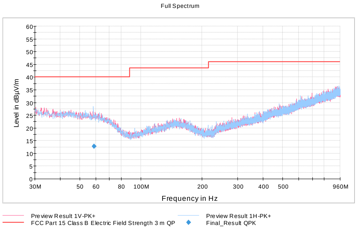
Figure 5: Radiated emissions 30 – 960 MHz
