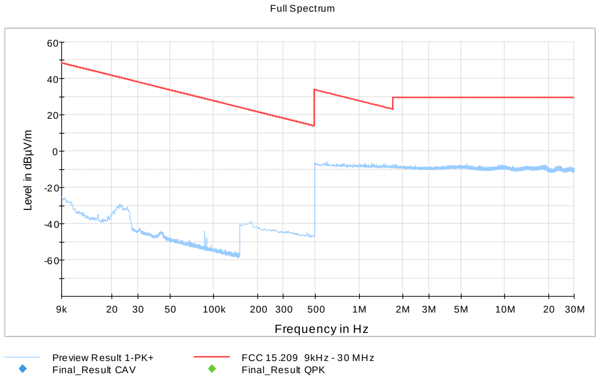
Figure 4: Radiated emissions 9 kHz – 30 MHz
