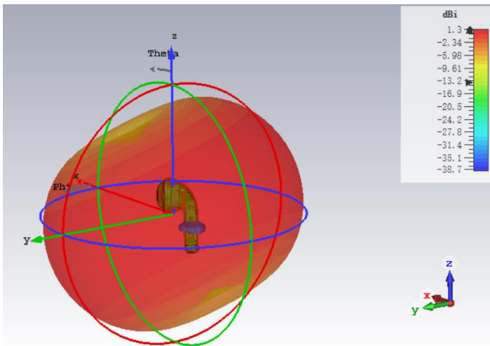
adiation pattern @2.480GHz
