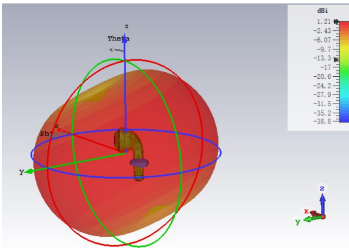
Radiation pattern @2.440GHz
