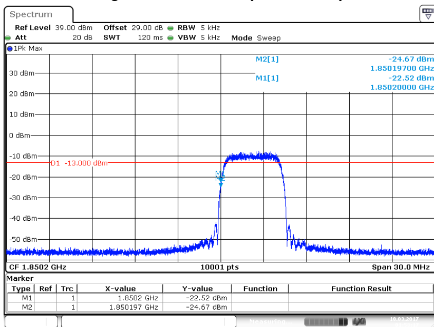
Figure Channel 9262 (1852.40MHz)
