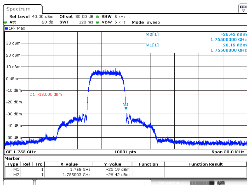
Figure Channel 1513 (1752.60MHz)
