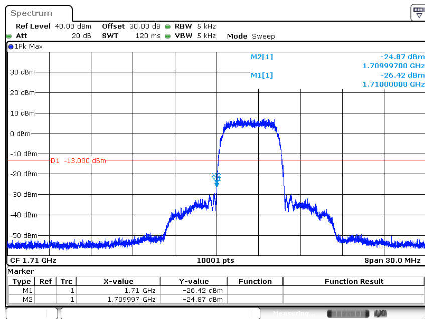
Figure Channel 1312 (1712.40MHz)
