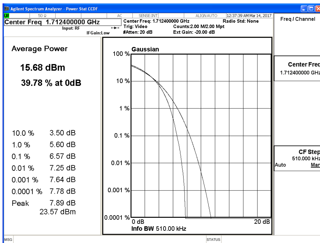
Figure Channel 1312 (1712.4MHz)
