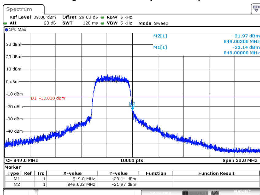
Figure Channel 251 (846.60MHz)
