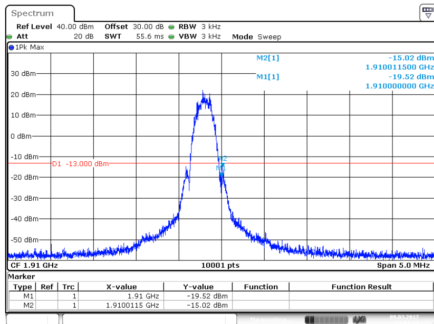
Figure Channel 810 (1909.80MHz)
