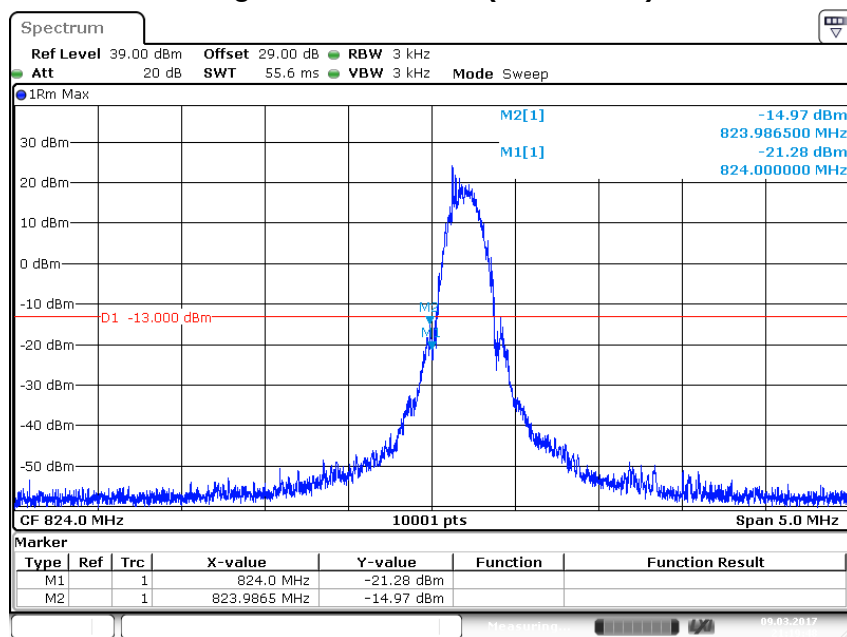
Figure Channel 128 (824.20MHz)
