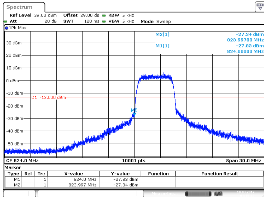
Figure Channel 4132 (826.40MHz)
