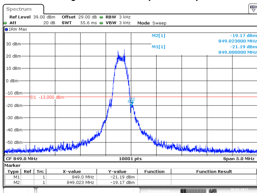
Figure Channel 251 (848.80MHz)
