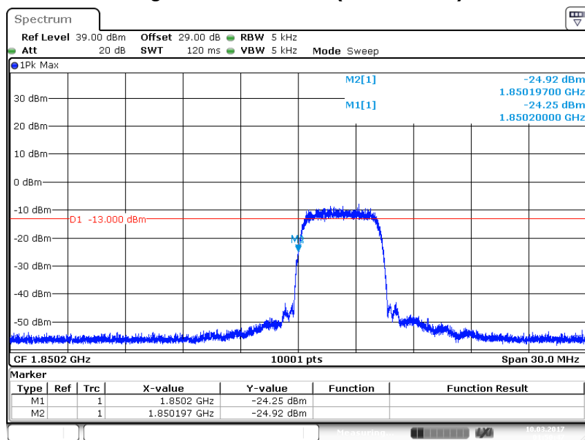
Figure Channel 9262 (1852.40MHz)
