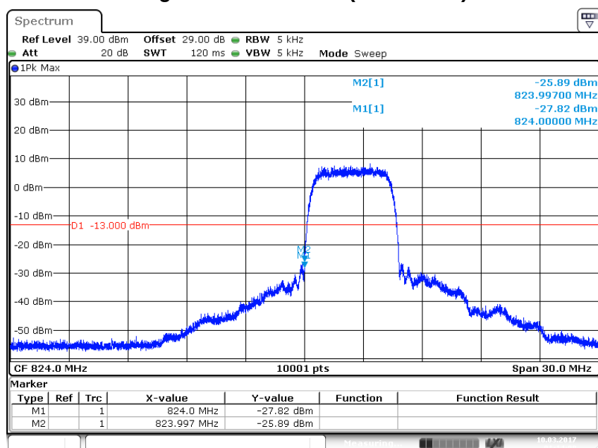
Figure Channel 4132 (826.40MHz)
