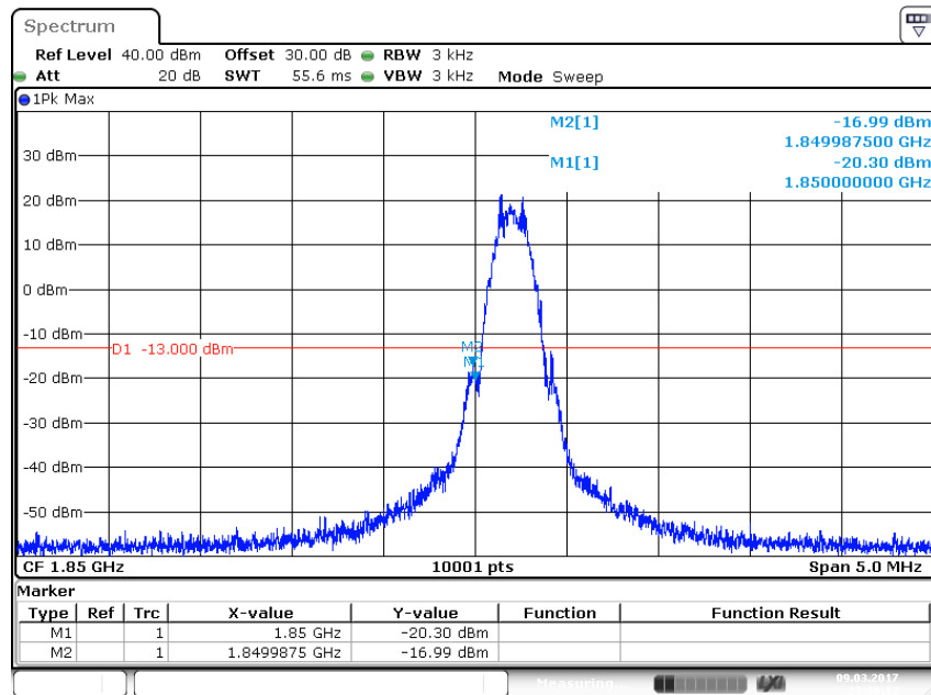
Figure Channel 512 (1850.20MHz)
