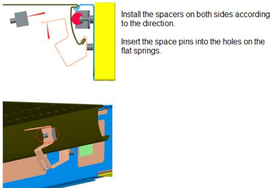
Figure 3-3 HS-AT3511 assembly diagram
