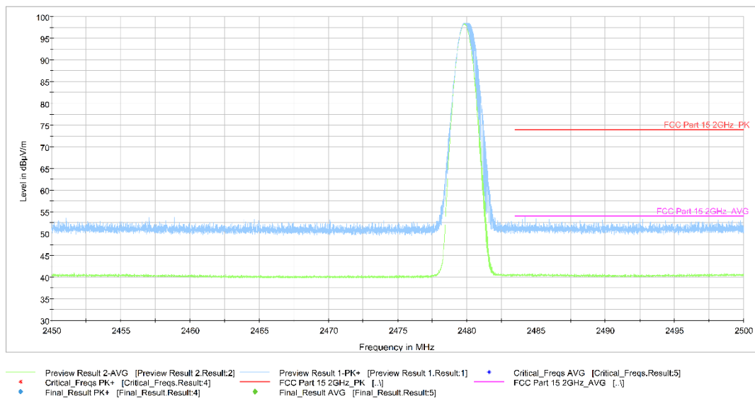
Fig.14. Frequency Band Edges: GFSK, Channel 78, Hopping Off, ch11, 2.45 GHz - 2.50GHz
