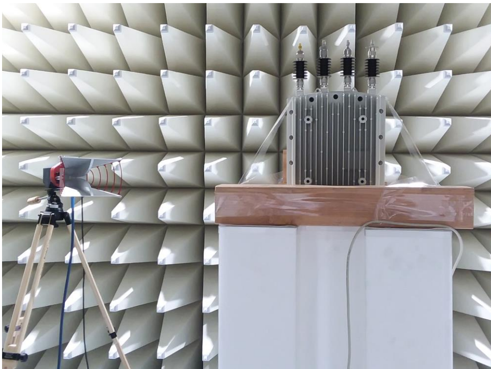
Figure B4: High Range 1-18GHz Radiated Emission test setup Using horn antenna
