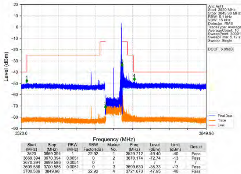
n78d_30kHz_MIMO_NTNV_30MHz_CP-OFDM_QPSK_3684.99MHz_Inner_1RB_Right
