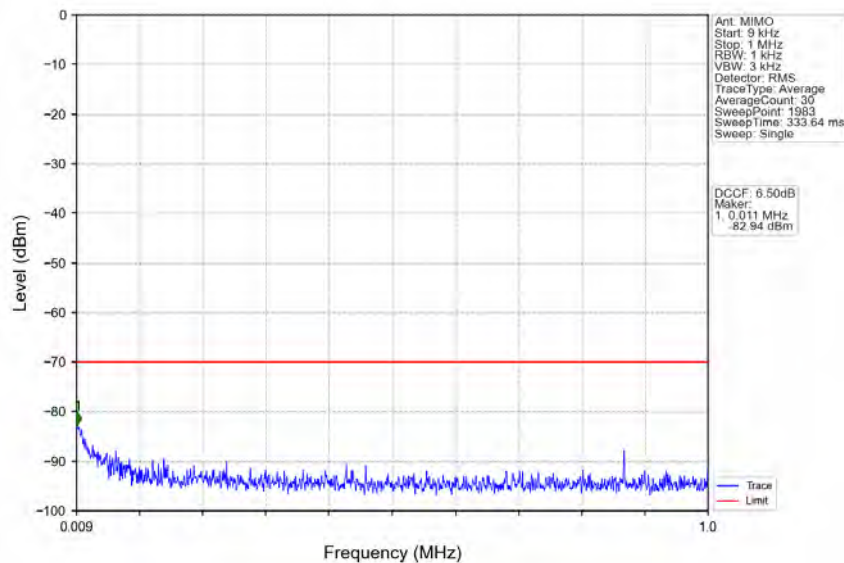
n78d_30kHz_MIMO_NTNV_30MHz_CP-OFDM_QPSK_3684.99MHz_Outer_Full
