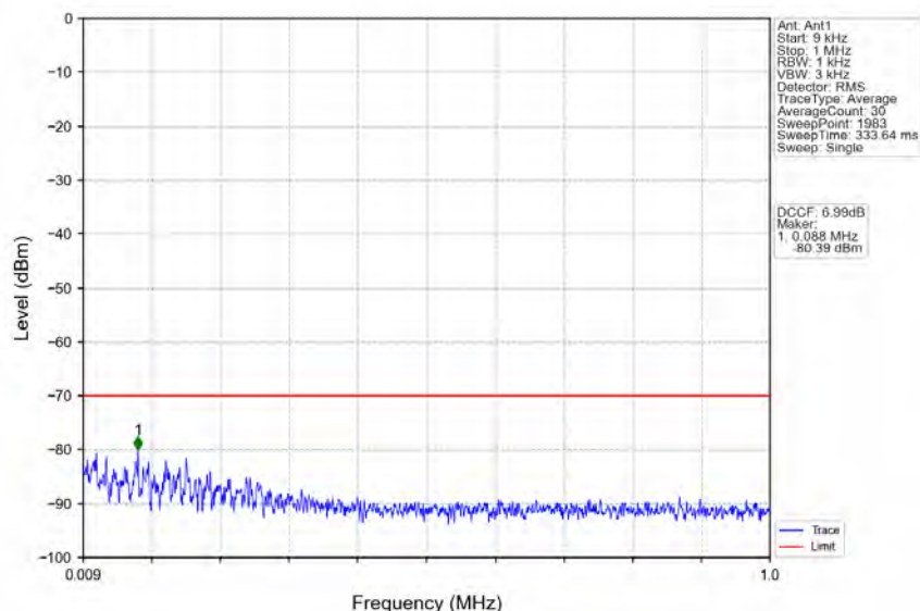
n78d_30kHz_MIMO_NTNV_30MHz_CP-OFDM_QPSK_3565.02MHz_Inner_1RB_Left
