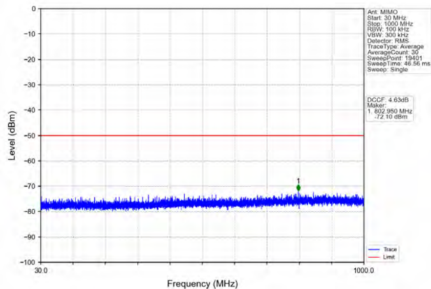
n78d_30kHz_MIMO_NTNV_50MHz_CP-OFDM_QPSK_3675MHz_Outer_Full
