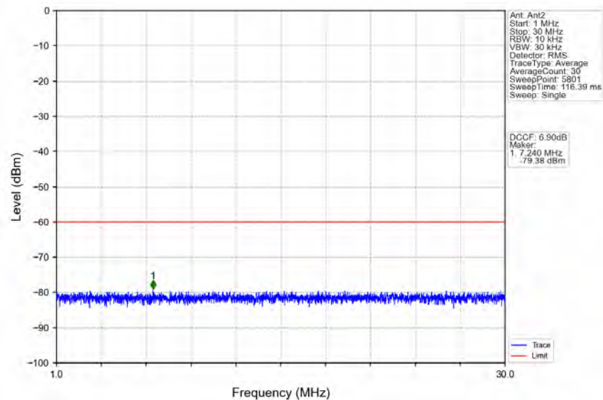
n78d_30kHz_MIMO_NTNV_50MHz_CP-OFDM_QPSK_3675MHz_Inner_1RB_Right
