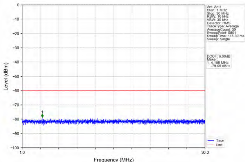
n78d_30kHz_MIMO_NTNV_40MHz_CP-OFDM_QPSK_3679.98MHz_Inner_1RB_Right
