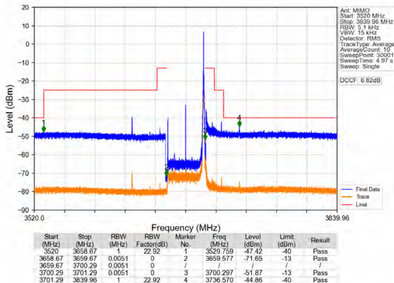
n78d_30kHz_MIMO_NTNV_40MHz_CP-OFDM_QPSK_3679.98MHz_Edge_1RB_Right
