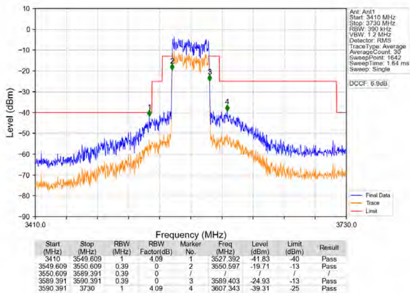
n78d_30kHz_MIMO_NTNV_40MHz_CP-OFDM QPSK_3570MHz_Outer_Full
