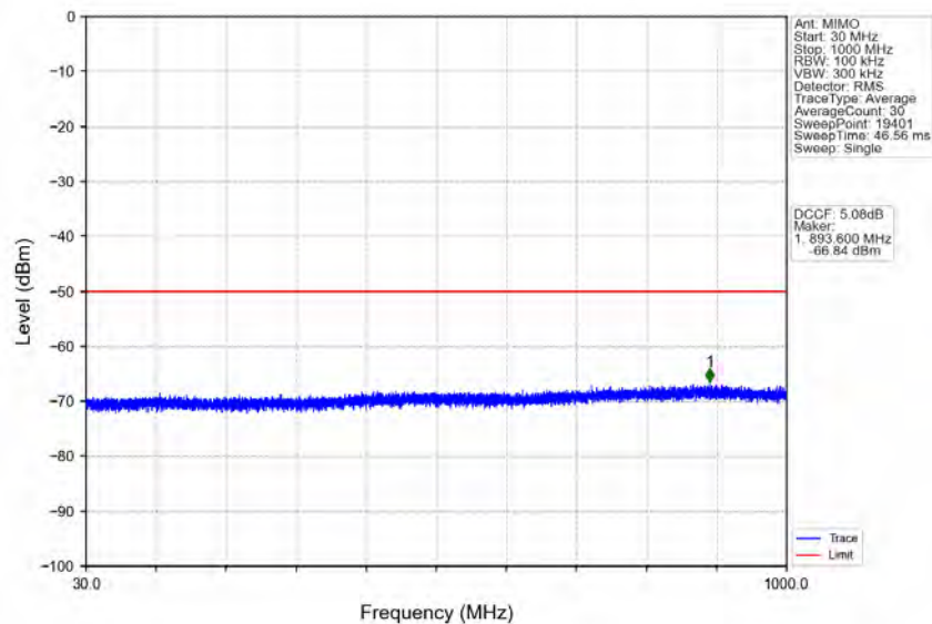
n78d_30kHz_MIMO_NTNV_50MHz_CP-OFDM QPSK_3675MHz_Edge_1RB_Right
