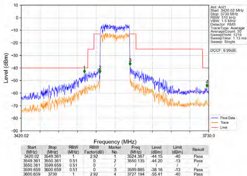
n78d_30kHz_MIMO_NTNV_50MHz_CP-OFDM_QPSK_3575.01MHz_Outer_Full
