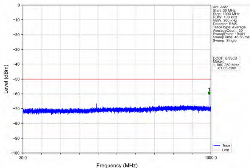
n78d_30kHz_MIMO_NTNV_30MHz_CP-OFDM_QPSK_3565.02MHz_Inner_1RB_Left
