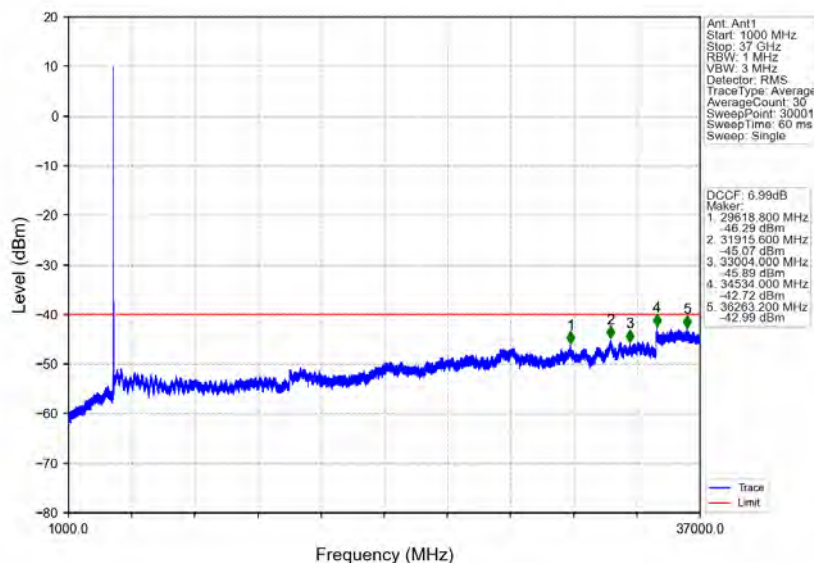
n78d_30kHz_MIMO_NTNV_40MHz_CP-OFDM_QPSK_3570MHz_Edge_1RB_Left
