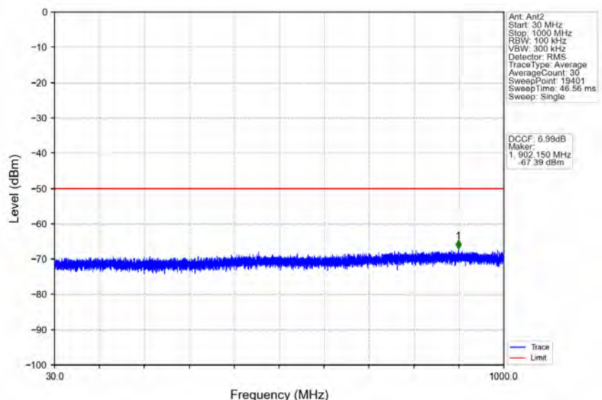
n78d_30kHz_MIMO_NTNV_50MHz_CP-OFDM_QPSK_3675MHz_Edge_1RB_Right
