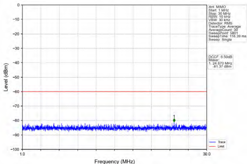
n78d_30kHz_MIMO_NTNV_30MHz_CP-OFDM QPSK_3684.99MHz_Outer_Full
