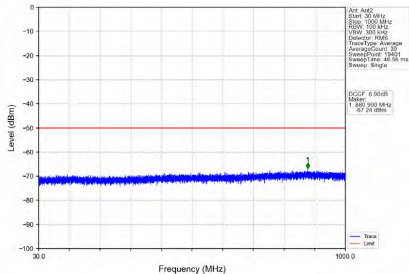
n78d_30kHz_MIMO_NTNV_50MHz_CP-OFDM_QPSK_3675MHz_Inner_1RB_Right
