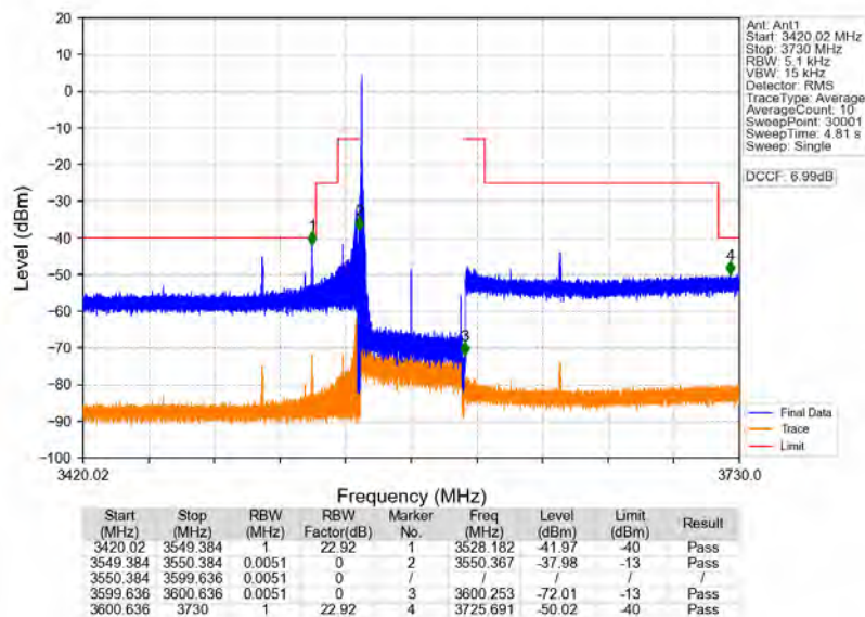
n78d_30kHz_MIMO_NTNV_50MHz_CP-OFDM_QPSK_3575.01MHz_Inner_1RB_Left
