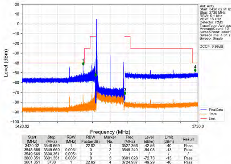
n78d_30kHz_MIMO_NTNV_50MHz_CP-OFDM_QPSK_3575.01MHz_Edge_1RB_Left
