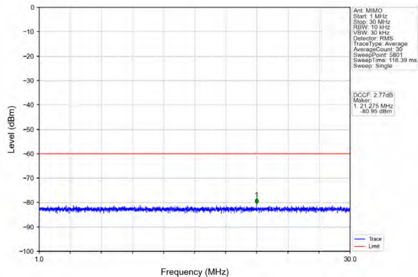
n78d_30kHz_MIMO_NTNV_60MHz_CP-OFDM_QPSK_3580.02MHz_Edge_1RB_Left
