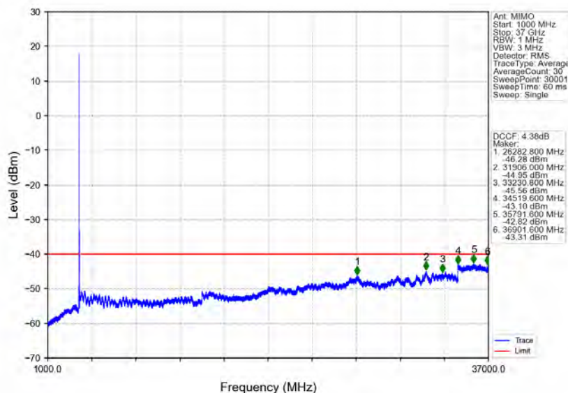
n78d_30kHz_MIMO_NTNV_30MHz_CP-OFDM_QPSK_3684.99MHz_Edge_1RB_Right
