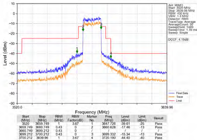
n78d_30kHz_MIMO_NTNV_40MHz_CP-OFDM_QPSK_3679.98MHz_Outer_Full
