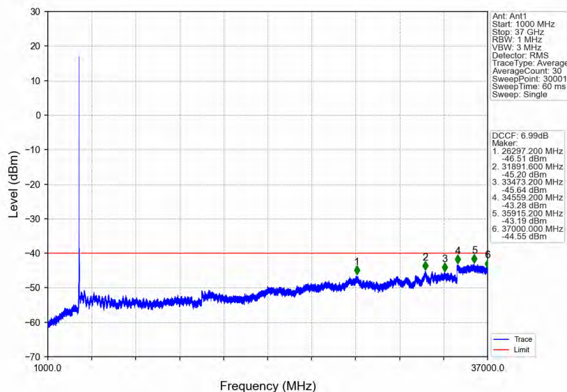
n78d_30kHz_MIMO_NTNV_50MHz_CP-OFDM_QPSK_3575.01MHz_Edge_1RB_Left
