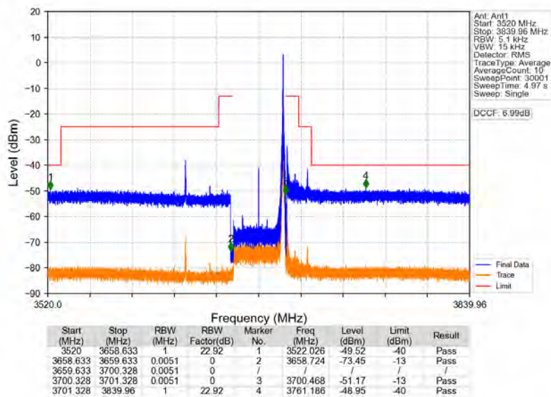
n78d_30kHz_MIMO_NTNV_40MHz_CP-OFDM_QPSK_3679.98MHz_Inner_1RB_Right
