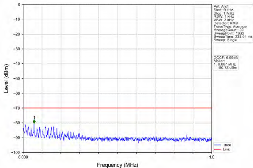
n78d_30kHz_MIMO_NTNV_30MHz_CP-OFDM_QPSK_3684.99MHz_Inner_1RB_Right
