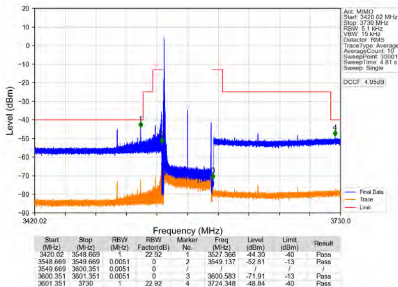
n78d_30kHz_MIMO_NTNV_50MHz_CP-OFDM_QPSK_3575.01MHz_Edge_1RB_Left
