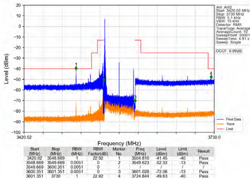
n78d_30kHz_MIMO_NTNV_50MHz_CP-OFDM_QPSK_3575.01MHz_Inner_1RB_Left
