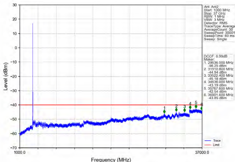
n78d_30kHz_MIMO_NTNV_30MHz_CP-OFDM_QPSK_3565.02MHz_Inner_1RB_Left
