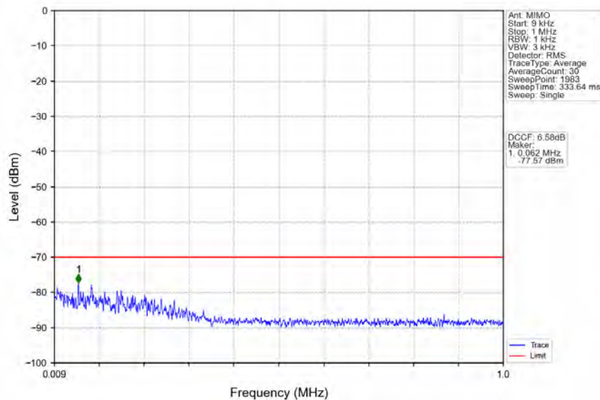
n78d_30kHz_MIMO_NTNV_40MHz_CP-OFDM_QPSK_3570MHz_Inner_1RB_Left
