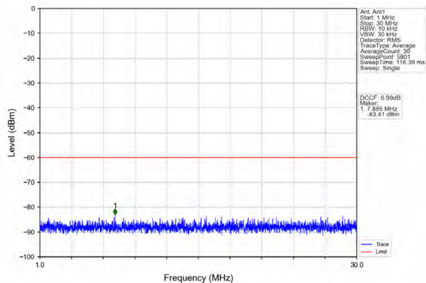
n78d_30kHz_MIMO_NTNV_40MHz_CP-OFDM_QPSK_3679.98MHz_Outer_Full
