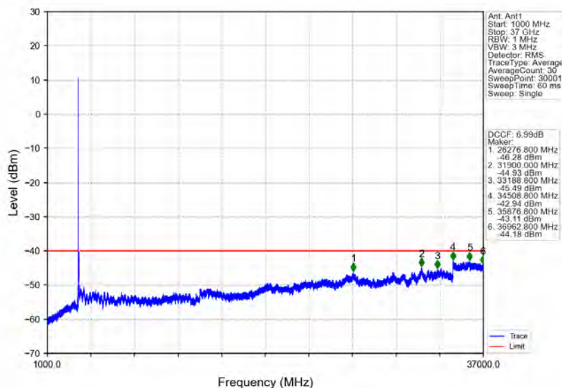
n78d_30kHz_MIMO_NTNV_60MHz_CP-OFDM_QPSK_3580.02MHz_Edge_1RB_Left
