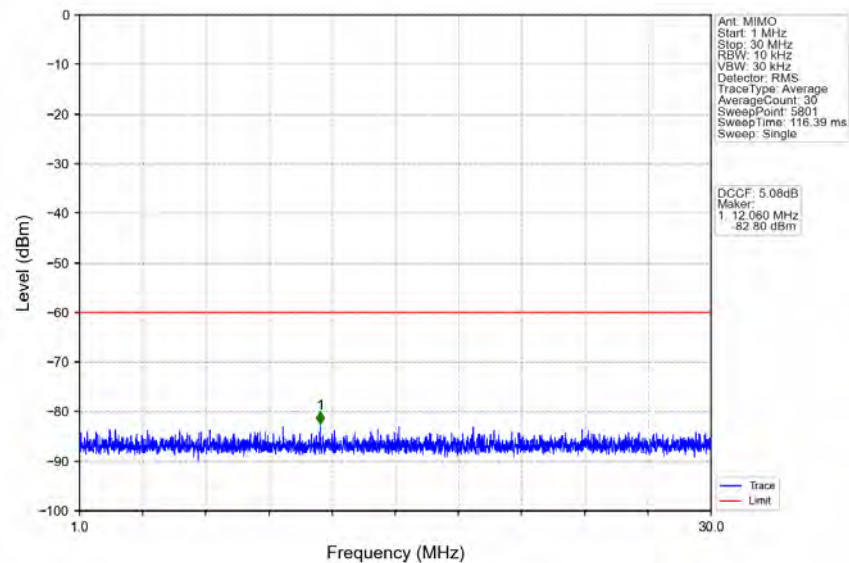
n78d_30kHz_MIMO_NTNV_50MHz_CP-OFDM_QPSK_3575.01MHz_Outer_Full
