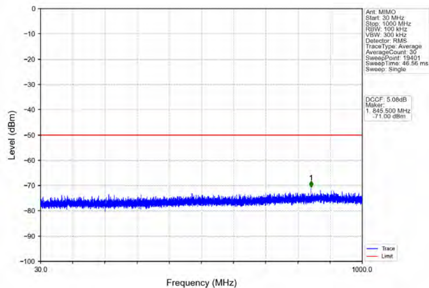
n78d_30kHz_MIMO_NTNV_50MHz_CP-OFDM QPSK_3575.01MHz_Outer_Full
