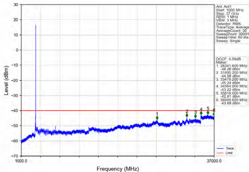
n78d_30kHz_MIMO_NTNV_40MHz_CP-OFDM QPSK_3679.98MHz_Edge_1RB_Right
