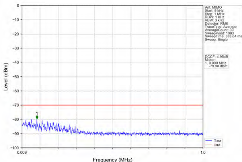
n78d_30kHz_MIMO_NTNV_50MHz_CP-OFDM_QPSK_3575.01MHz_Edge_1RB_Left
