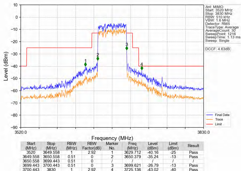
n78d_30kHz_MIMO_NTNV_50MHz_CP-OFDM_QPSK_3675MHz_Outer_Full
