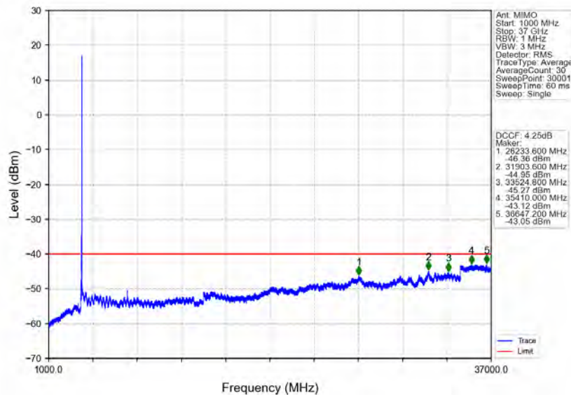
n78d_30kHz_MIMO_NTNV_40MHz_CP-OFDM QPSK_3679.98MHz_Inner_1RB_Right
