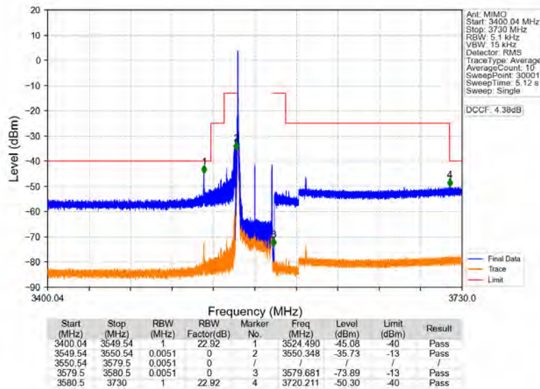
n78d_30kHz_MIMO_NTNV_30MHz_CP-OFDM_QPSK_3565.02MHz_Inner_1RB_Left
