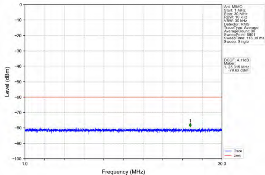
n78d_30kHz_MIMO_NTNV_50MHz_CP-OFDM_QPSK_3575.01MHz_Inner_1RB_Left
