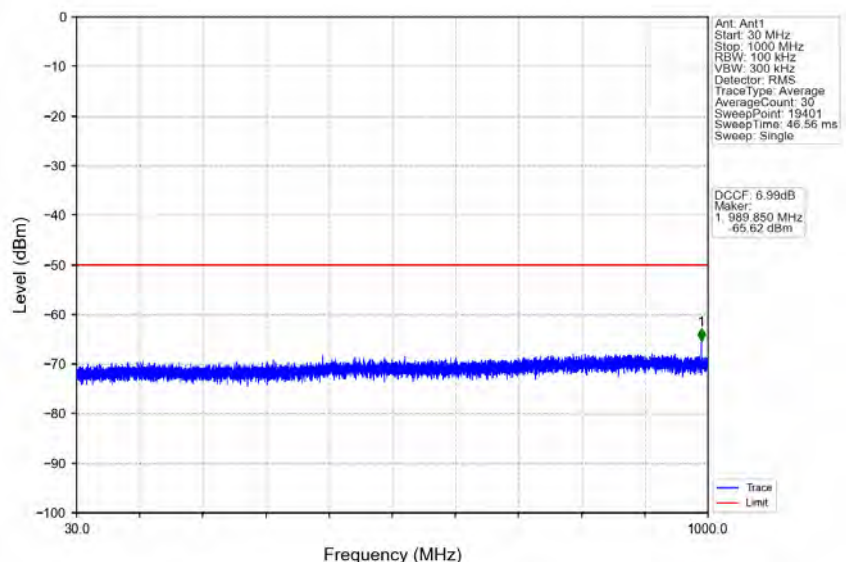
n78d_30kHz_MIMO_NTNV_40MHz_CP-OFDM_QPSK_3570MHz_Edge_1RB_Left
