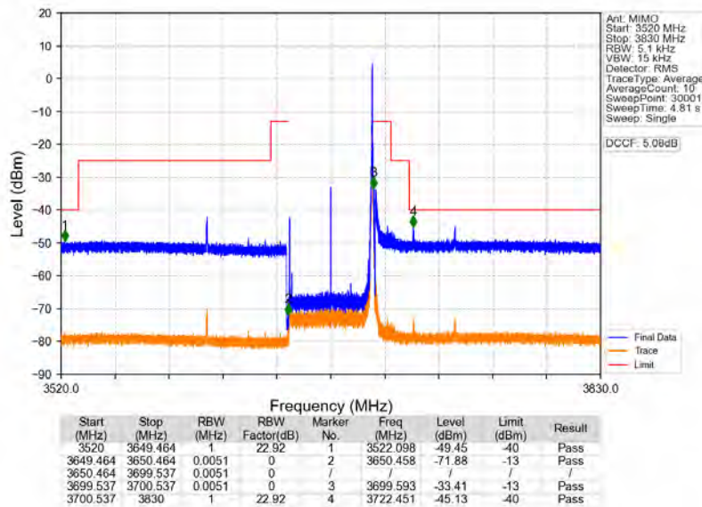
n78d_30kHz_MIMO_NTNV_50MHz_CP-OFDM_QPSK_3675MHz_Edge_1RB_Right
