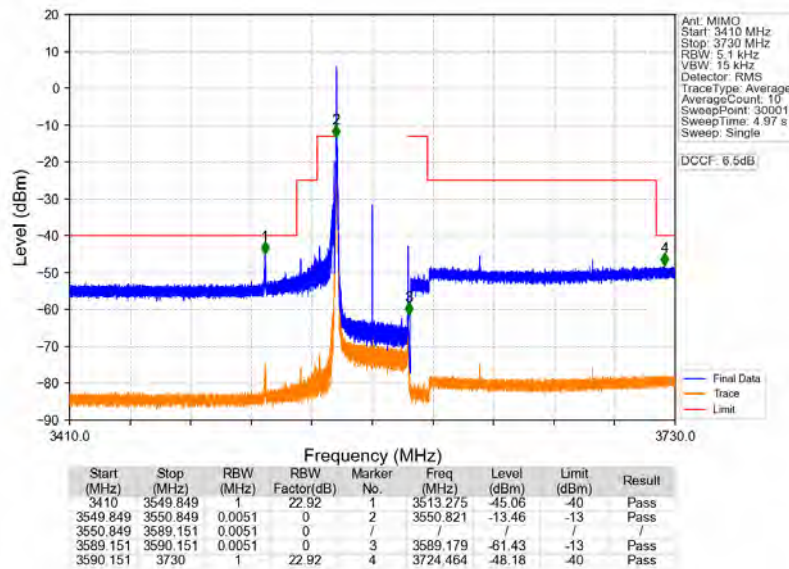
n78d_30kHz_MIMO_NTNV_40MHz_CP-OFDM_QPSK_3570MHz_Edge_1RB_Left
