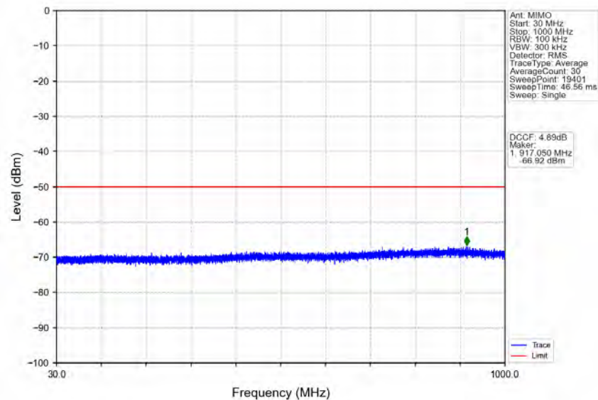
n78d_30kHz_MIMO_NTNV_30MHz_CP-OFDM QPSK_3684.99MHz_Edge_1RB_Right
