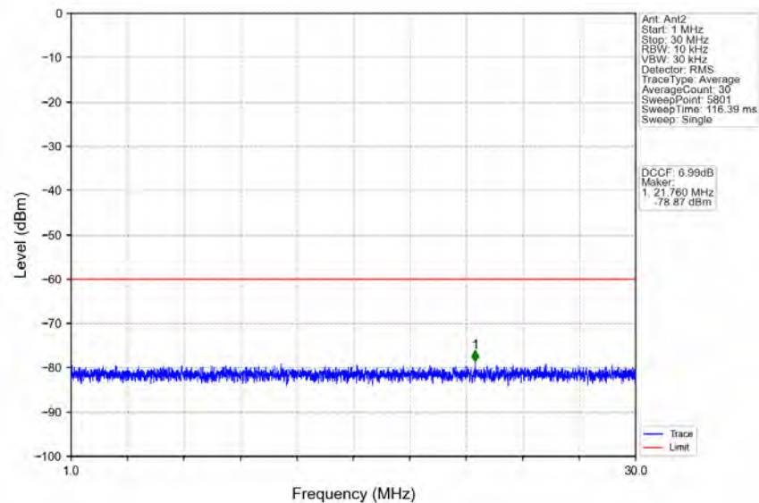
n78d_30kHz_MIMO_NTNV_40MHz_CP-OFDM_QPSK_3570MHz_Inner_1RB_Left
