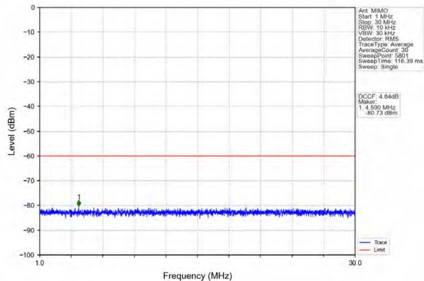
n78d_30kHz_MIMO_NTNV_40MHz_CP-OFDM_QPSK_3570MHz_Outer_Full
