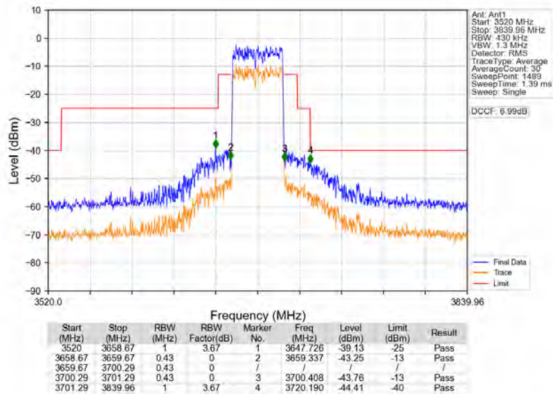
n78d_30kHz_MIMO_NTNV_40MHz_CP-OFDM_QPSK_3679.98MHz_Outer_Full
