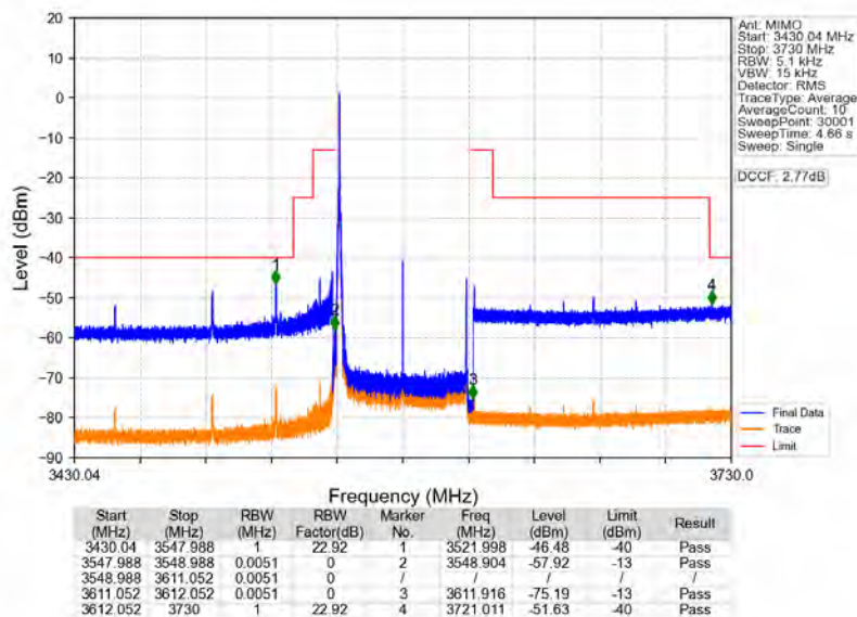
n78d_30kHz_MIMO_NTNV_60MHz_CP-OFDM_QPSK_3580.02MHz_Edge_1RB_Left
