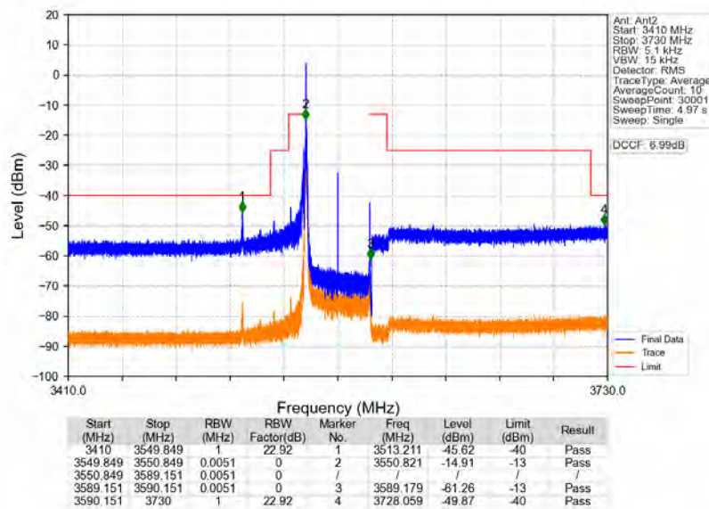
n78d_30kHz_MIMO_NTNV_40MHz_CP-OFDM_QPSK_3570MHz_Edge_1RB_Left
