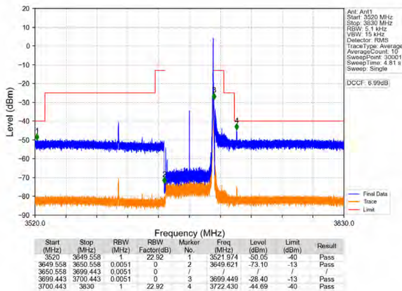
n78d_30kHz_MIMO_NTNV_50MHz_CP-OFDM_QPSK_3675MHz_Edge_1RB_Right
