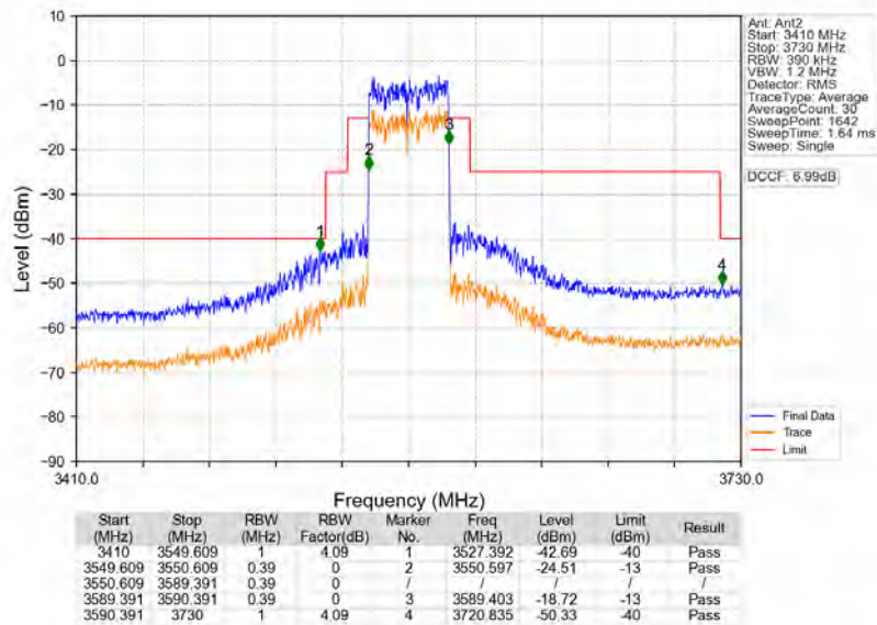
n78d_30kHz_MIMO_NTNV_40MHz_CP-OFDM_QPSK_3570MHz_Outer_Full
