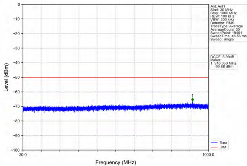
n78d_30kHz_MIMO_NTNV_30MHz_CP-OFDM_QPSK_3684.99MHz_Edge_1RB_Right
