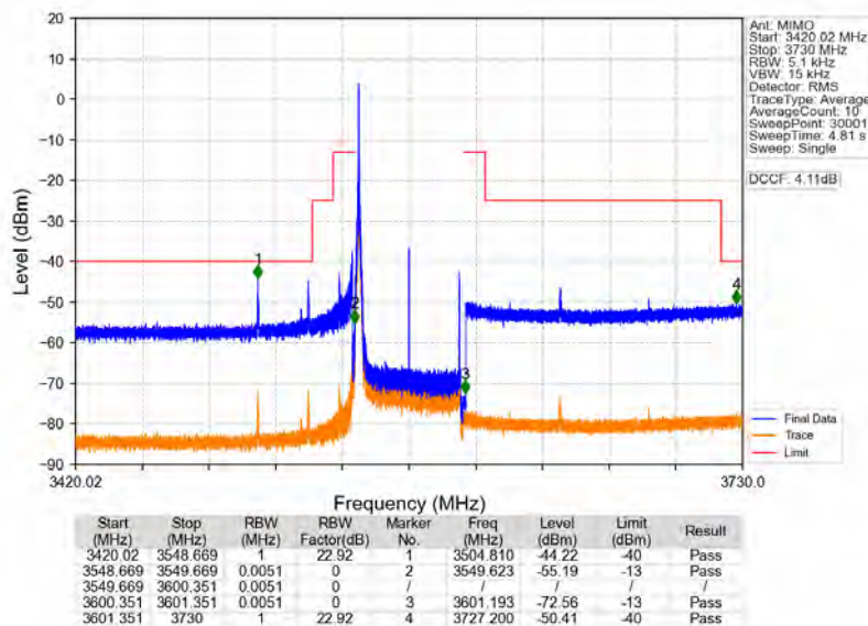
n78d_30kHz_MIMO_NTNV_50MHz_CP-OFDM_QPSK_3575.01MHz_Inner_1RB_Left
