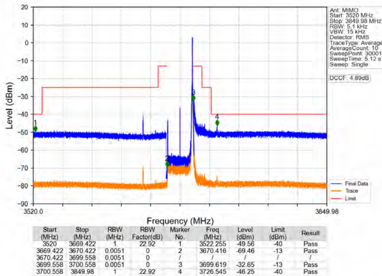
n78d_30kHz_MIMO_NTNV_30MHz_CP-OFDM_QPSK_3684.99MHz_Edge_1RB_Right
