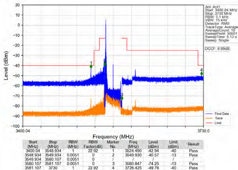
n78d_30kHz_MIMO_NTNV_30MHz_CP-OFDM_QPSK_3565.02MHz_Inner_1RB_Left
