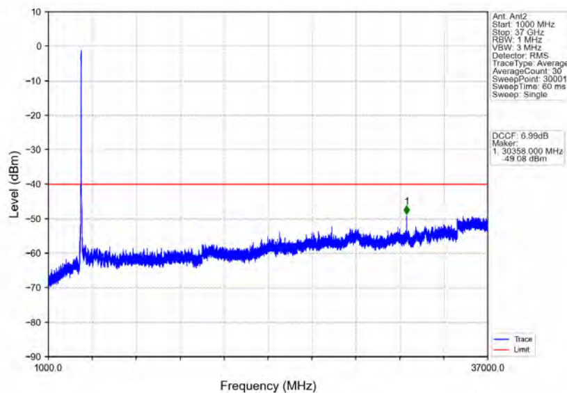
n78d_30kHz_MIMO_NTNV_40MHz_CP-OFDM QPSK_3679.98MHz_Outer_Full
