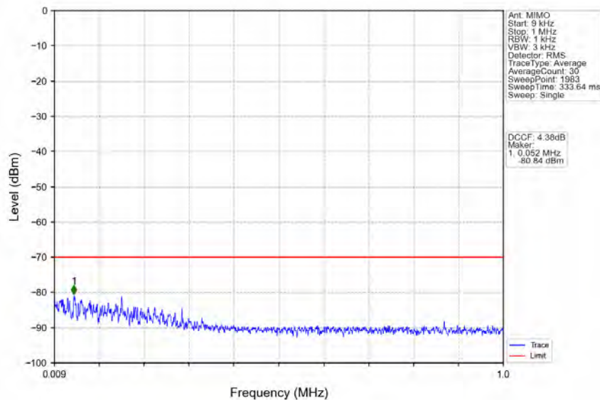
n78d_30kHz_MIMO_NTNV_30MHz_CP-OFDM_QPSK_3565.02MHz_Inner_1RB_Left
