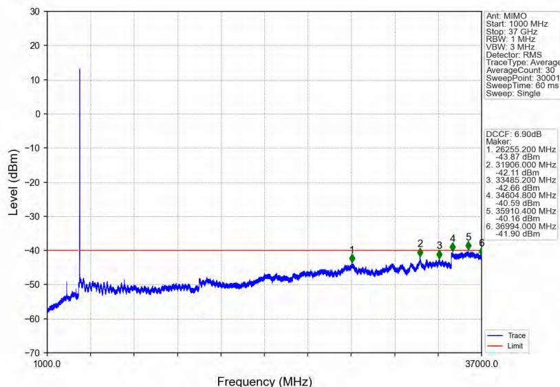
n78d_30kHz_MIMO_NTNV_30MHz_CP-OFDM QPSK_3684.99MHz_Inner_1RB_Right
