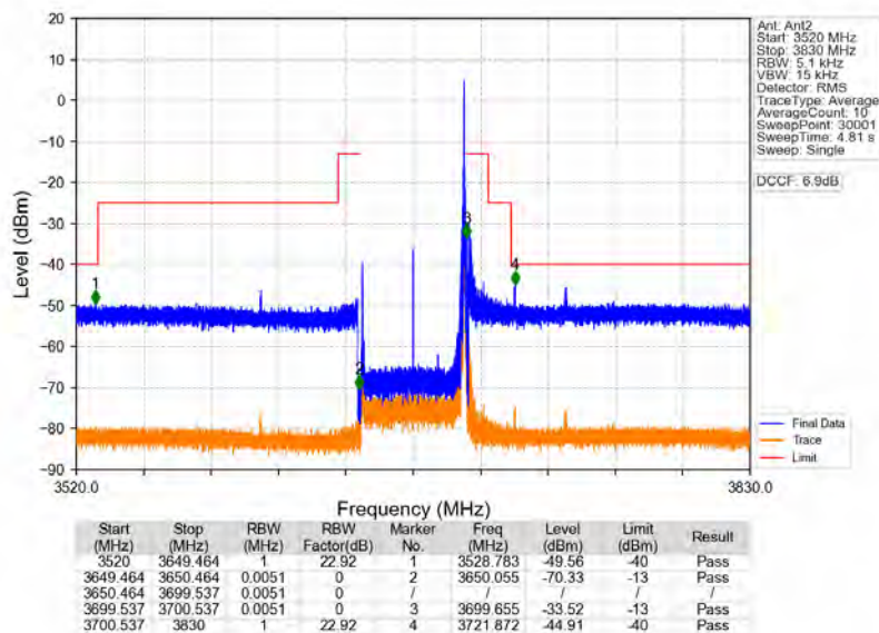
n78d_30kHz_MIMO_NTNV_50MHz_CP-OFDM_QPSK_3675MHz_Inner_1RB_Right
