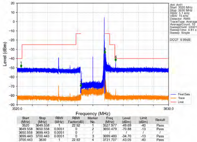
n78d_30kHz_MIMO_NTNV_50MHz_CP-OFDM_QPSK_3675MHz_Inner_1RB_Right
