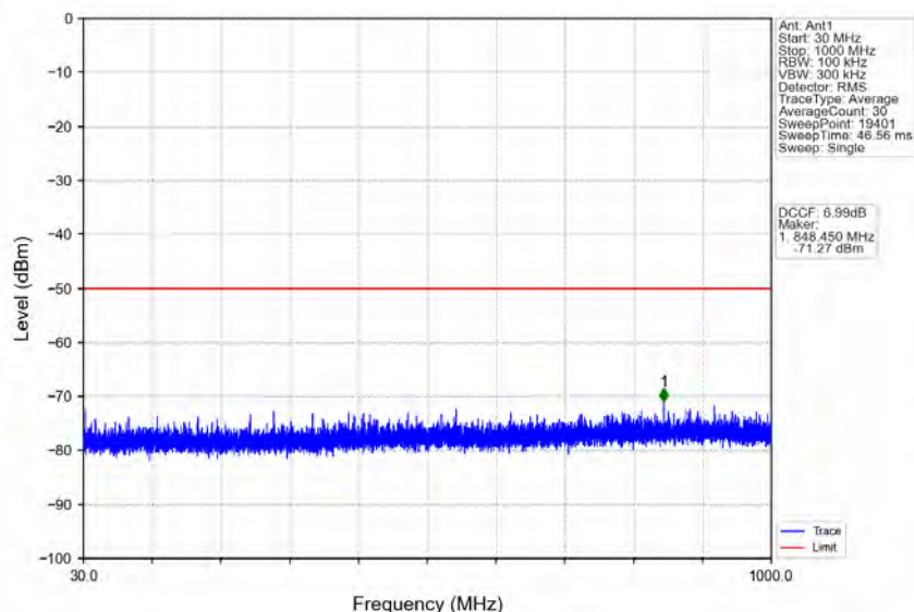
n78d_30kHz_MIMO_NTNV_50MHz_CP-OFDM_QPSK_3675MHz_Outer_Full
