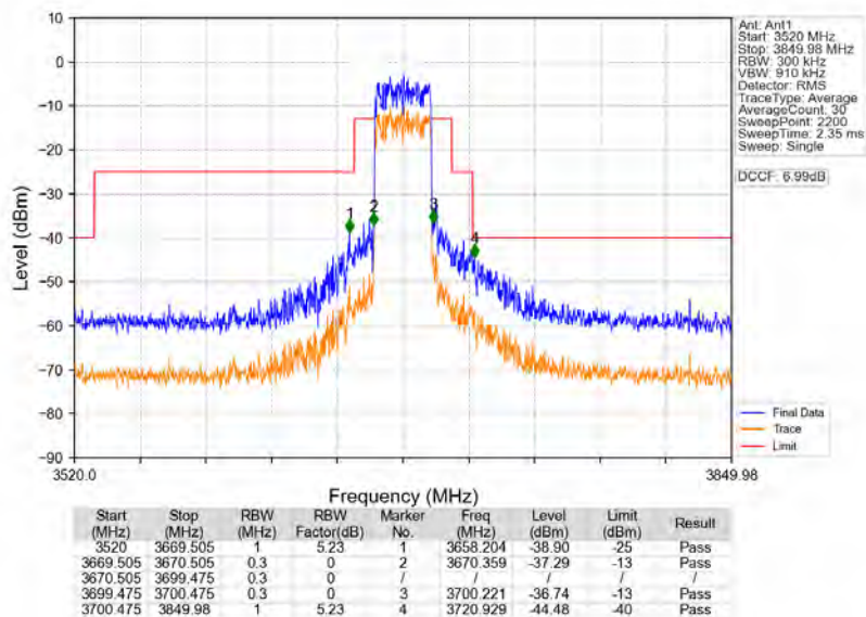
n78d_30kHz_MIMO_NTNV_30MHz_CP-OFDM_QPSK_3684.99MHz_Outer_Full
