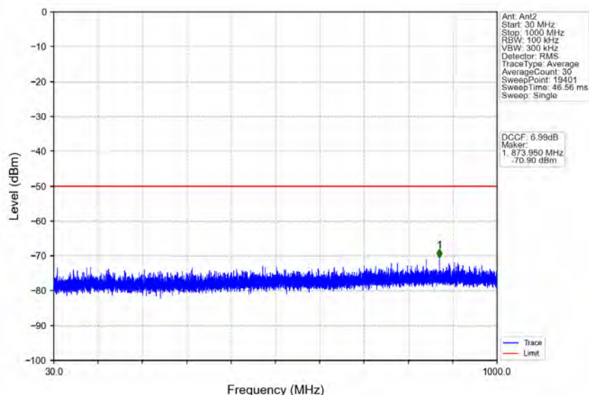
n78d_30kHz_MIMO_NTNV_50MHz_CP-OFDM_QPSK_3575.01MHz_Outer_Full
