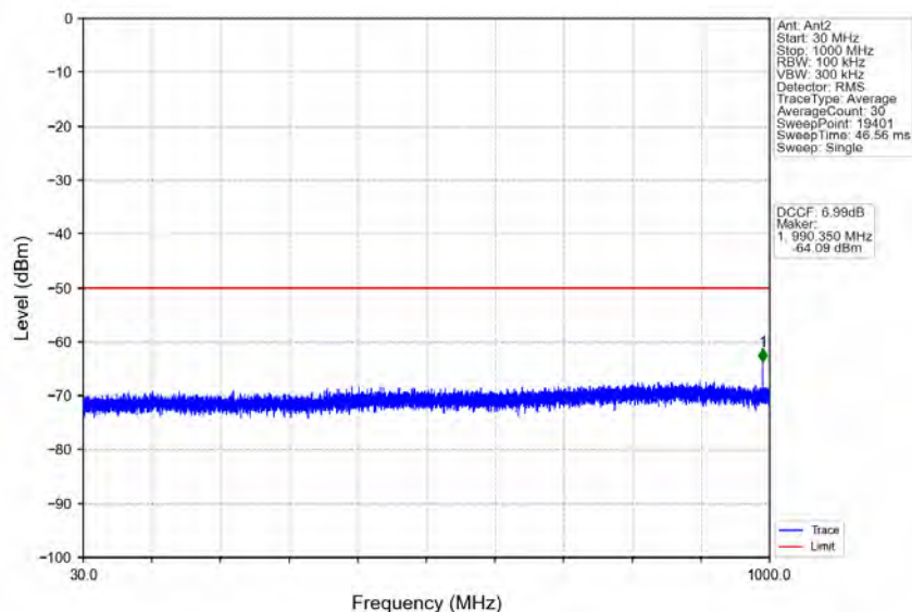
n78d_30kHz_MIMO_NTNV_50MHz_CP-OFDM_QPSK_3575.01MHz_Inner_1RB_Left
