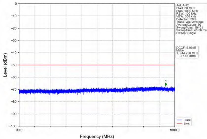
n78d_30kHz_MIMO_NTNV_40MHz_CP-OFDM QPSK_3679.98MHz_Edge_1RB_Right
