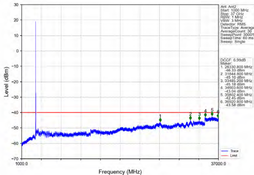
n78d_30kHz_MIMO_NTNV_40MHz_CP-OFDM_QPSK_3570MHz_Inner_1RB_Left
