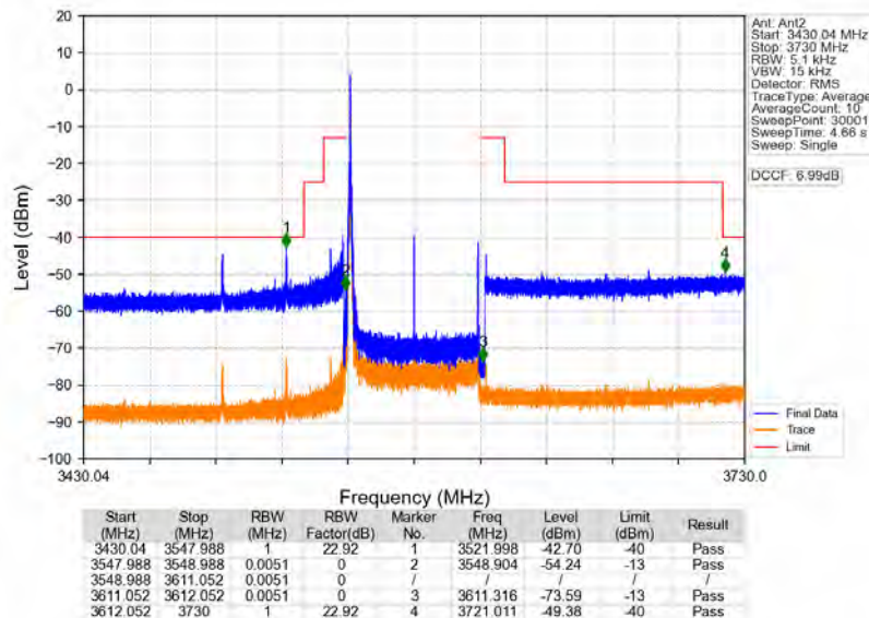
n78d_30kHz_MIMO_NTNV_60MHz_CP-OFDM_QPSK_3580.02MHz_Edge_1RB_Left
