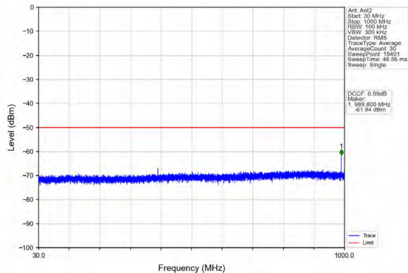
n78d_30kHz_MIMO_NTNV_40MHz_CP-OFDM_QPSK_3570MHz_Edge_1RB_Left
