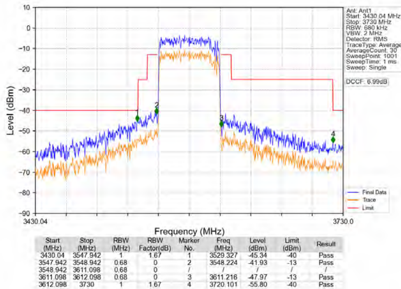
n78d_30kHz_MIMO_NTNV_60MHz_CP-OFDM_QPSK_3580.02MHz_Outer_Full
