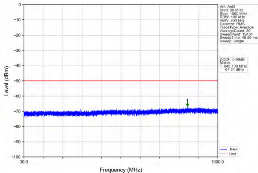
n78d_30kHz_MIMO_NTNV_40MHz_CP-OFDM_QPSK_3679.98MHz_Inner_1RB_Right
