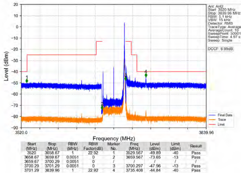
n78d_30kHz_MIMO_NTNV_40MHz_CP-OFDM_QPSK_3679.98MHz_Inner_1RB_Right
