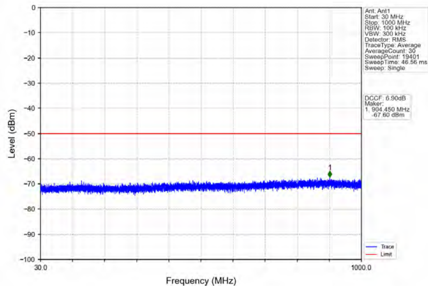
n78d_30kHz_MIMO_NTNV_40MHz_CP-OFDM_QPSK_3570MHz_Outer_Full
