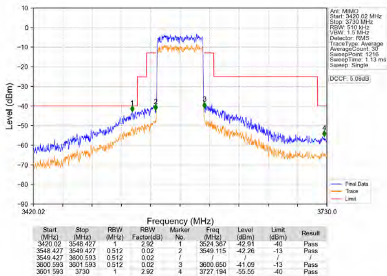
n78d_30kHz_MIMO_NTNV_50MHz_CP-OFDM_QPSK_3575.01MHz_Outer_Full
