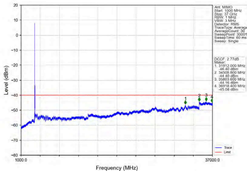
n78d_30kHz_MIMO_NTNV_60MHz_CP-OFDM_QPSK_3580.02MHz_Outer_Full
