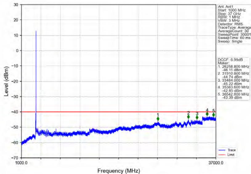
n78d_30kHz_MIMO_NTNV_50MHz_CP-OFDM QPSK_3675MHz_Edge_1RB_Right
