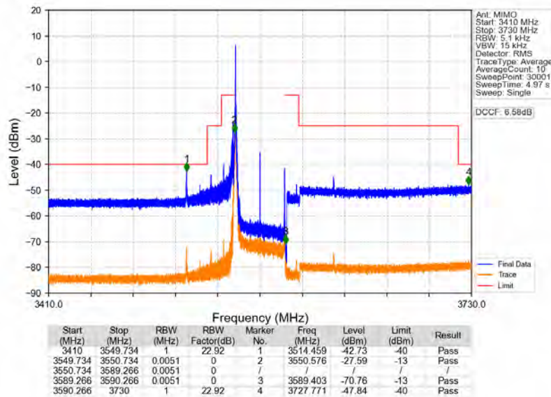
n78d_30kHz_MIMO_NTNV_40MHz_CP-OFDM_QPSK_3570MHz_Inner_1RB_Left
