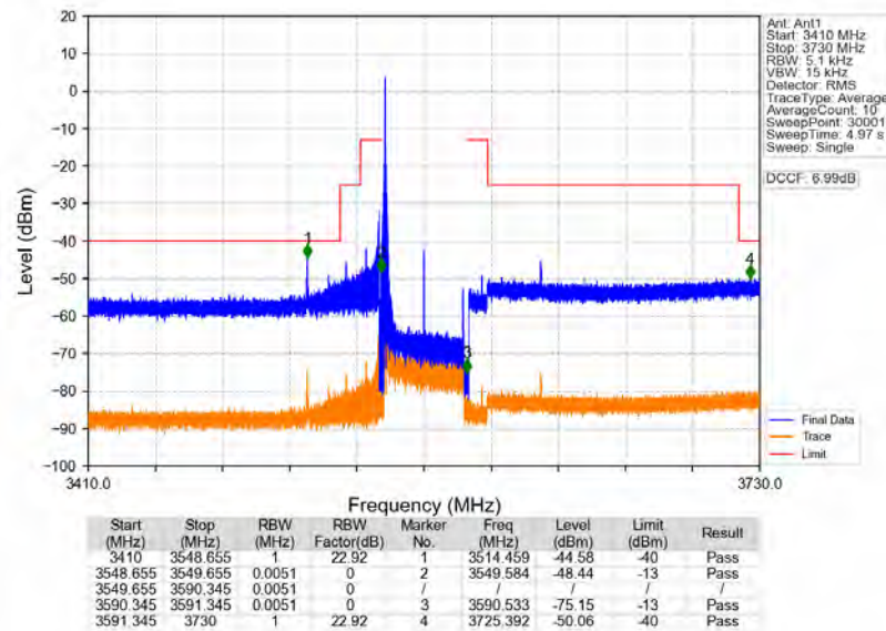
n78d_30kHz_MIMO_NTNV_40MHz_CP-OFDM_QPSK_3570MHz_Inner_1RB_Left
