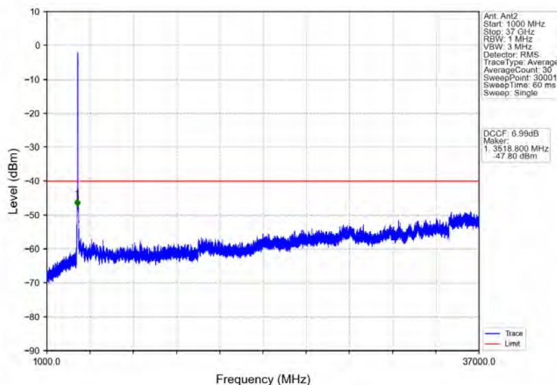
n78d_30kHz_MIMO_NTNV_50MHz_CP-OFDM_QPSK_3575.01MHz_Outer_Full
