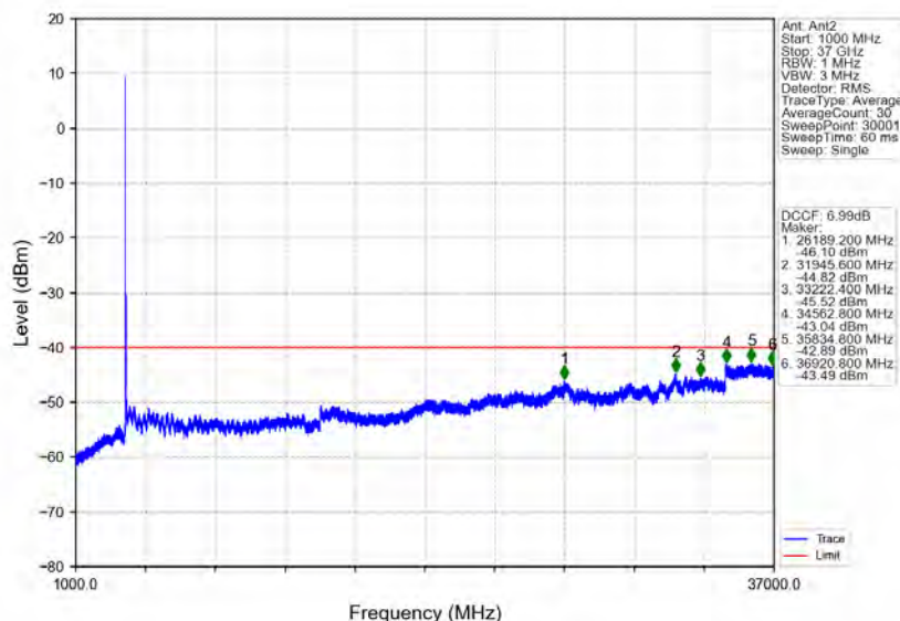
n78d_30kHz_MIMO_NTNV_50MHz_CP-OFDM_QPSK_3575.01MHz_Inner_1RB_Left
