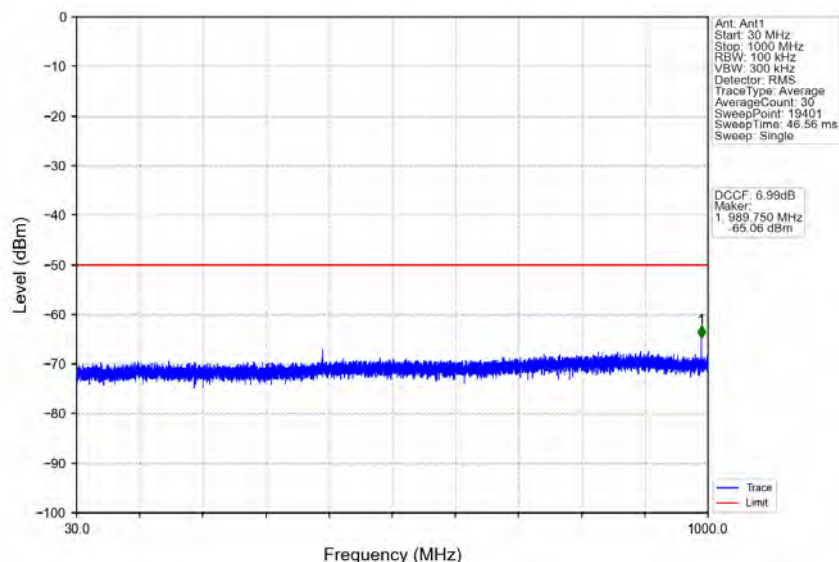
n78d_30kHz_MIMO_NTNV_60MHz_CP-OFDM_QPSK_3580.02MHz_Edge_1RB_Left
