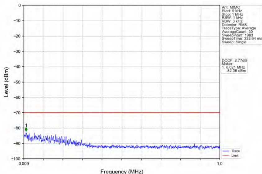
n78d_30kHz_MIMO_NTNV_60MHz_CP-OFDM_QPSK_3580.02MHz_Edge_1RB_Left
