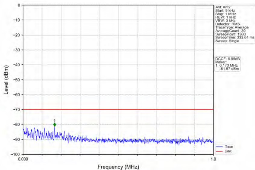
n78d_30kHz_MIMO_NTNV_30MHz_CP-OFDM_QPSK_3684.99MHz_Edge_1RB_Right
