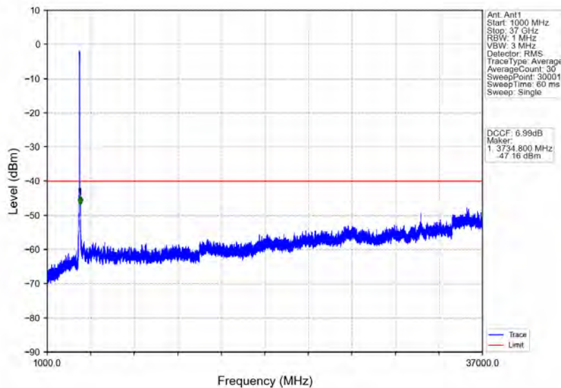
n78d_30kHz_MIMO_NTNV_50MHz_CP-OFDM_QPSK_3675MHz_Outer_Full
