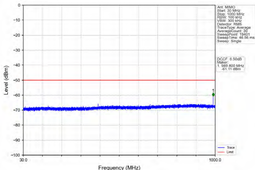
n78d_30kHz_MIMO_NTNV_40MHz_CP-OFDM_QPSK_3570MHz_Edge_1RB_Left
