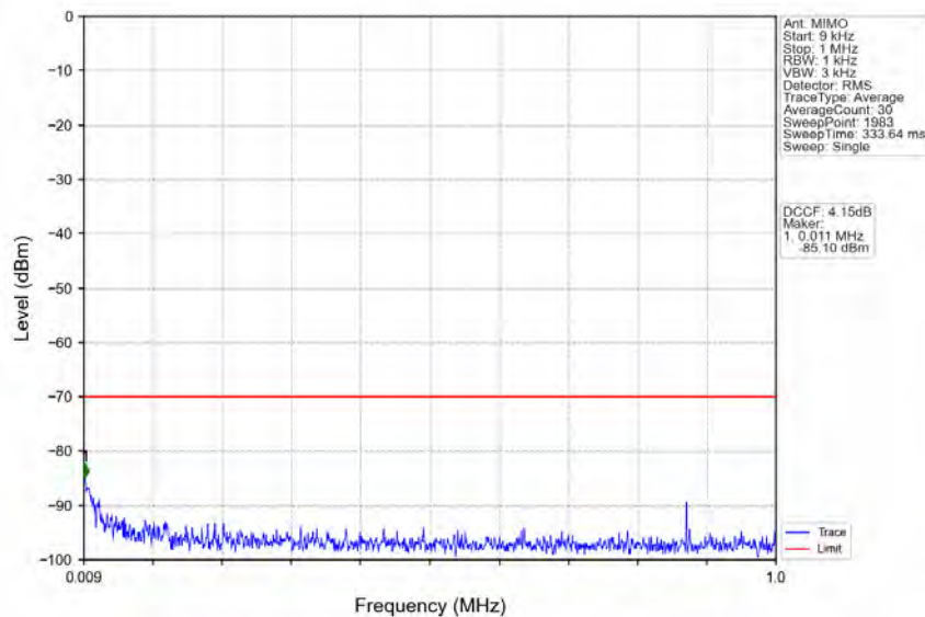
n78d_30kHz_MIMO_NTNV_40MHz_CP-OFDM_QPSK_3679.98MHz_Outer_Full
