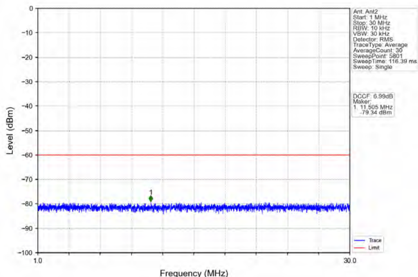
n78d_30kHz_MIMO_NTNV_50MHz_CP-OFDM_QPSK_3575.01MHz_Edge_1RB_Left
