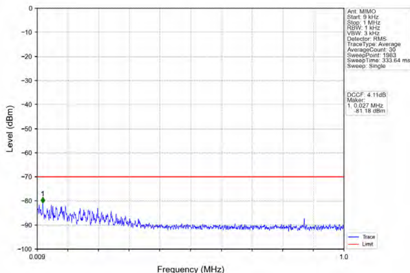
n78d_30kHz_MIMO_NTNV_50MHz_CP-OFDM_QPSK_3575.01MHz_Inner_1RB_Left
