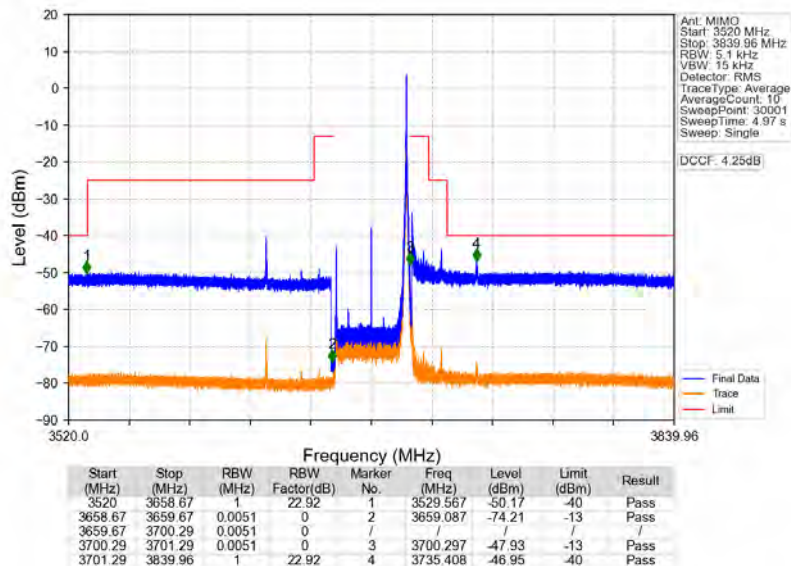
n78d_30kHz_MIMO_NTNV_40MHz_CP-OFDM_QPSK_3679.98MHz_Inner_1RB_Right
