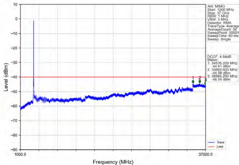
n78d_30kHz_MIMO_NTNV_40MHz_CP-OFDM_QPSK_3570MHz_Outer_Full
