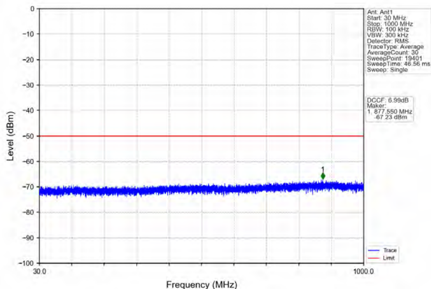
n78d_30kHz_MIMO_NTNV_30MHz_CP-OFDM_QPSK_3684.99MHz_Inner_1RB_Right
