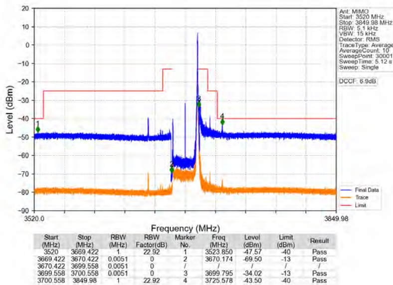
n78d_30kHz_MIMO_NTNV_30MHz_CP-OFDM_QPSK_3684.99MHz_Inner_1RB_Right
