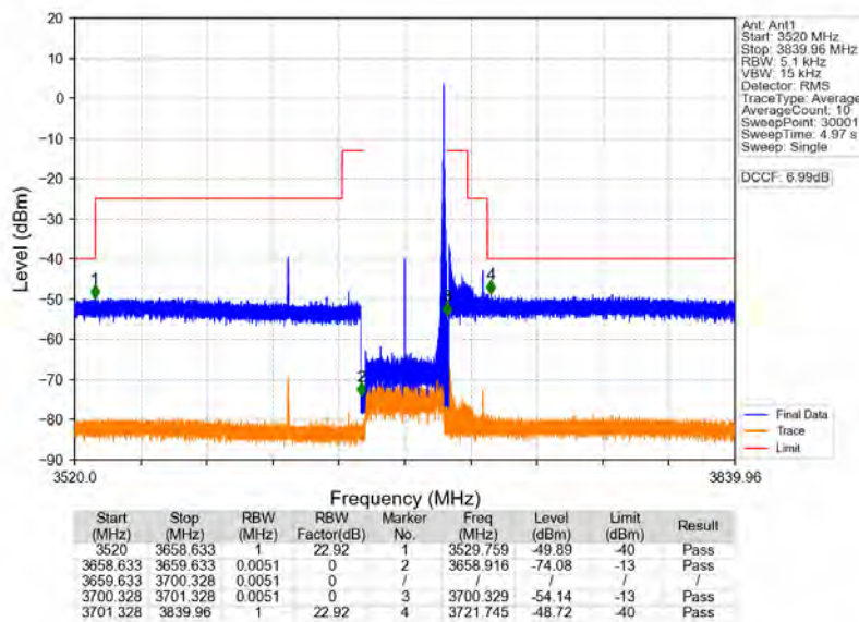
n78d_30kHz_MIMO_NTNV_40MHz_CP-OFDM QPSK_3679.98MHz_Edge_1RB_Right
