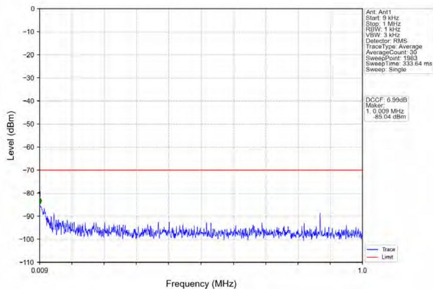
n78d_30kHz_MIMO_NTNV_50MHz_CP-OFDM_QPSK_3675MHz_Outer_Full
