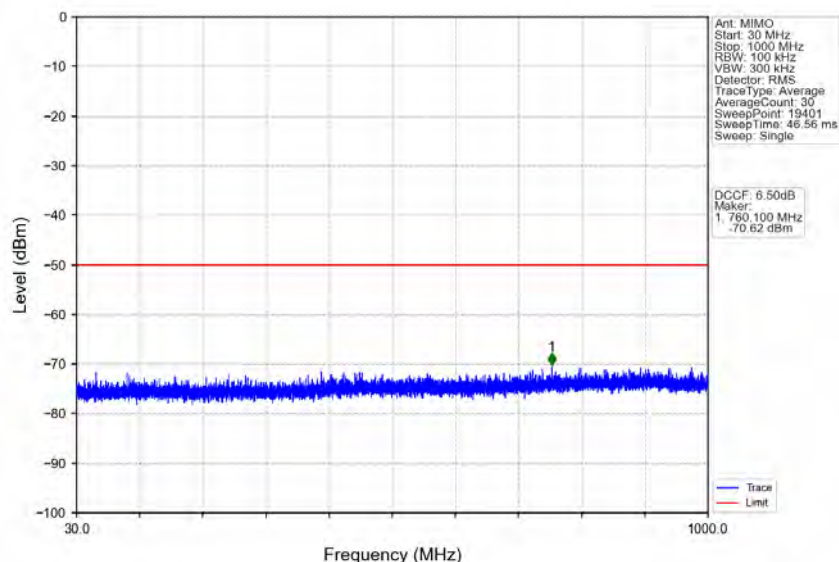
n78d_30kHz_MIMO_NTNV_30MHz_CP-OFDM QPSK_3684.99MHz_Outer_Full
