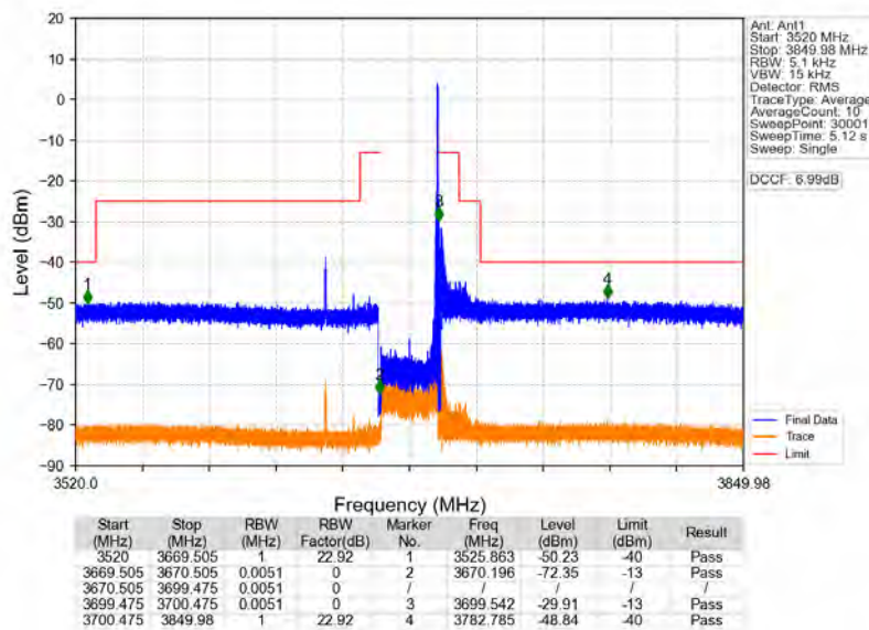
n78d_30kHz_MIMO_NTNV_30MHz_CP-OFDM_QPSK_3684.99MHz_Edge_1RB_Right
