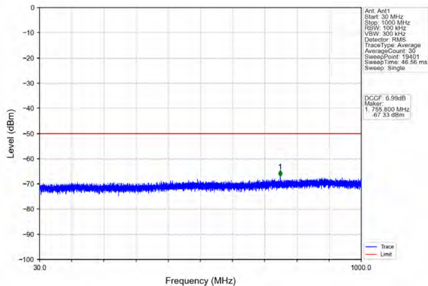
n78d_30kHz_MIMO_NTNV_50MHz_CP-OFDM_QPSK_3675MHz_Inner_1RB_Right
