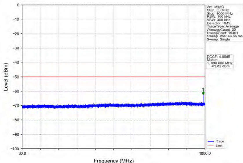
n78d_30kHz_MIMO_NTNV_50MHz_CP-OFDM_QPSK_3575.01MHz_Edge_1RB_Left
