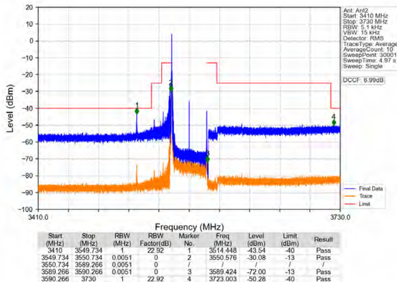
n78d_30kHz_MIMO_NTNV_40MHz_CP-OFDM_QPSK_3570MHz_Inner_1RB_Left
