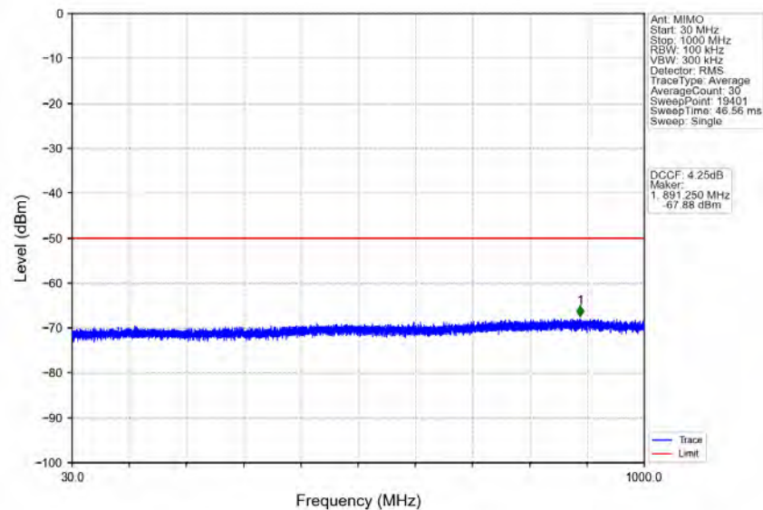
n78d_30kHz_MIMO_NTNV_40MHz_CP-OFDM QPSK_3679.98MHz_Inner_1RB_Right
