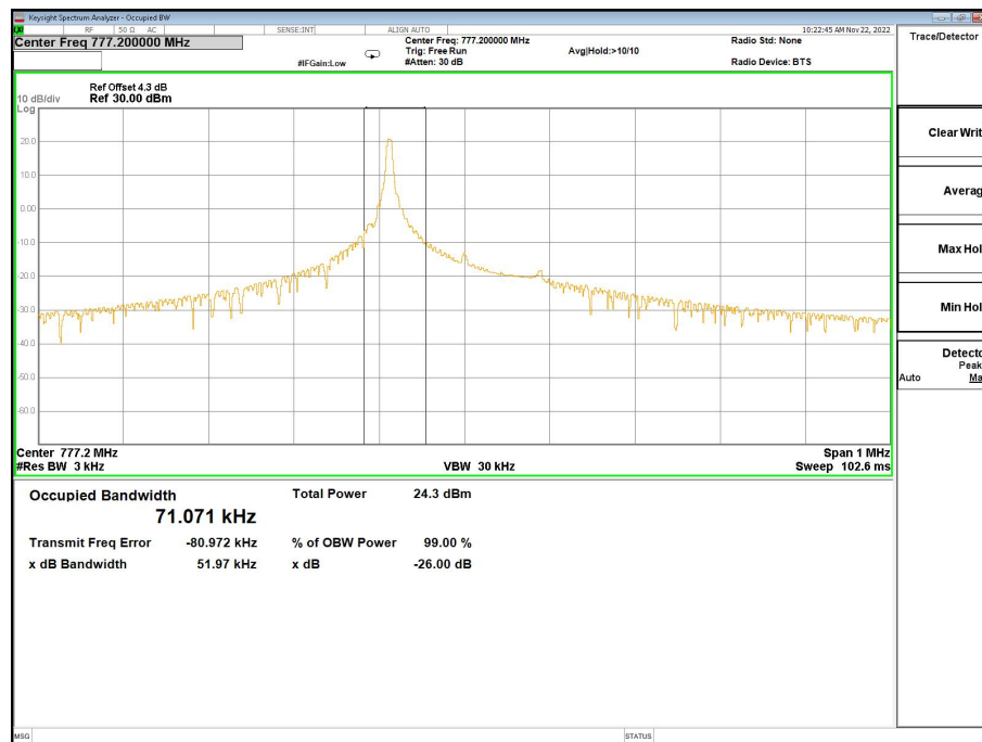
Band13-26dB/99% OBW-23182 Channel-BPSK-1@0-3.75K
