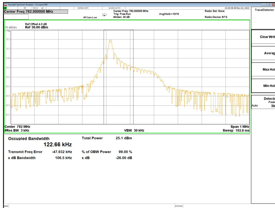
Band13-26dB/99% OBW-23230 Channel-BPSK-1@0-15K
