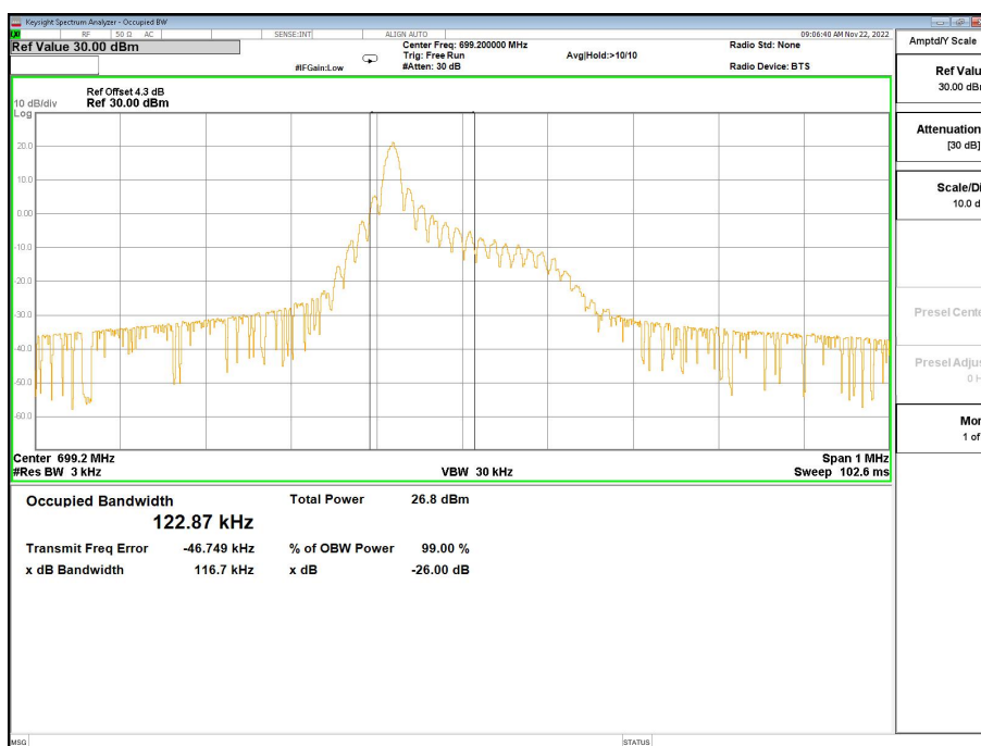
Band12-26dB/99% OBW-23012 Channel-QPSK-1@0-15K
