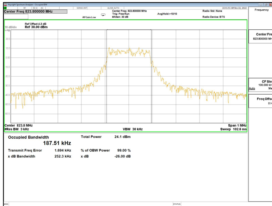
Band26-26dB/99% OBW-26788 Channel-QPSK-12@0-15K
