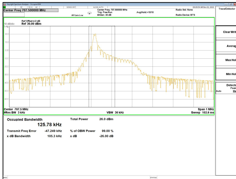
Band12-26dB/99% OBW-23095 Channel-BPSK-1@0-15K
