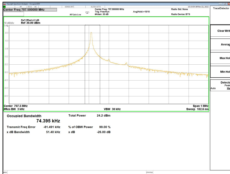
Band12-26dB/99% OBW-23095 Channel-BPSK-1@0-3.75K
