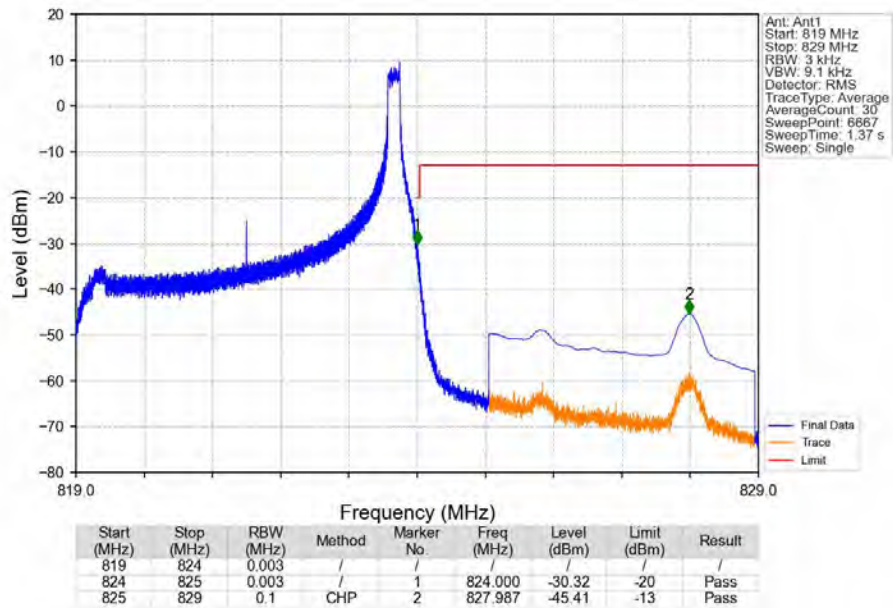
Band26a_5MHz_QPSK_HCH_821.5MHz_RB_1_24_NTNV
