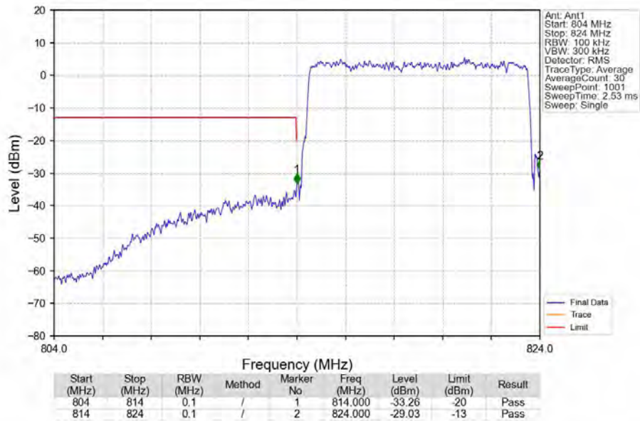
Band26a_10MHz_16QAM_LCH_819MHz_RB_50_0_NTNV
