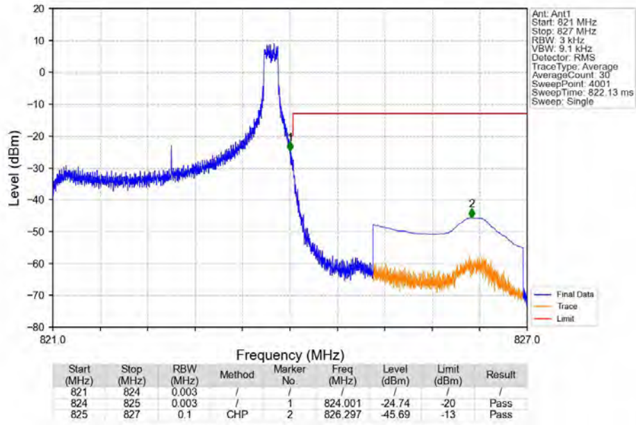
Band26a 3MHz 16QAM HCH 822.5MHz RB 1 14 NTN
