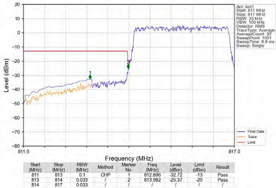
Band26a_3MHz_16QAM_LCH_815.5MHz_RB_15_0_NTNV
