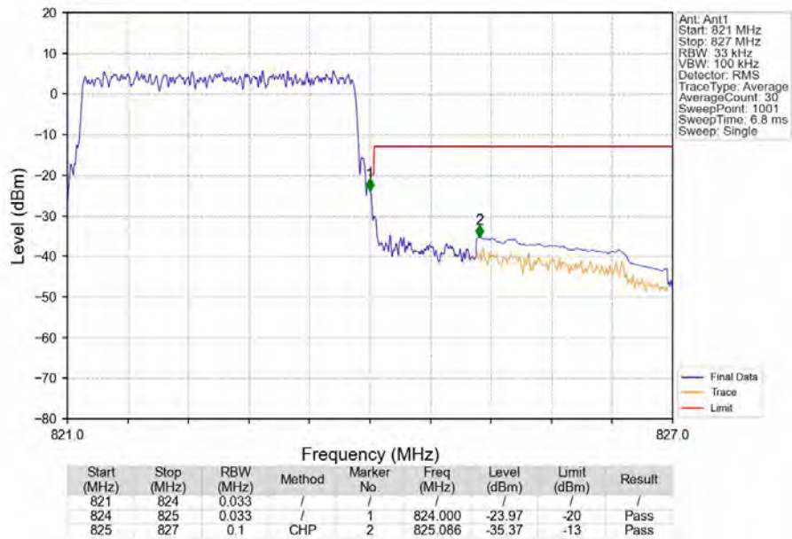
Band26a 3MHz 16QAM HCH 822.5MHz RB 15 0 NTN
