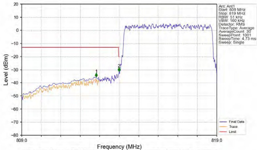
Band26a_5MHz_16QAM_LCH_816.5MHz_RB_25_0_NTNV
