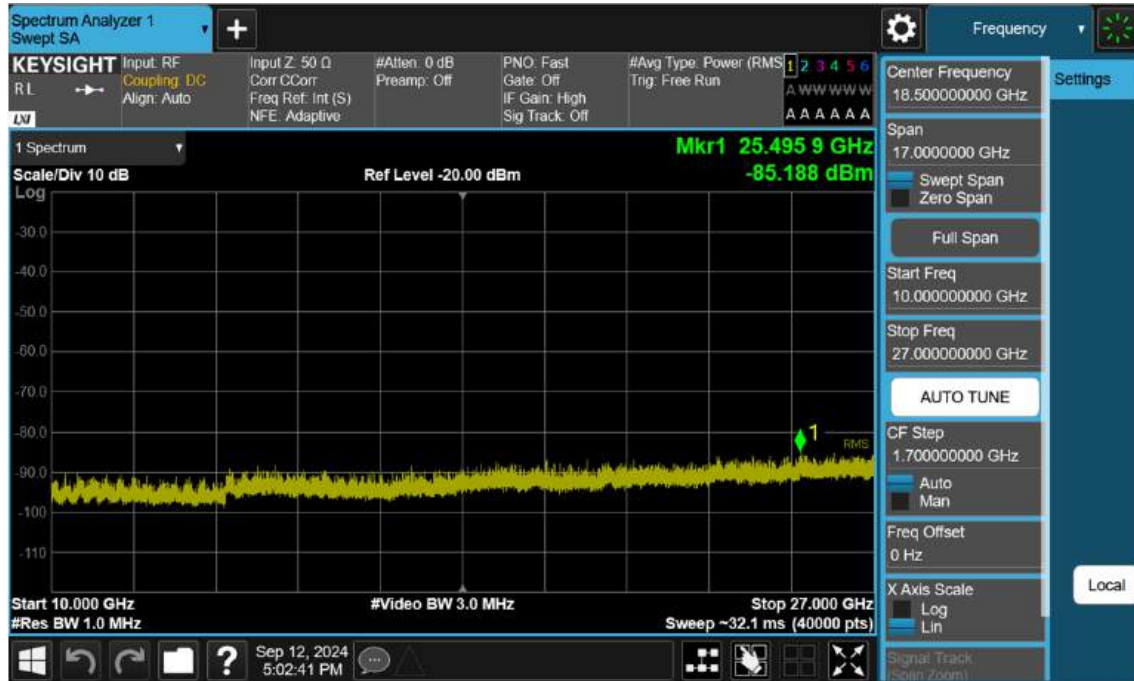
NR41_60 M_Conducted Spurious(Above10 G)_High_BPSK_1RB
