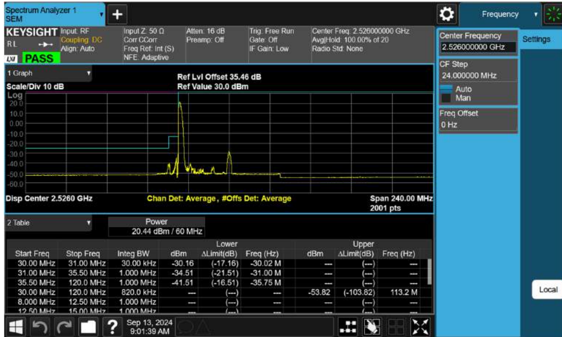
NR41_60 M_Channel Edge_Lower_Low_BPSK_1RB
