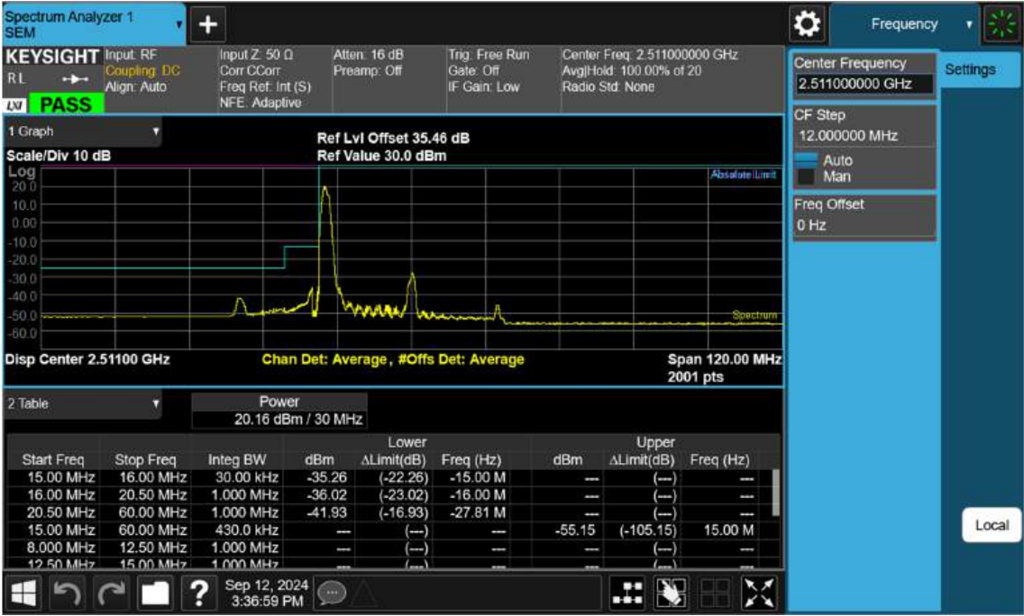
NR41_30 M_Channel Edge_Lower_Low_BPSK_1RB
