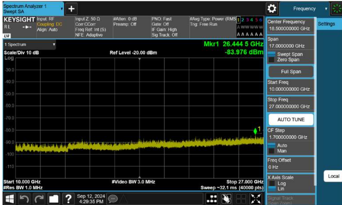
NR41_20 M_Conducted Spurious(Above10 G)_Mid_BPSK_1RB
