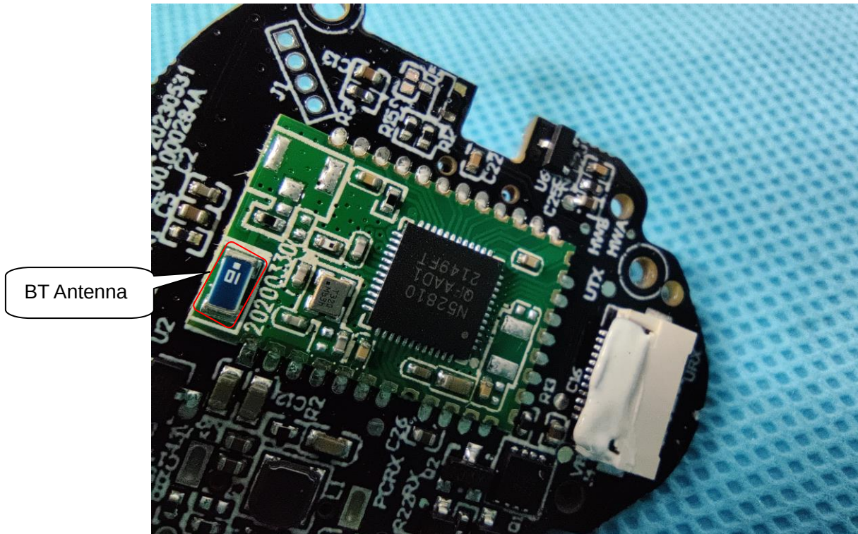
INTERNAL VIEW OF EUT (FIGURE 5)
