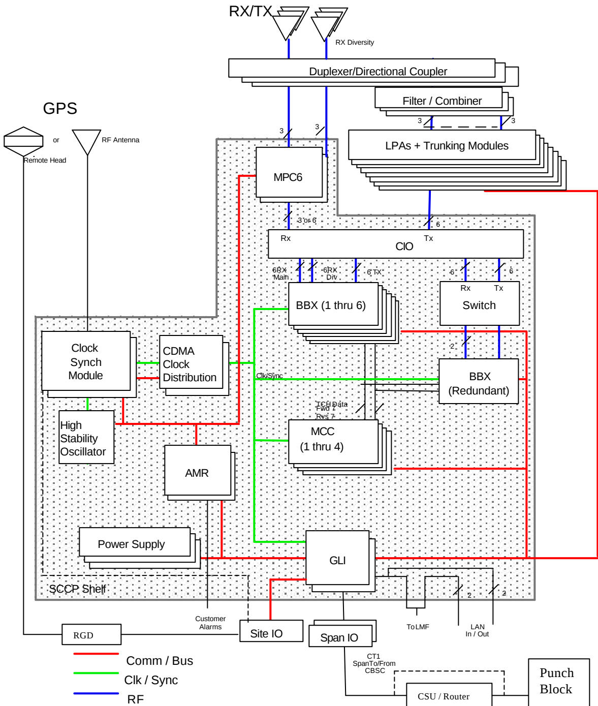
SC4812 T Lite Functional Block Diagram
