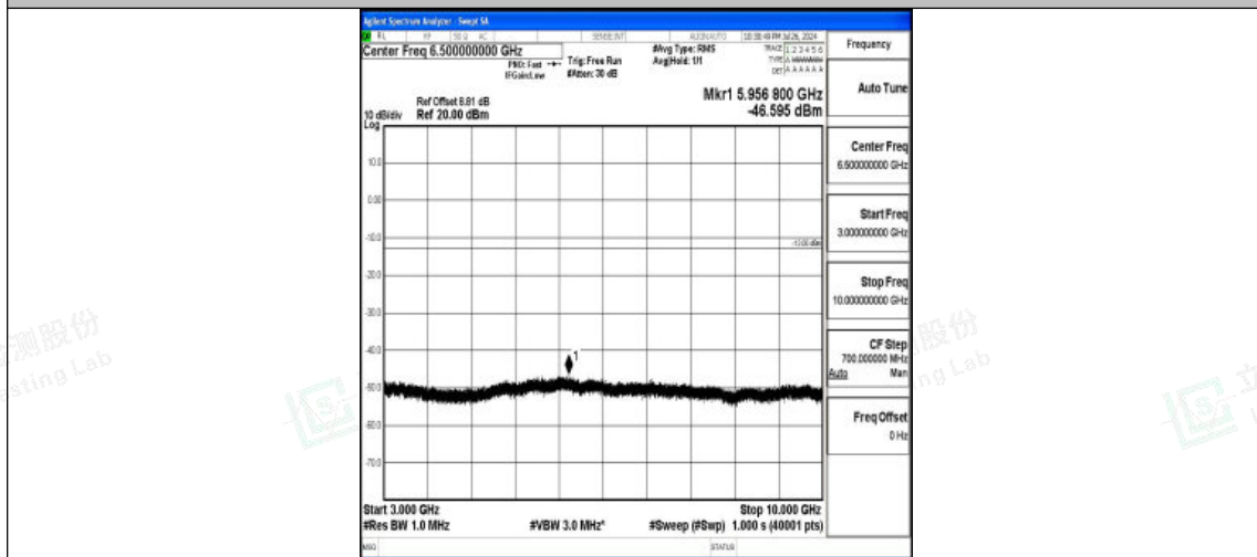
Band5-10MHz-QPSK-20450-1RB#0-3000~10000-PASS
