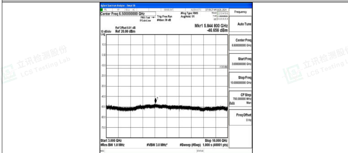
Band5-1.4MHz-16QAM-20643-1RB#0-3000~10000-PASS
