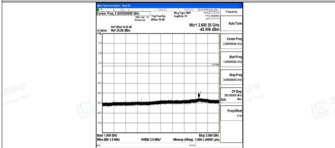
Band5-3MHz-QPSK-20525-1RB#0-1000~3000-PASS
