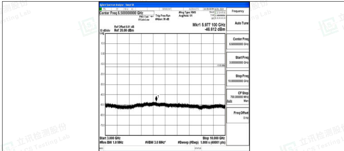
Band5-10MHz-QPSK-20600-1RB#0-3000~10000-PASS
