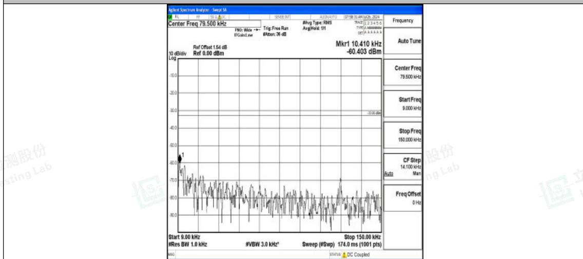
Band5-1.4MHz-16QAM-20643-1RB#0-0.009~0.15-PASS
