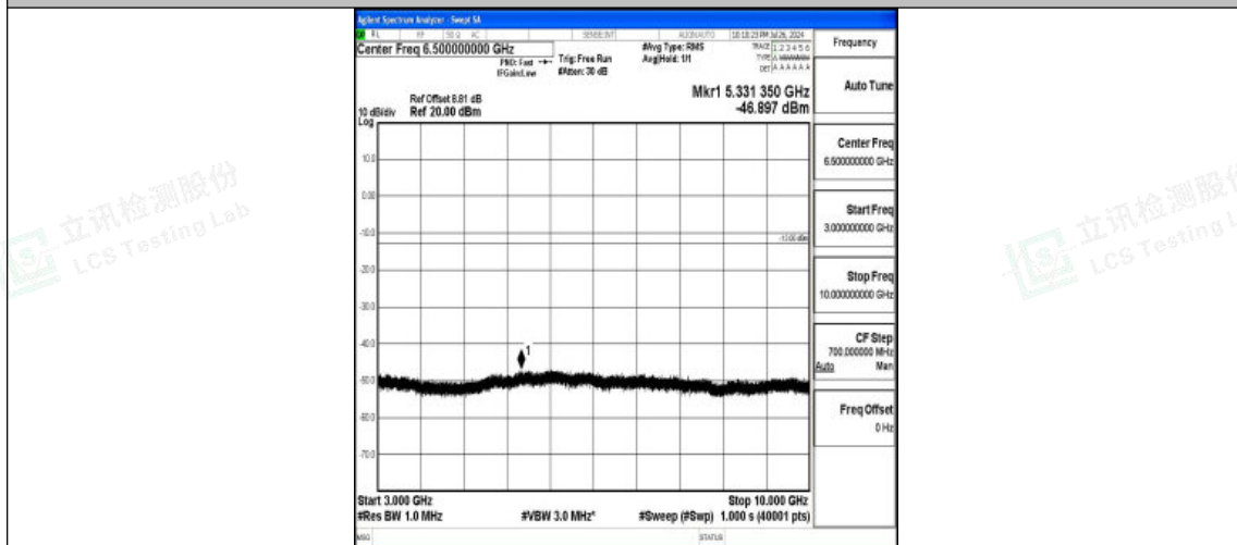
Band5-5MHz-QPSK-20525-1RB#0-3000~10000-PASS
