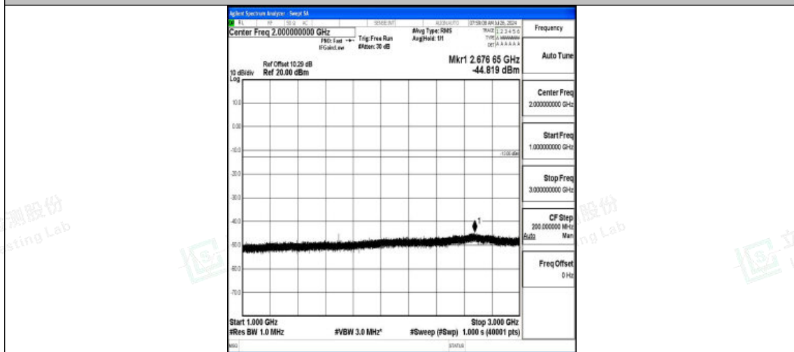
Band5-1.4MHz-16QAM-20643-1RB#0-1000~3000-PASS
