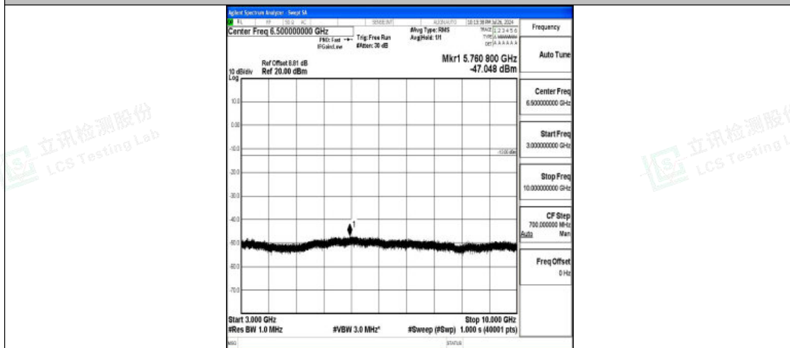
Band5-5MHz-16QAM-20625-1RB#0-3000~10000-PASS
