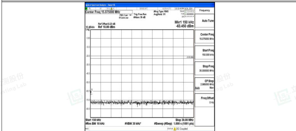
Band5-5MHz-16QAM-20525-1RB#0-0.15~30-PASS
