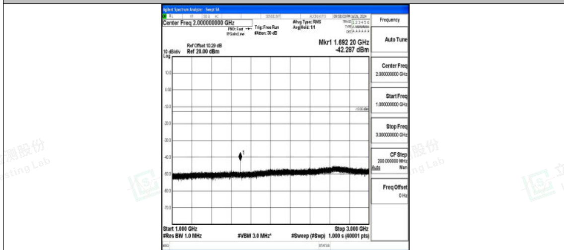
Band5-3MHz-16QAM-20635-1RB#0-1000~3000-PASS
