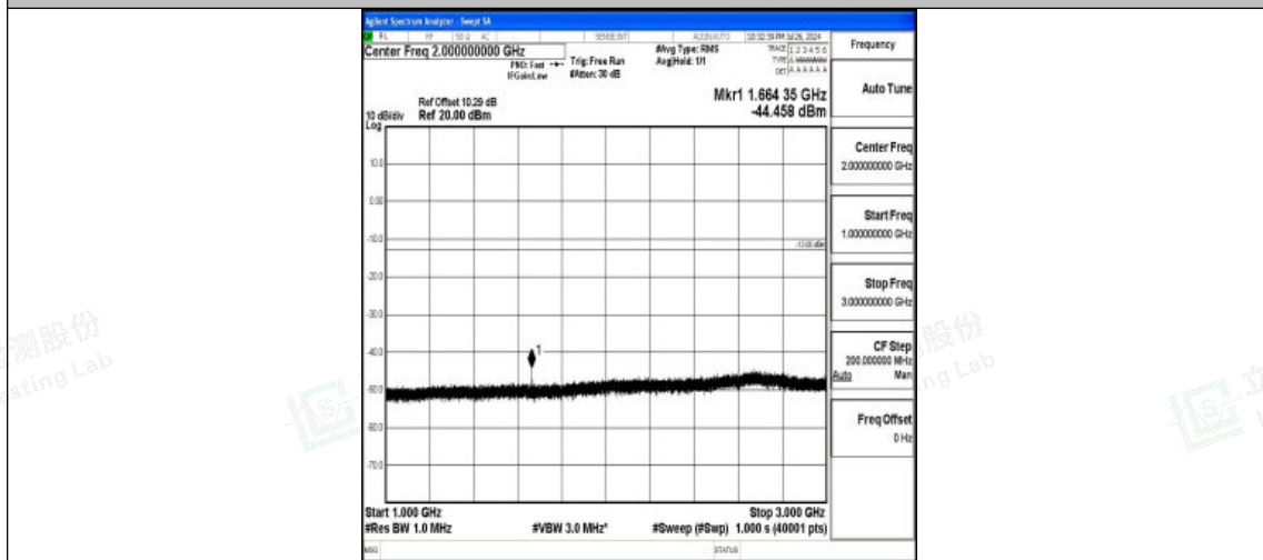
Band5-10MHz-QPSK-20525-1RB#0-1000~3000-PASS
