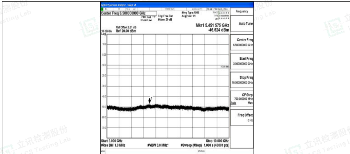
Band5-3MHz-QPSK-20635-1RB#0-3000~10000-PASS
