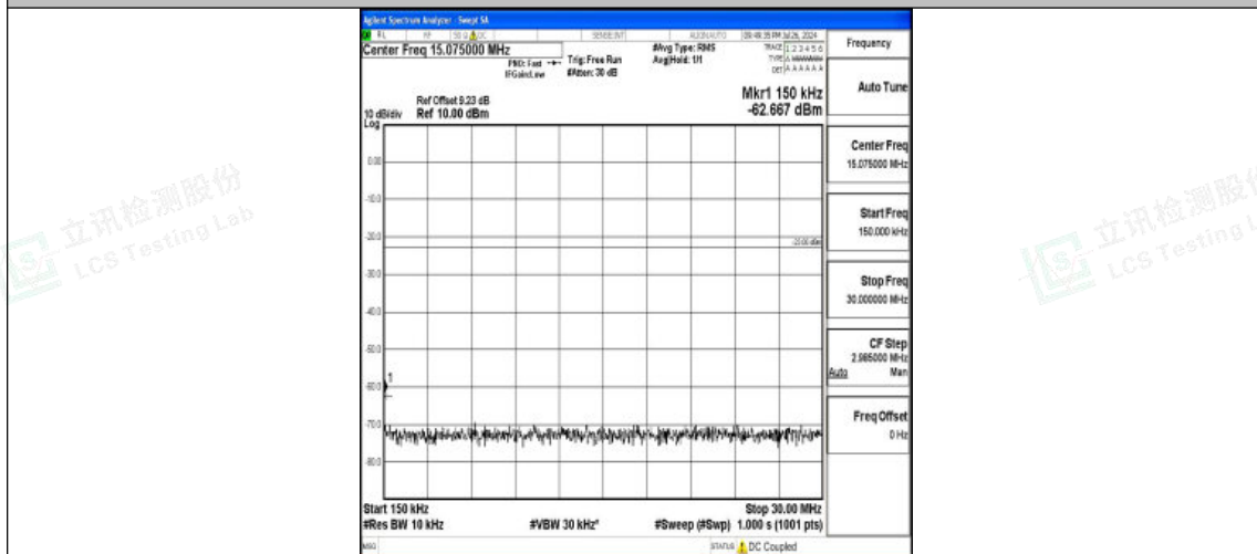
Band5-3MHz-16QAM-20635-1RB#0-0.15~30-PASS
