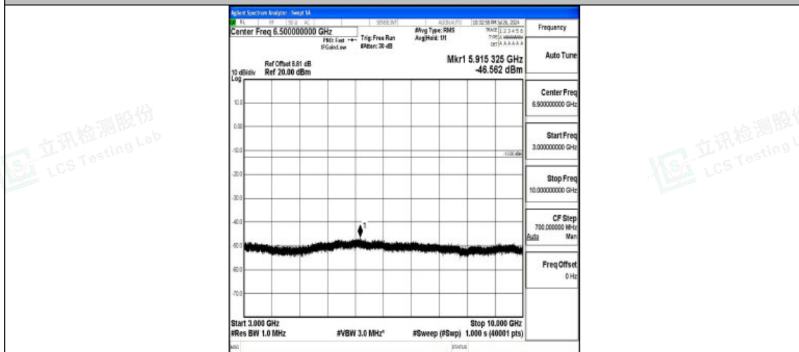
Band5-10MHz-QPSK-20525-1RB#0-3000~10000-PASS
