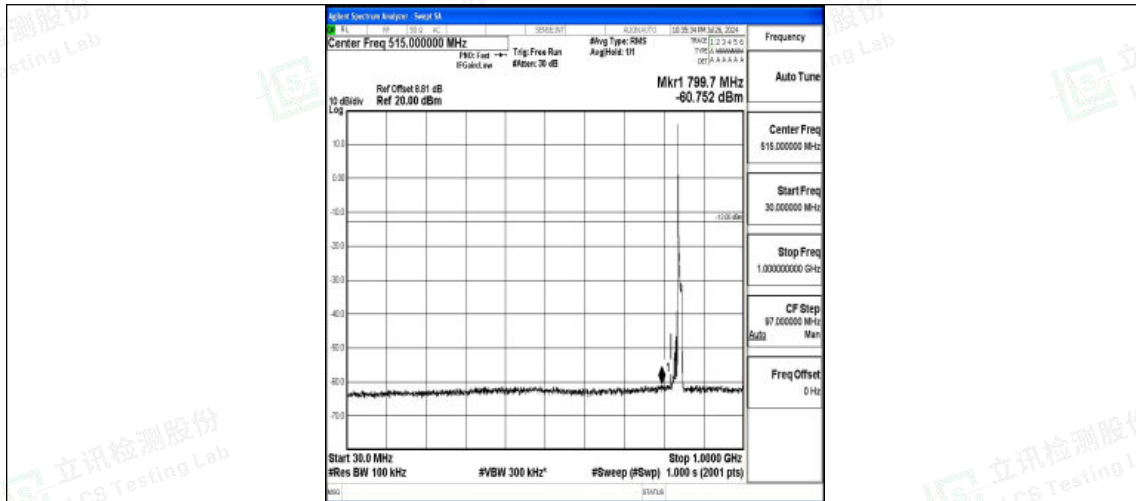
Band5-10MHz-16QAM-20600-1RB#0-30~1000-PASS
