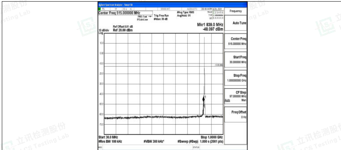
Band5-3MHz-16QAM-20635-1RB#0-30~1000-PASS
