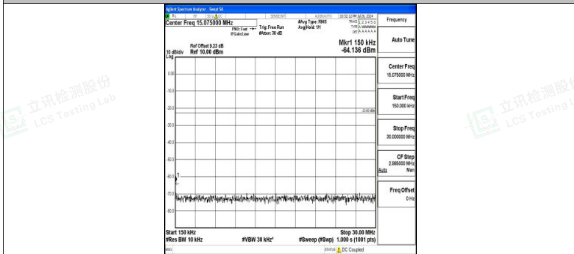
Band5-10MHz-QPSK-20525-1RB#0-0.15~30-PASS
