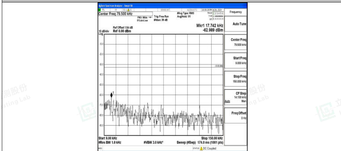
Band5-5MHz-QPSK-20525-1RB#0-0.009~0.15-PASS
