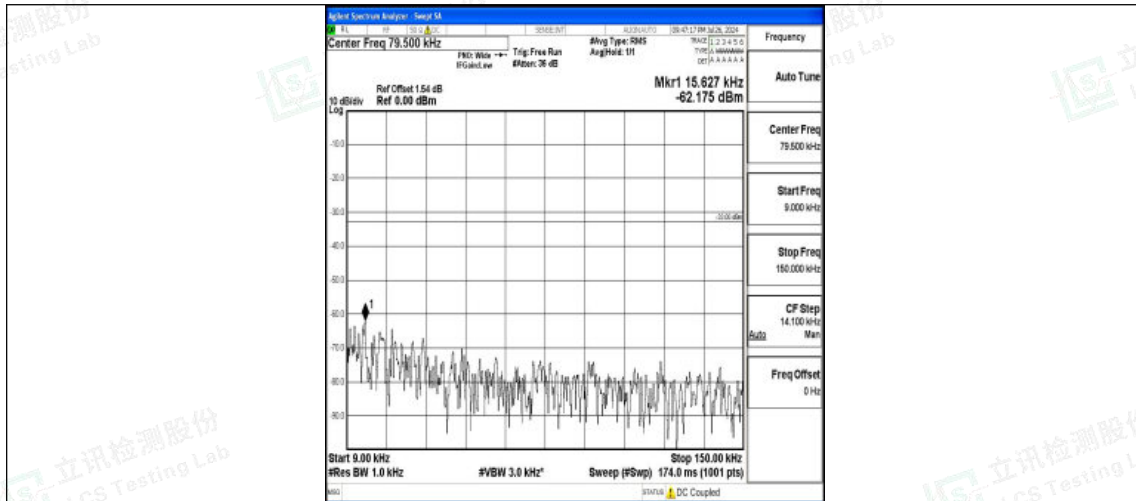
Band5-3MHz-16QAM-20525-1RB#0-0.009~0.15-PASS
