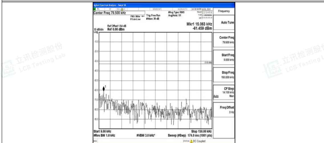
Band5-10MHz-16QAM-20450-1RB#0-0.009~0.15-PASS
