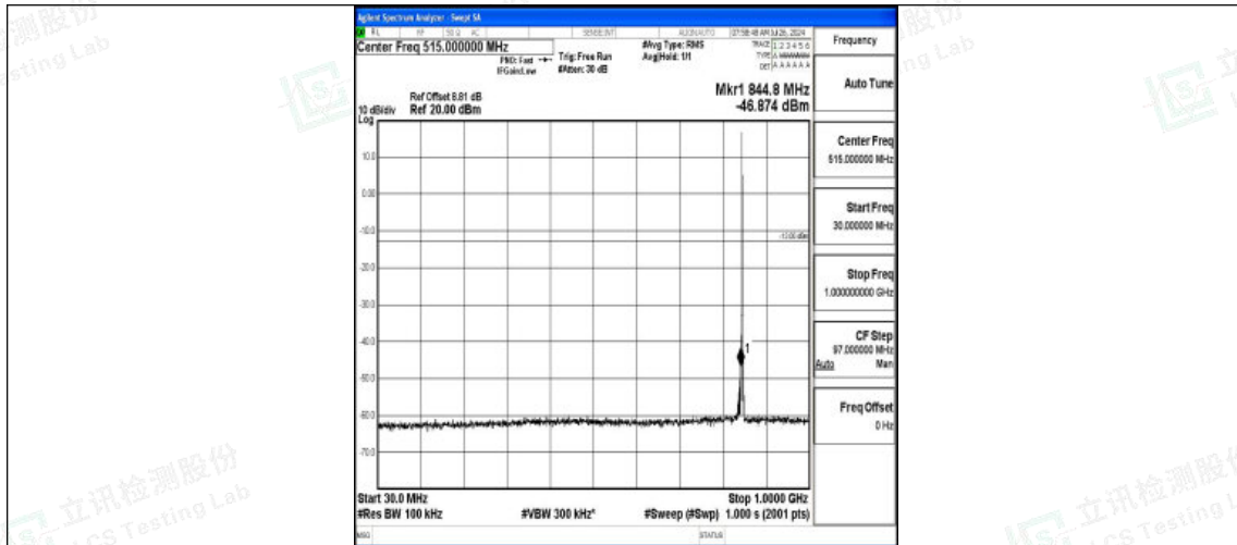
Band5-1.4MHz-16QAM-20643-1RB#0-30~1000-PASS
