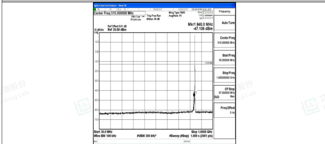
Band5-3MHz-QPSK-20635-1RB#0-30~1000-PASS
