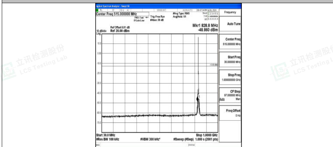
Band5-3MHz-16QAM-20525-1RB#0-30~1000-PASS
