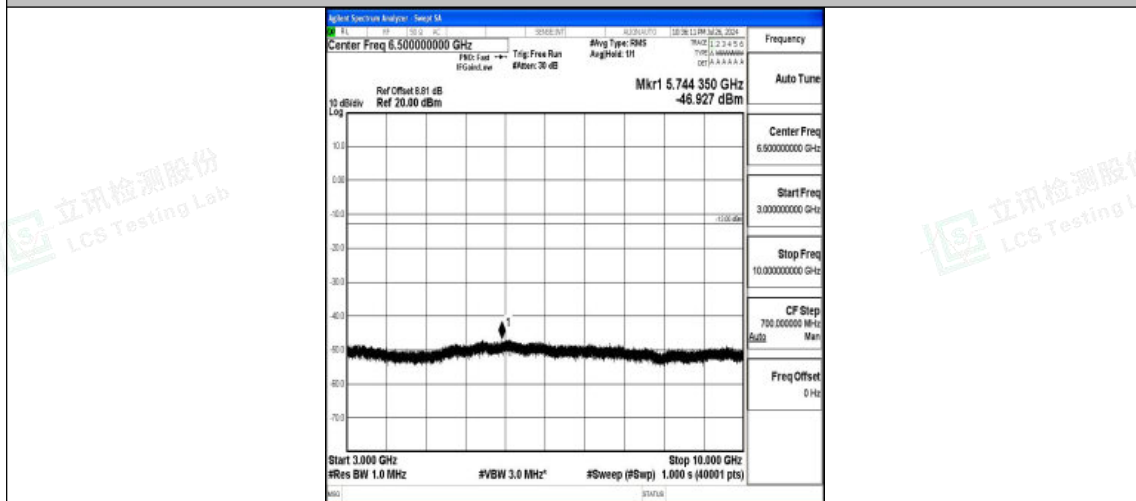
Band5-10MHz-16QAM-20600-1RB#0-3000~10000-PASS
