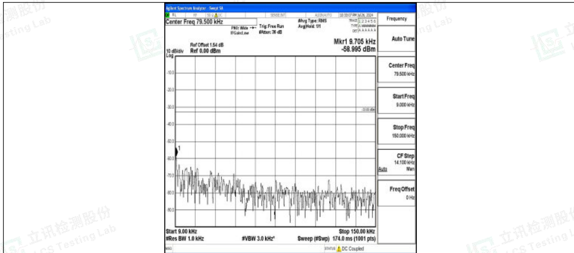
Band5-10MHz-16QAM-20525-1RB#0-0.009~0.15-PASS
