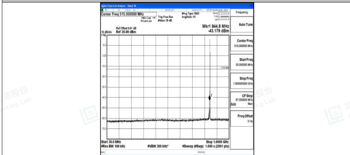
Band5-1.4MHz-QPSK-20643-1RB#0-30~1000-PASS
