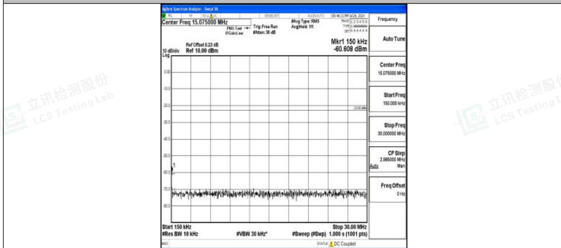
Band5-3MHz-QPSK-20525-1RB#0-0.15~30-PASS
