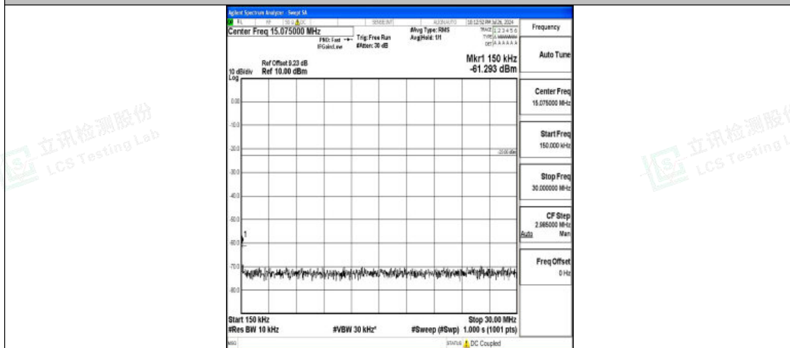
Band5-5MHz-16QAM-20625-1RB#0-0.15~30-PASS
