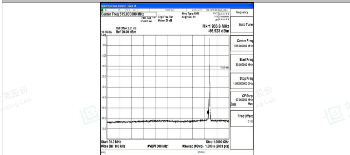
Band5-5MHz-QPSK-20625-1RB#0-30~1000-PASS
