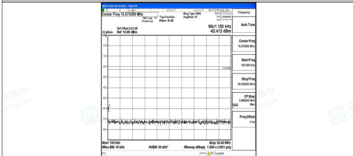
Band5-3MHz-16QAM-20525-1RB#0-0.15~30-PASS
