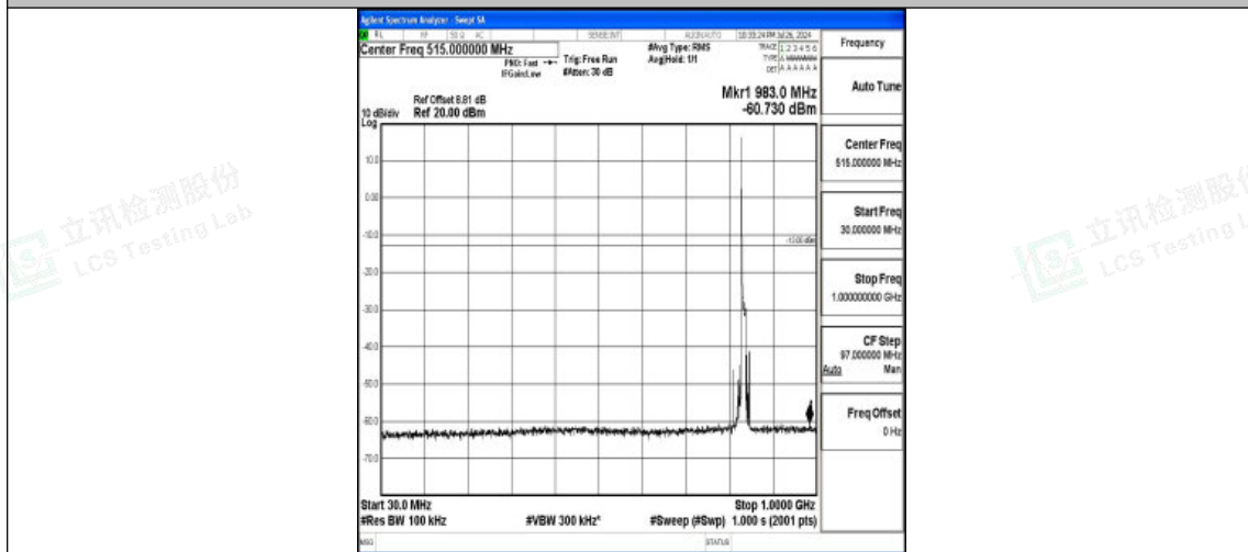
Band5-10MHz-16QAM-20525-1RB#0-30~1000-PASS
