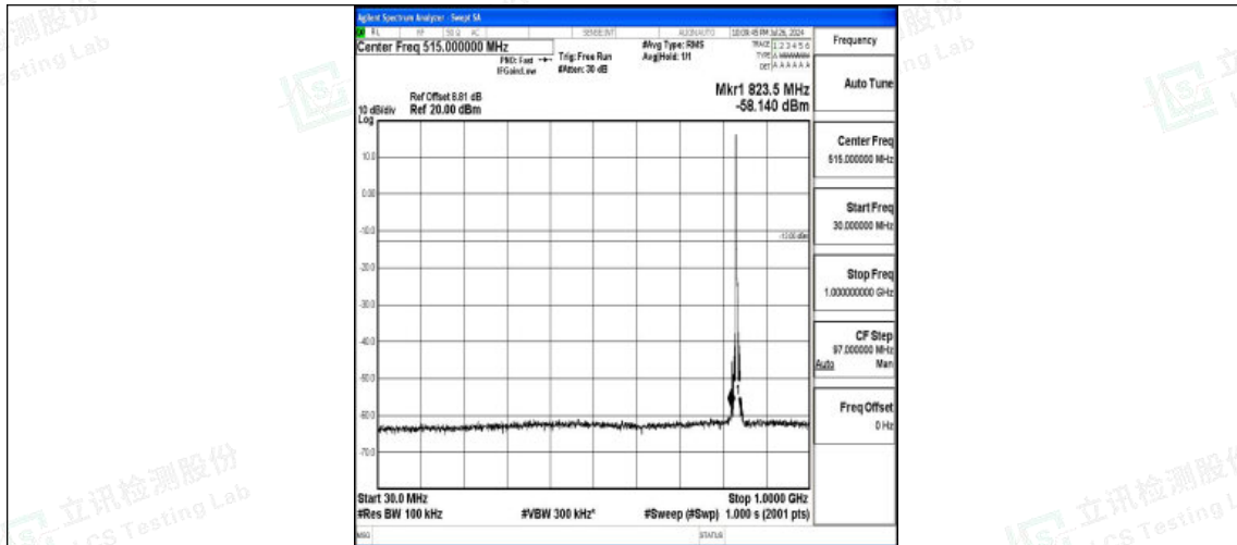
Band5-5MHz-QPSK-20525-1RB#0-30~1000-PASS
