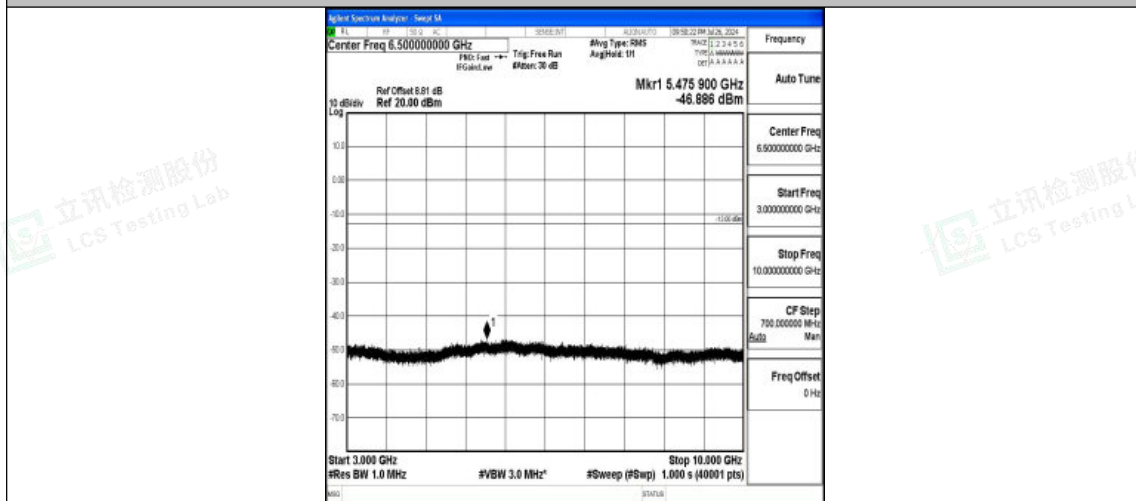
Band5-3MHz-16QAM-20635-1RB#0-3000~10000-PASS
