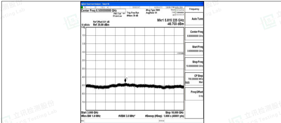
Band5-5MHz-16QAM-20425-1RB#0-3000~10000-PASS
