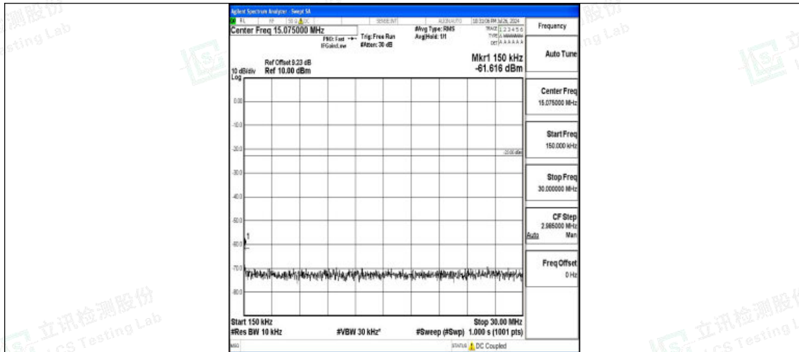
Band5-10MHz-16QAM-20450-1RB#0-0.15~30-PASS
