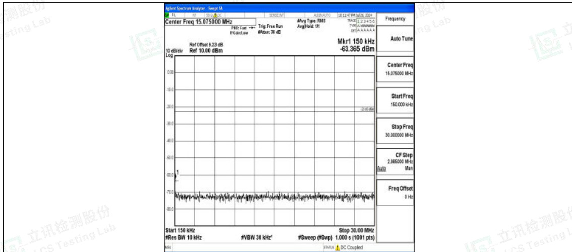
Band5-5MHz-QPSK-20625-1RB#0-0.15~30-PASS
