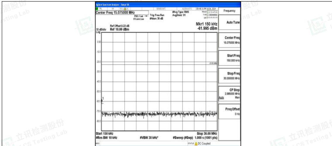
Band5-3MHz-QPSK-20635-1RB#0-0.15~30-PASS
