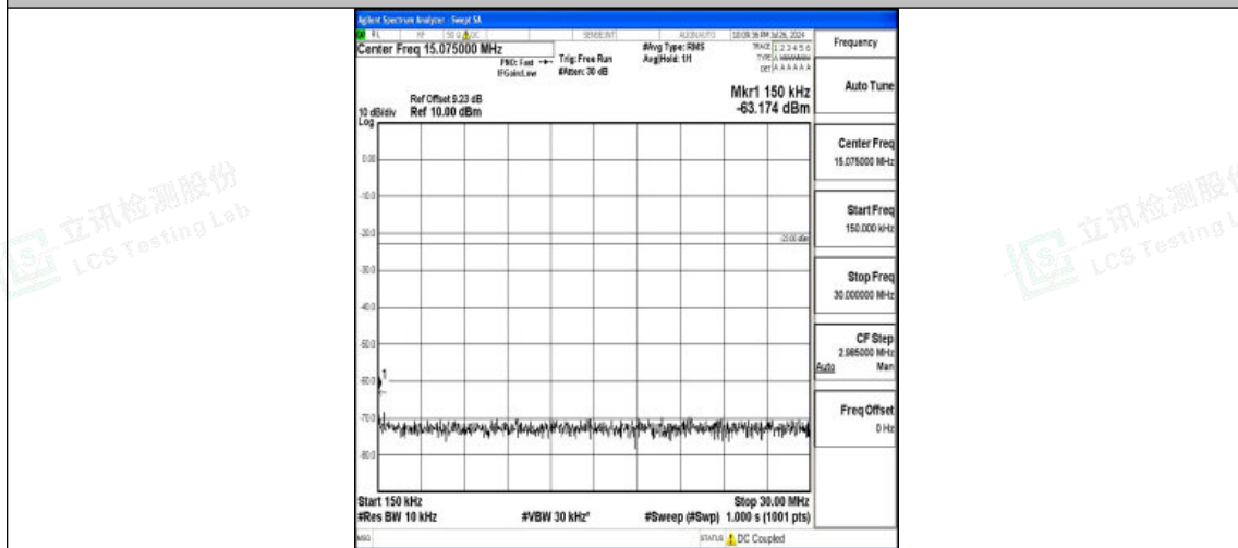
Band5-5MHz-QPSK-20525-1RB#0-0.15~30-PASS
