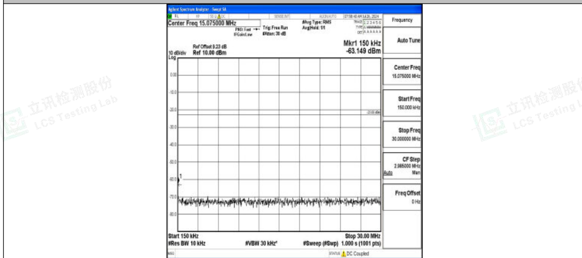
Band5-1.4MHz-16QAM-20643-1RB#0-0.15~30-PASS
