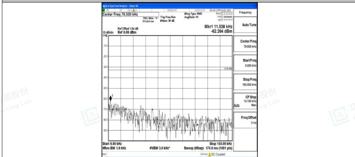
Band5-3MHz-QPSK-20525-1RB#0-0.009~0.15-PASS
