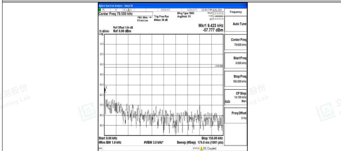
Band5-10MHz-16QAM-20600-1RB#0-0.009~0.15-PASS
