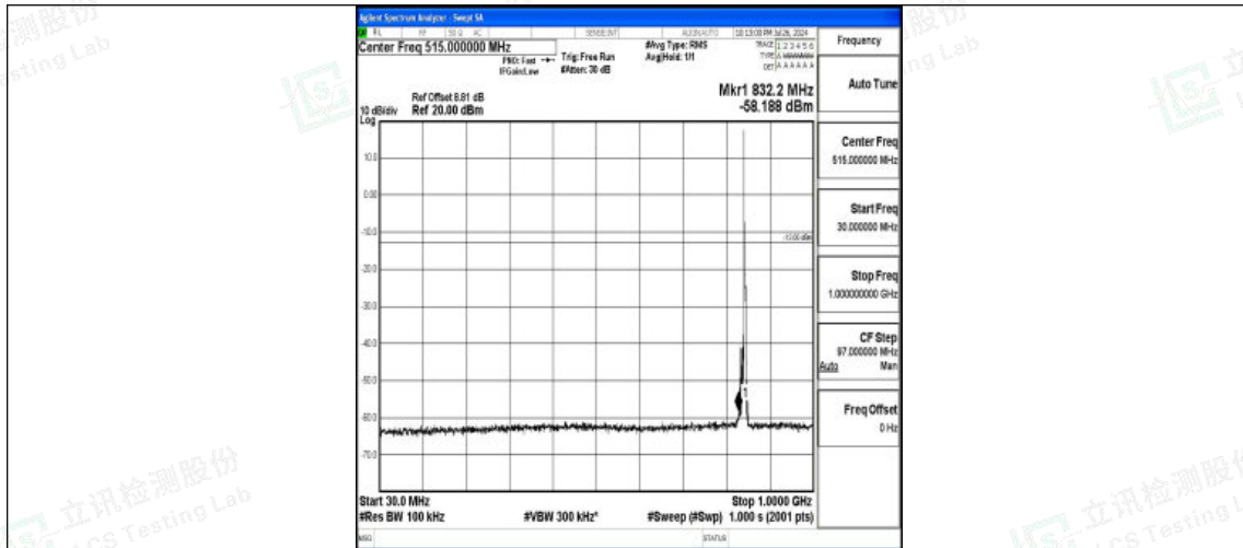
Band5-5MHz-16QAM-20625-1RB#0-30~1000-PASS
