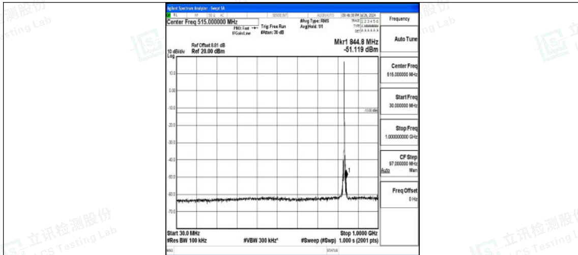
Band5-3MHz-QPSK-20525-1RB#0-30~1000-PASS
