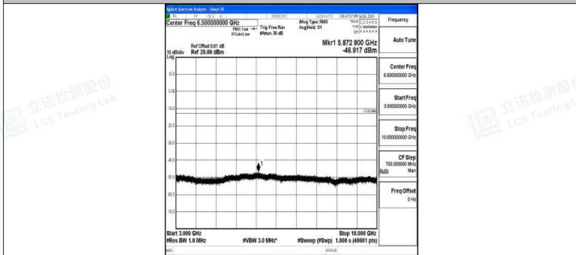
Band5-3MHz-QPSK-20525-1RB#0-3000~10000-PASS
