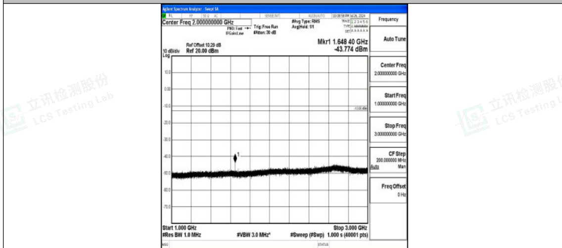
Band5-5MHz-16QAM-20425-1RB#0-1000~3000-PASS
