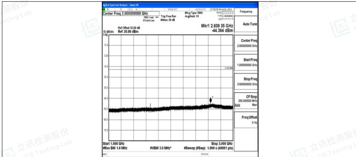
Band5-1.4MHz-16QAM-20525-1RB#0-1000~3000-PASS
