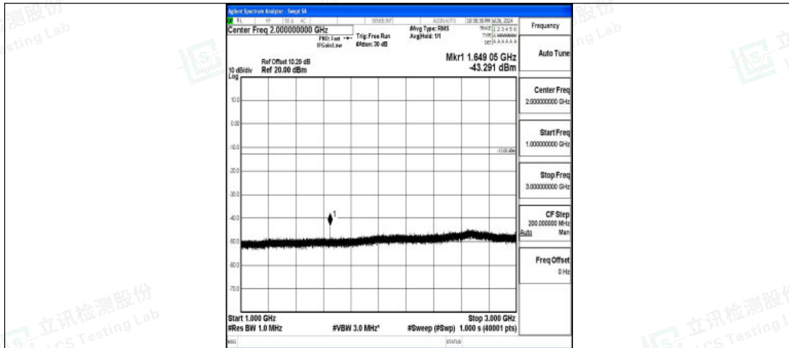
Band5-10MHz-QPSK-20450-1RB#0-1000~3000-PASS
