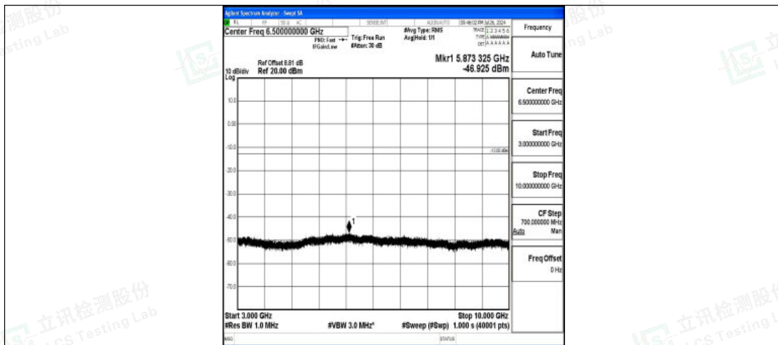
Band5-3MHz-16QAM-20415-1RB#0-3000~10000-PASS
