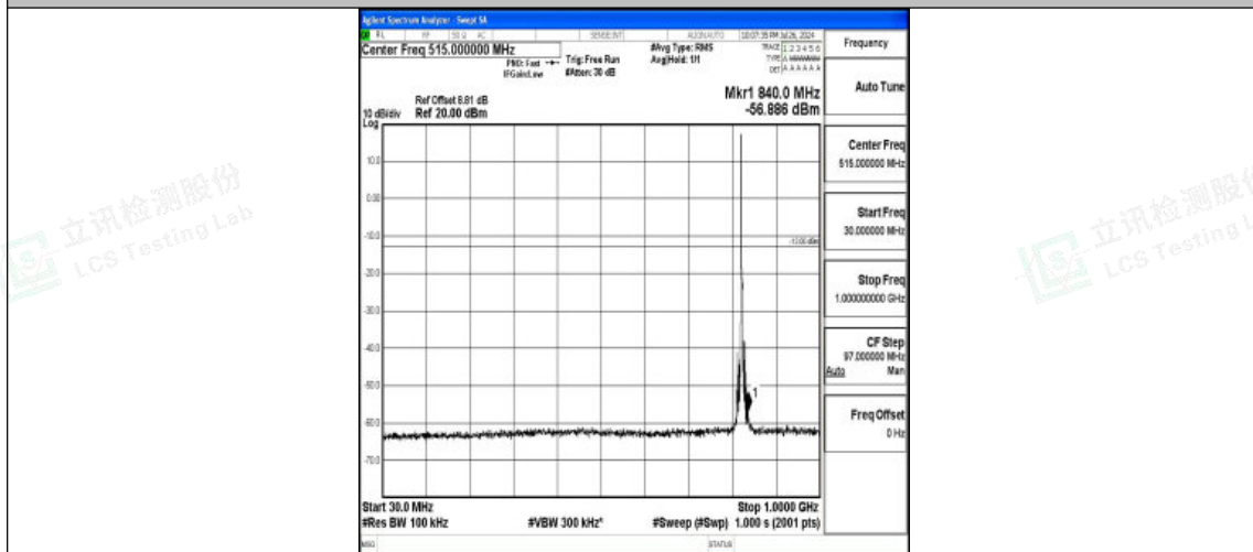
Band5-5MHz-QPSK-20425-1RB#0-30~1000-PASS
