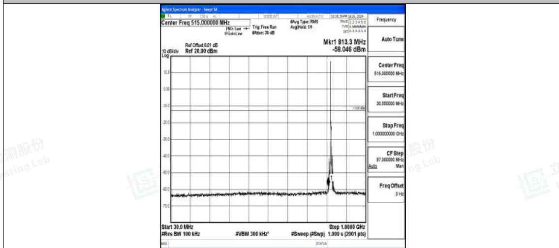
Band5-5MHz-16QAM-20425-1RB#0-30~1000-PASS
