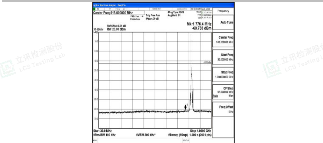
Band5-10MHz-QPSK-20450-1RB#0-30~1000-PASS
