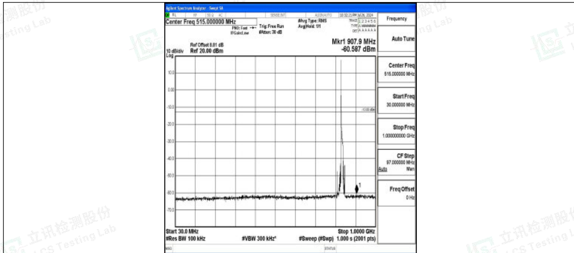
Band5-10MHz-QPSK-20525-1RB#0-30~1000-PASS
