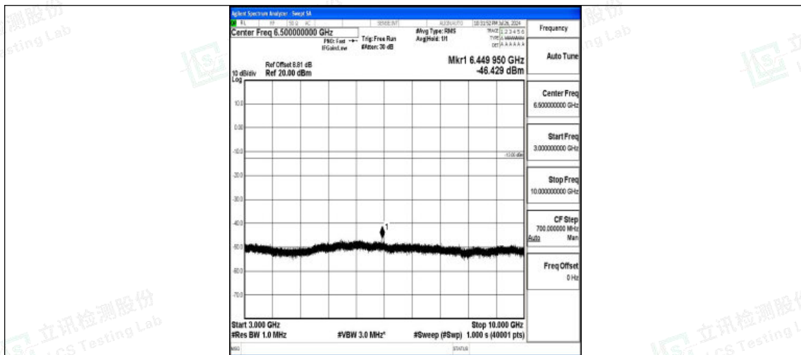
Band5-10MHz-16QAM-20450-1RB#0-3000~10000-PASS
