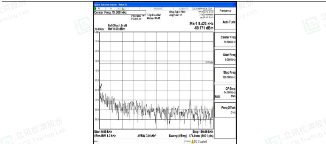
Band5-10MHz-QPSK-20450-1RB#0-0.009~0.15-PASS
