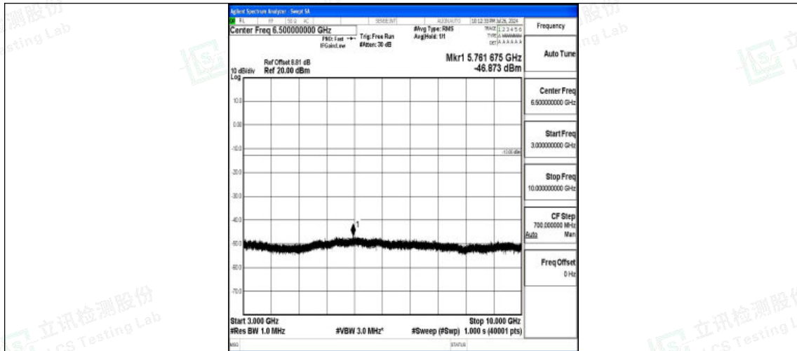
Band5-5MHz-QPSK-20625-1RB#0-3000~10000-PASS
