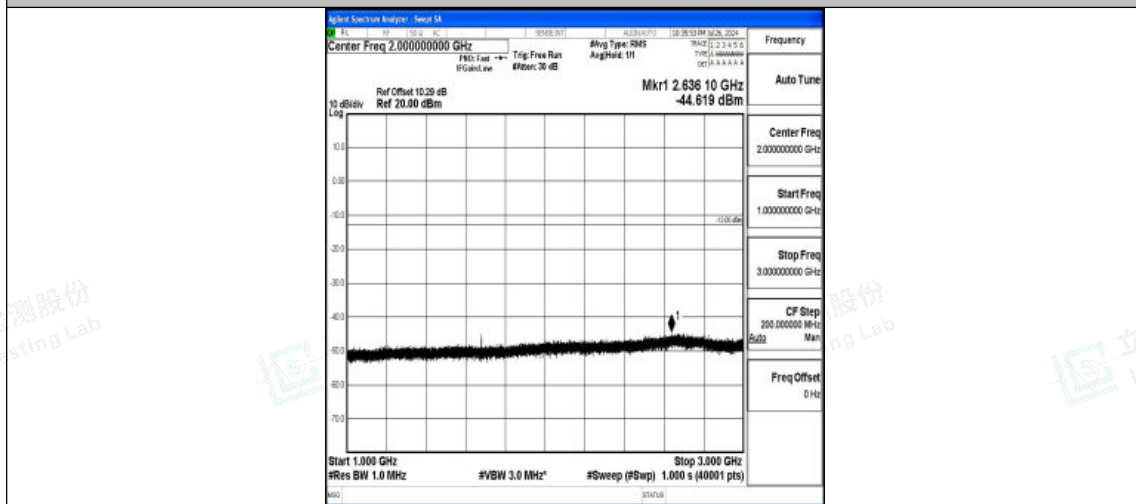
Band5-10MHz-16QAM-20600-1RB#0-1000~3000-PASS
