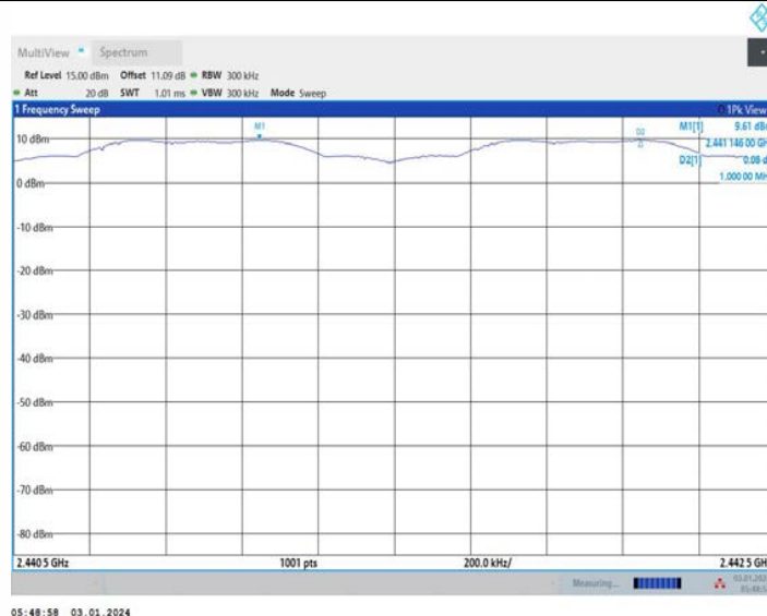
2DH5_Ant1_Hop_2441
