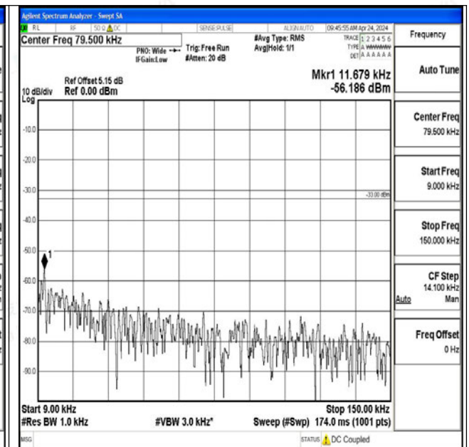
Band12_10MHz_16QAM_23095_1RB#0_0.009~0.15_0. 009~0.15
