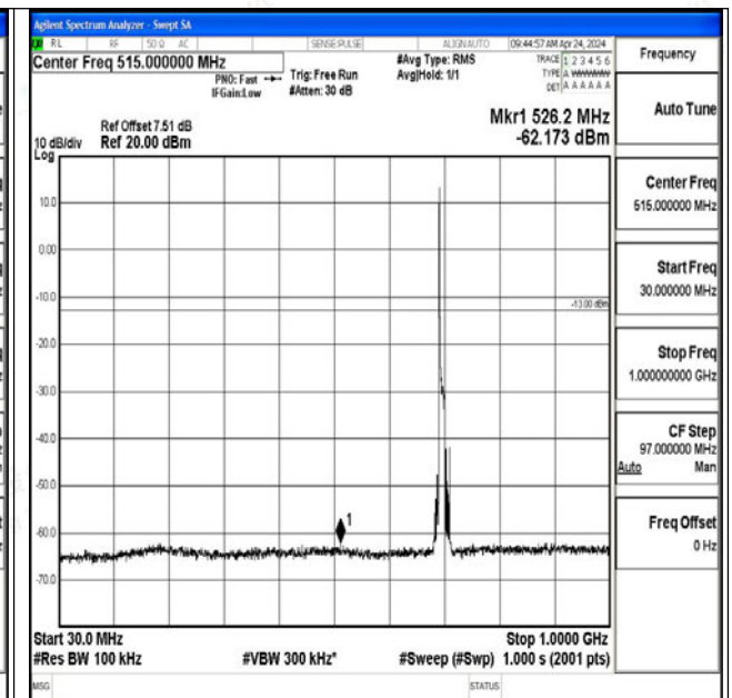
Band12_10MHz_16QAM_23060_1RB#0_30~1000_30~1000
