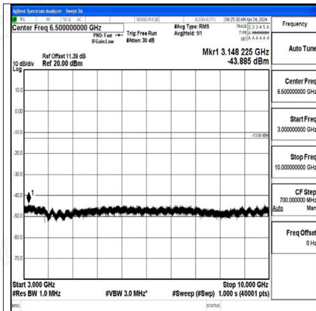
Band12_5MHz_QPSK_23155_1RB#0_3000~10000_300 0~10000
