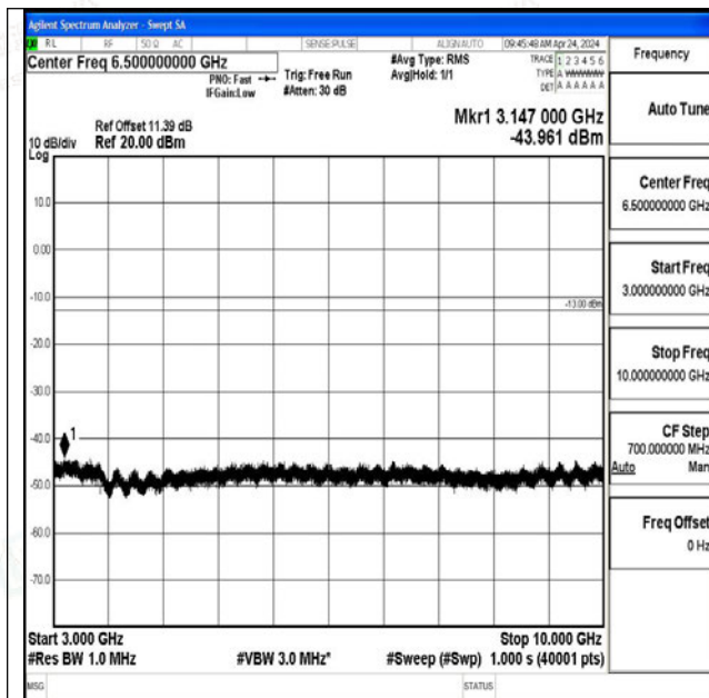
Band12_10MHz_QPSK_23095_1RB#0_3000~10000_30 00~10000
