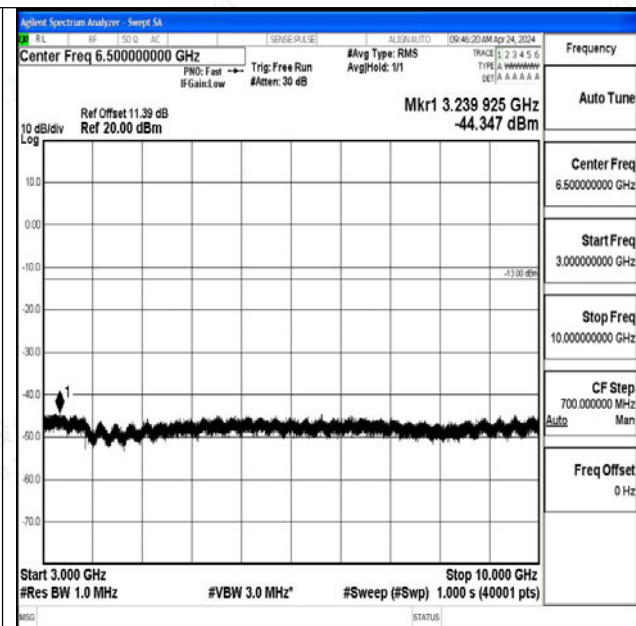
Band12_10MHz_16QAM_23095_1RB#0_3000~10000_3 000~10000
