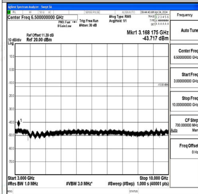
Band12_10MHz_QPSK_23060_1RB#0_3000~10000_3000~10000
