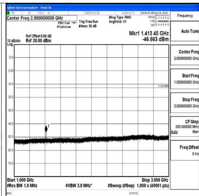
Band12_10MHz_QPSK_23130_1RB#0_1000~3000_1000~3000
