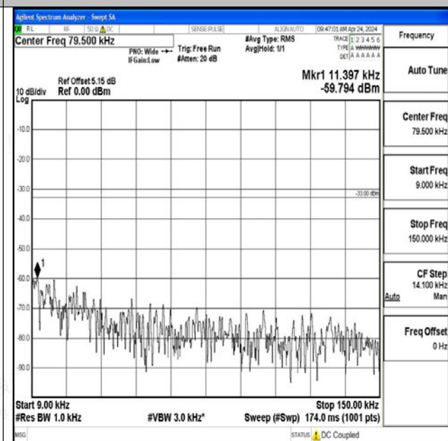
Band12_10MHz_16QAM_23130_1RB#0_0.009~0.15_0.009~0.15
