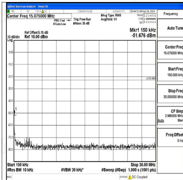
Band12_10MHz_16QAM_23060_1RB#0_0.15~30_0.15~30
