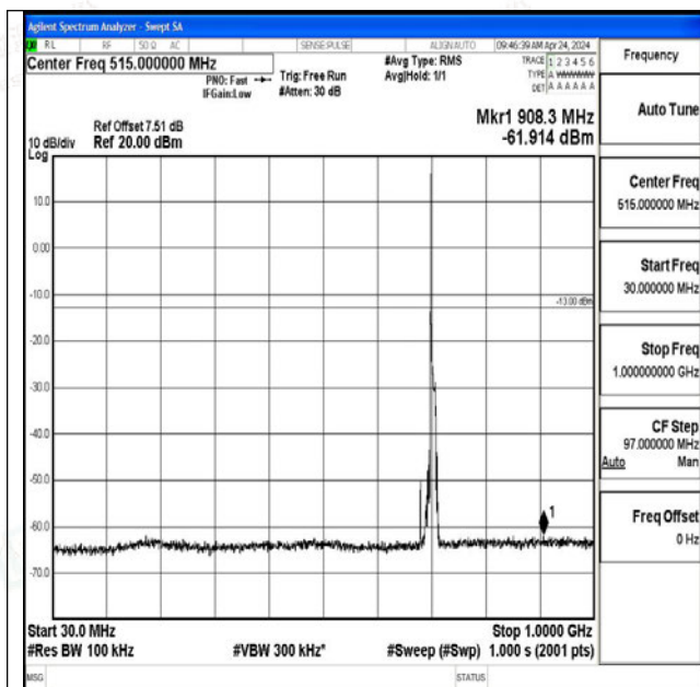
Band12_10MHz_QPSK_23130_1RB#0_30~1000_30~1000
