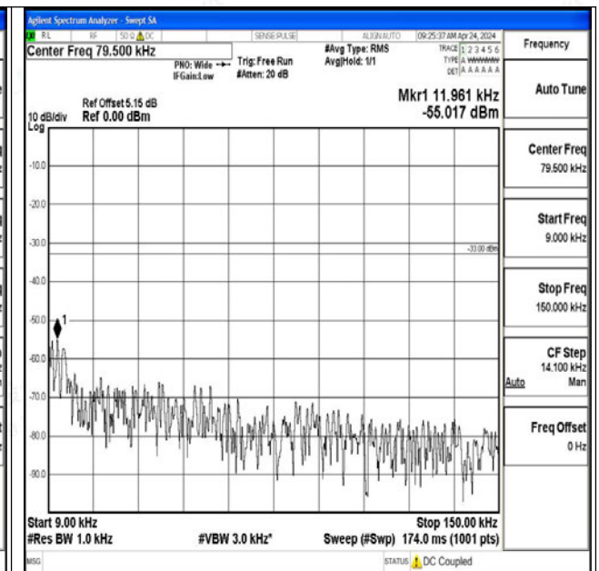
Band12_5MHz_16QAM_23155_1RB#0_0.009~0.15_0.0 09~0.15
