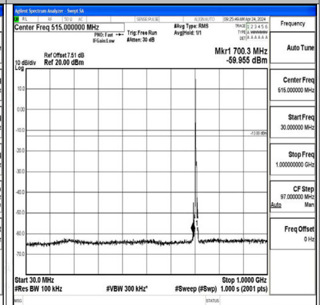
Band12_5MHz_16QAM_23155_1RB#0_30~1000_30~10 00
