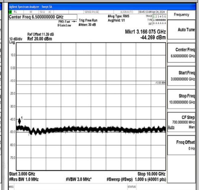
Band12_10MHz_16QAM_23060_1RB#0_3000~10000_3000~10000
