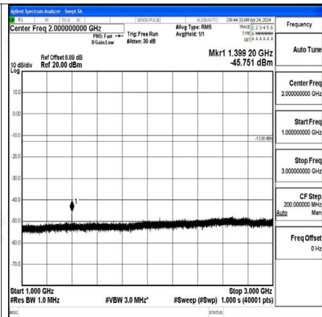
Band12_10MHz_QPSK_23060_1RB#0_1000~3000_1000~3000
