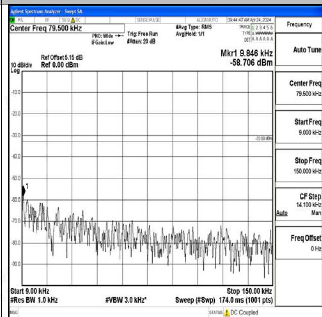
Band12_10MHz_16QAM_23060_1RB#0_0.009~0.15_0.009~0.15
