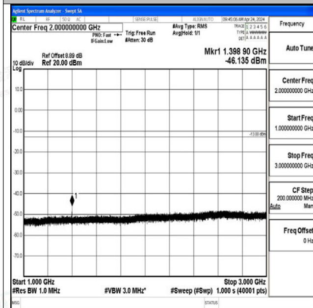
Band12_10MHz_16QAM_23060_1RB#0_1000~3000_1000~3000
