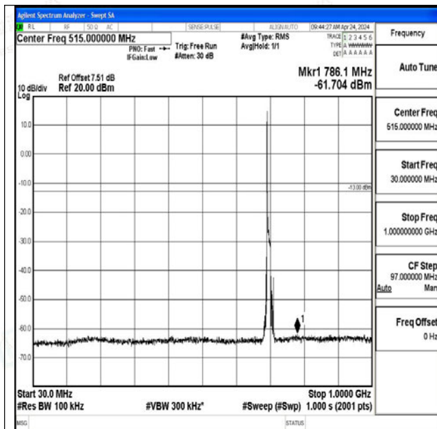
Band12_10MHz_QPSK_23060_1RB#0_30~1000_30~1000
