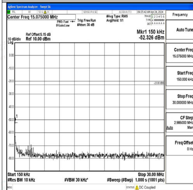
Band12_5MHz_16QAM_23155_1RB#0_0.15~30_0.15~3 0
