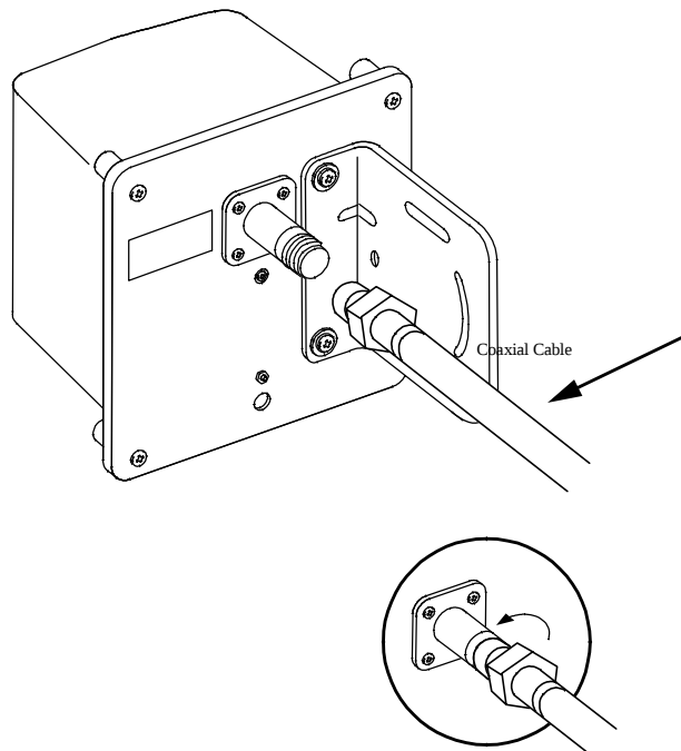
Figure 2-6 : Coaxial Cable Connection to Antenna
