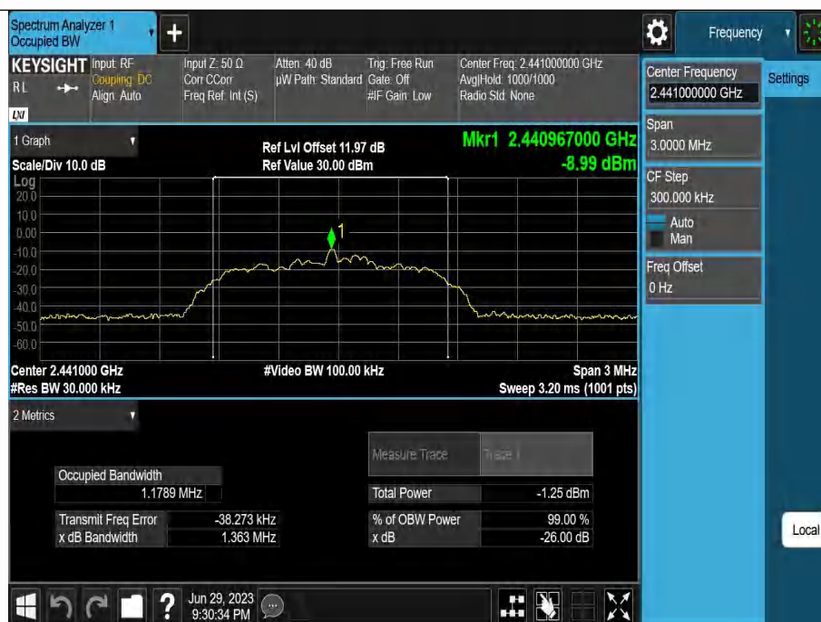
2DH5-Ant1-2441
