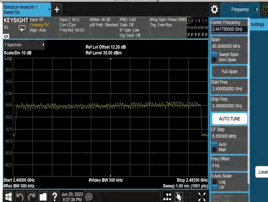
2DH5-Ant1-Hop
