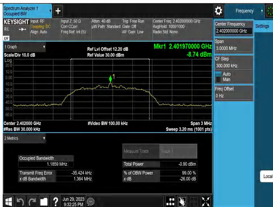
3DH5-Ant1-2402
