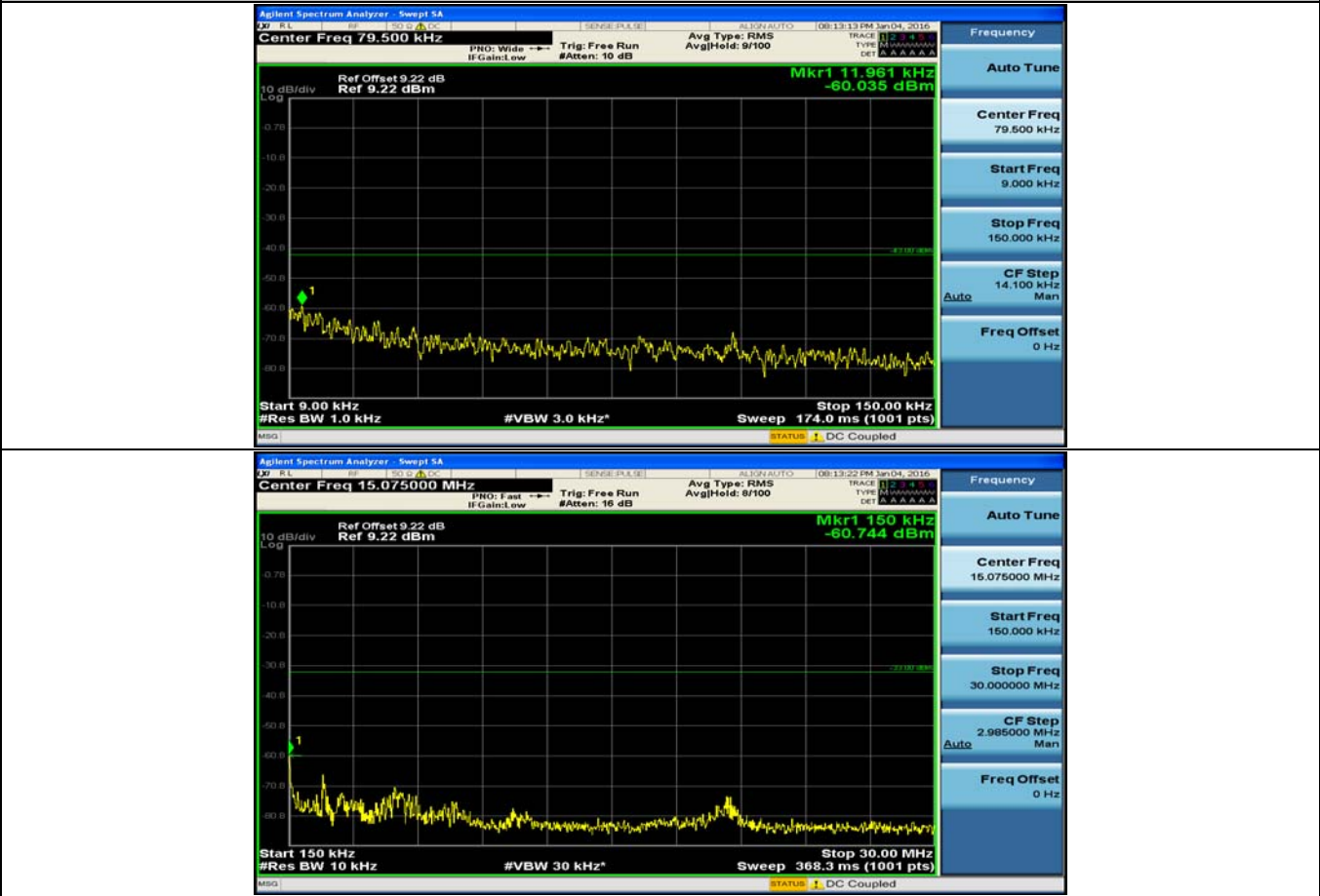
Channel Bandwidth: 10 MHz_HCH_16QAM_1RB#0
