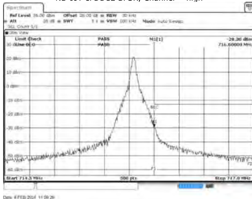
NB-IoT eFDD12 BPSK, Channel = high
