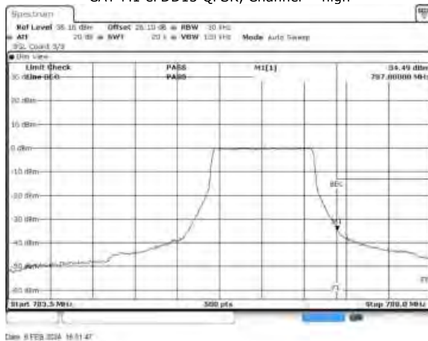
CAT-M1 eFDD13 QPSK, Channel = high
