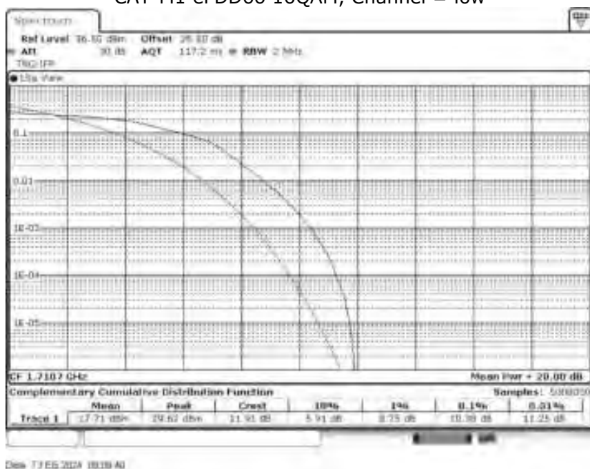
CAT-M1 eFDD66 16QAM, Channel = low
