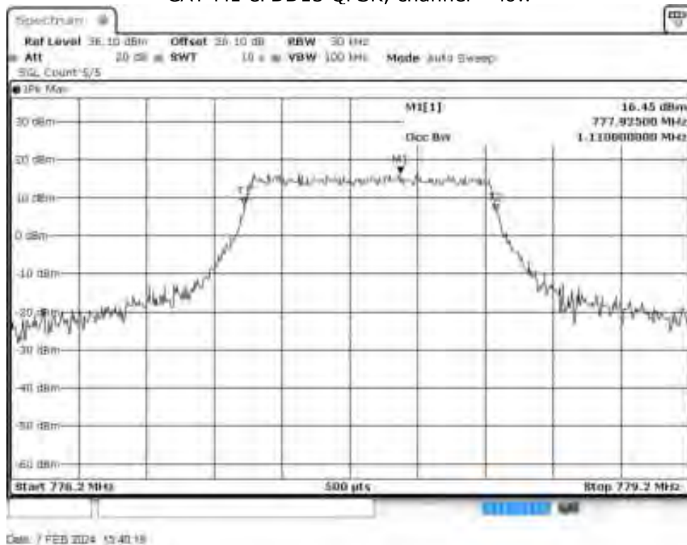
CAT-M1 eFDD13 QPSK, channel = low
