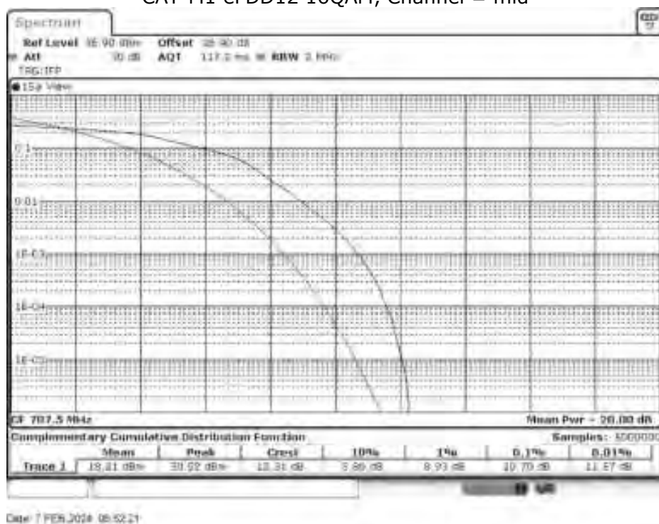
CAT-M1 eFDD12 16QAM, Channel = mid
