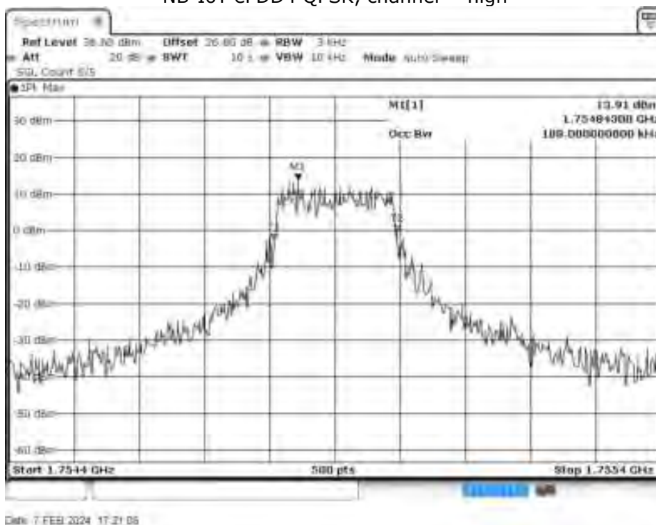
NB-IoT eFDD4 QPSK, channel = high
