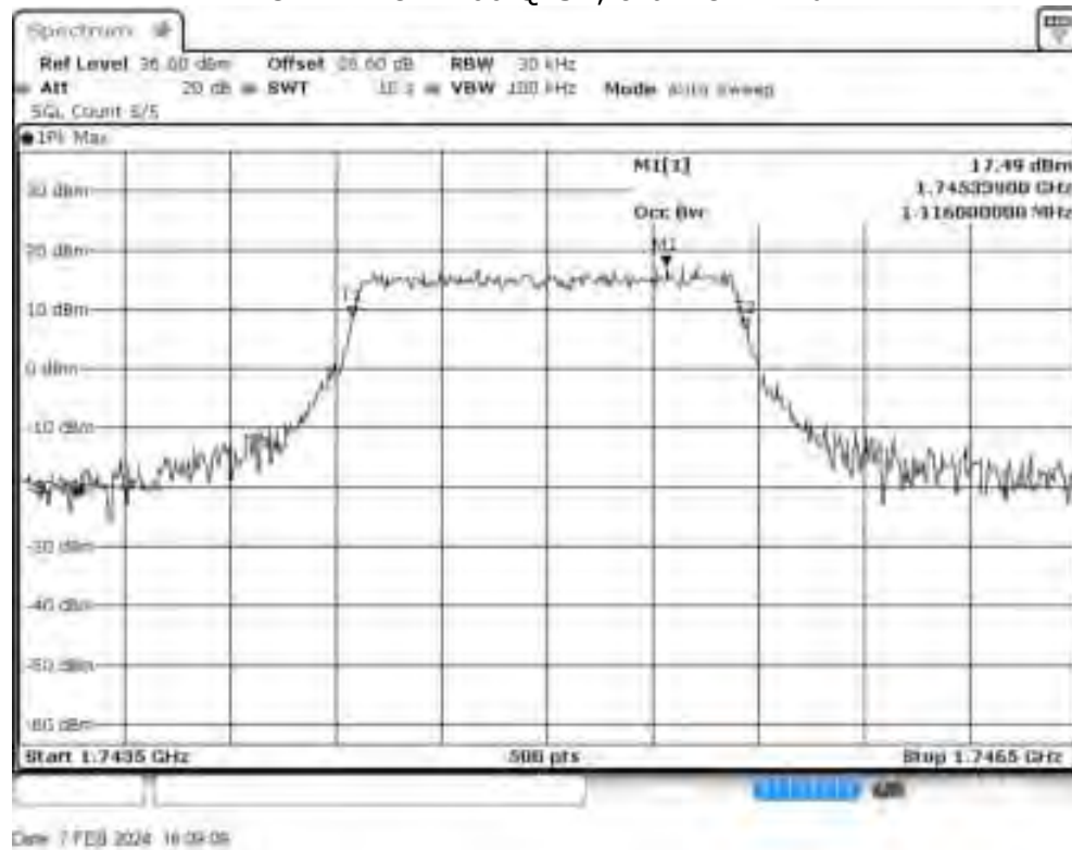
CAT-M1 eFDD66 QPSK, channel = mid
