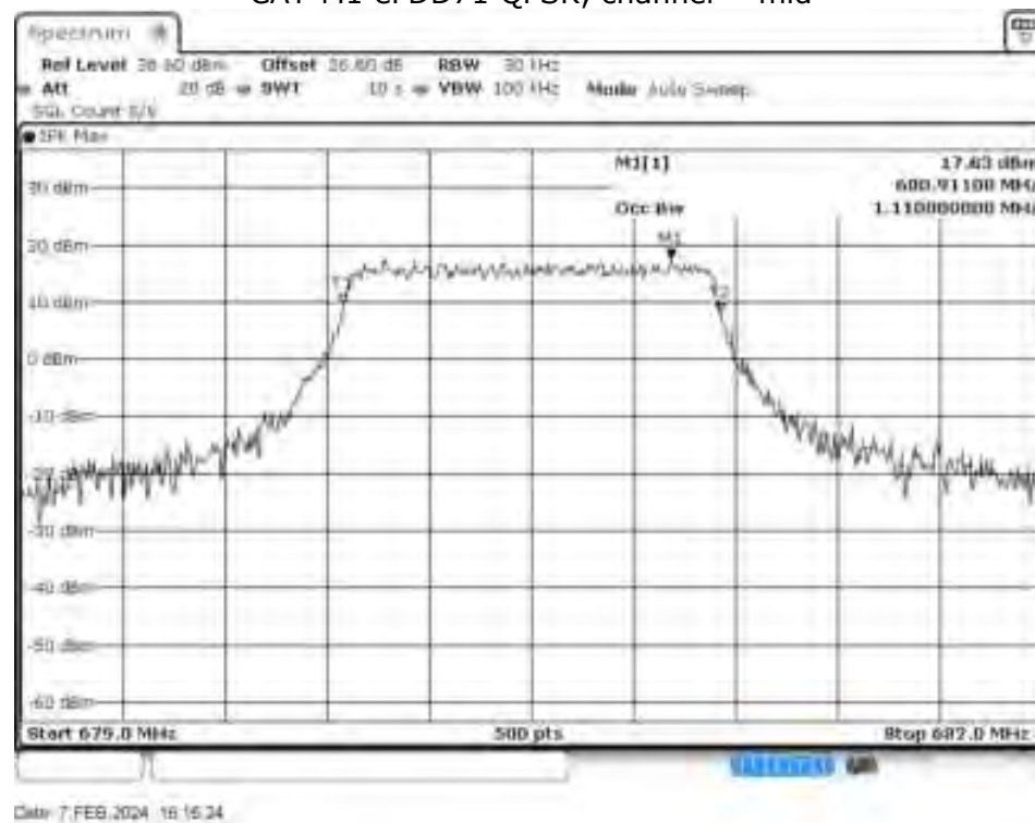
CAT-M1 eFDD71 QPSK, channel = mid
