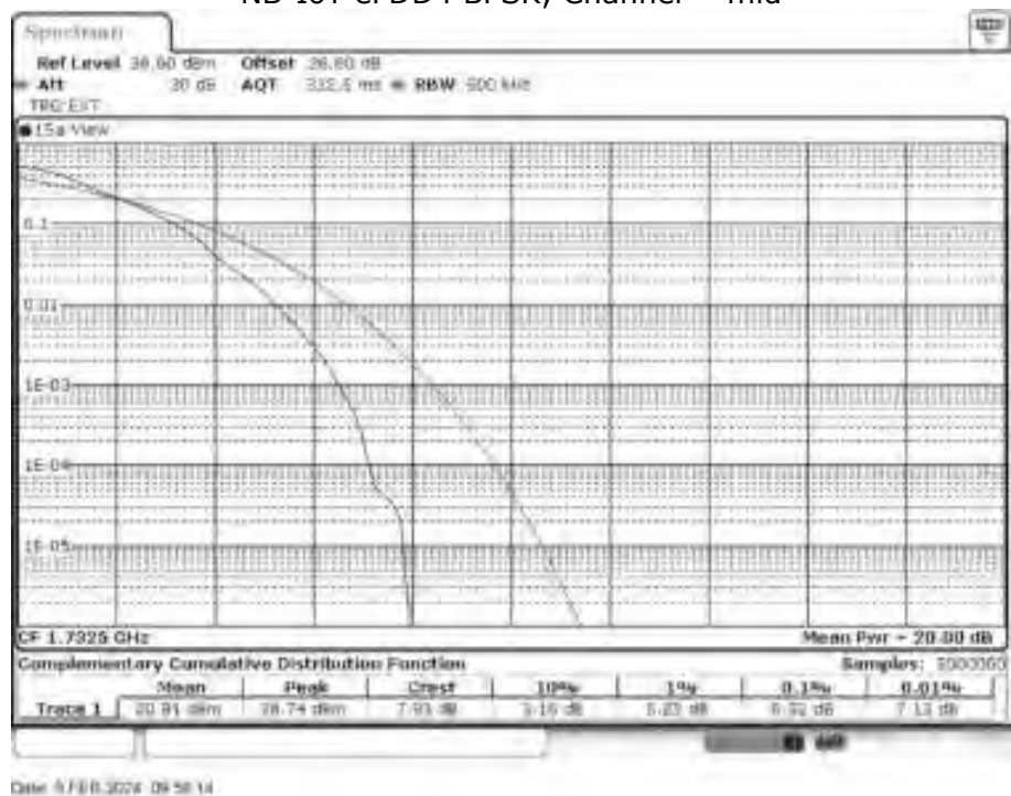
NB-IoT eFDD4 BPSK, Channel = mid
