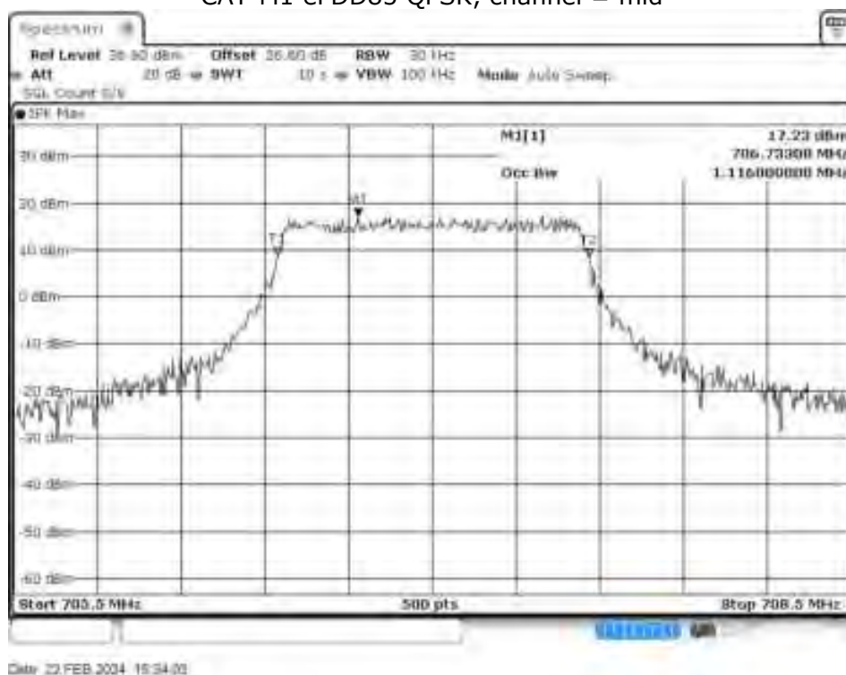
CAT-M1 eFDD85 QPSK, channel = mid
