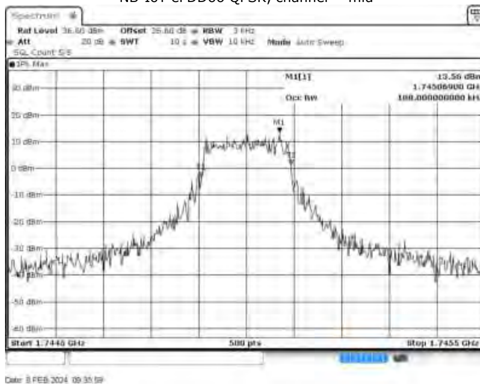
NB-IoT eFDD66 QPSK, channel = mid
