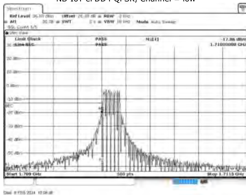
NB-IoT eFDD4 QPSK, Channel = low
