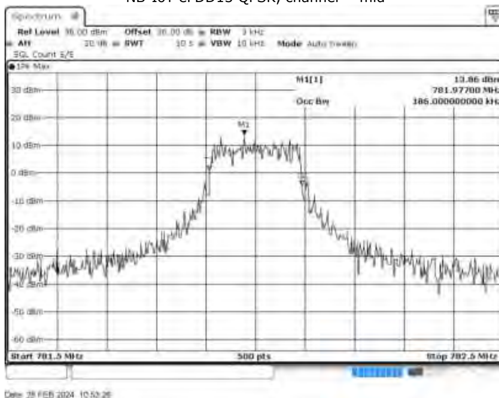
NB-IoT eFDD13 QPSK, channel = mid
