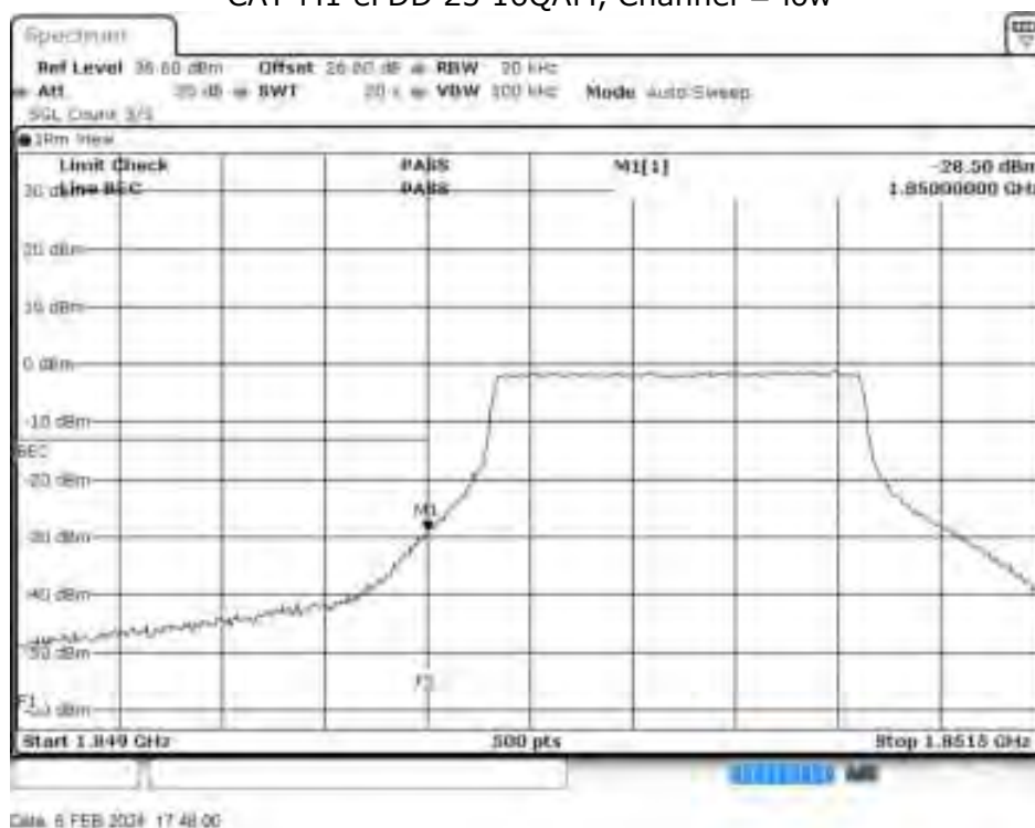
CAT-M1 eFDD 25 16QAM, Channel = low
