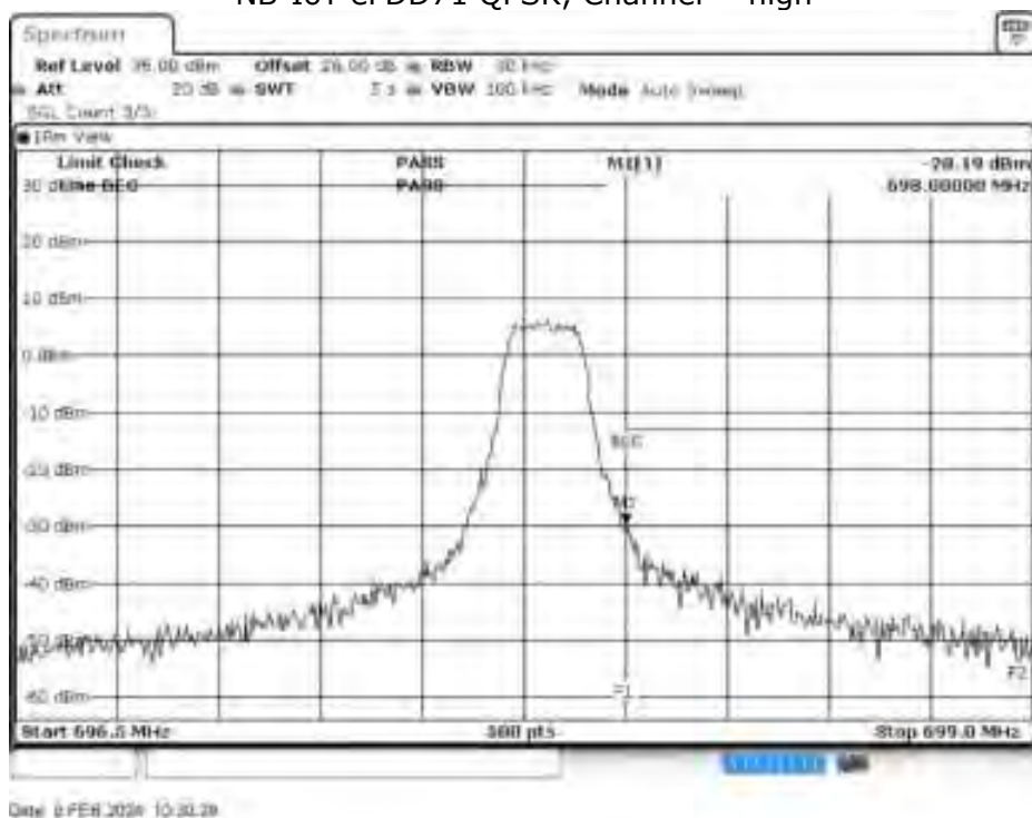
NB-IoT eFDD71 QPSK, Channel = high
