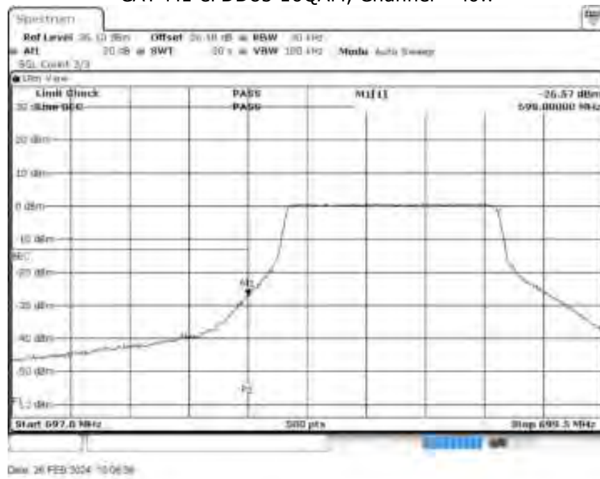
CAT-M1 eFDD85 16QAM, Channel = low
