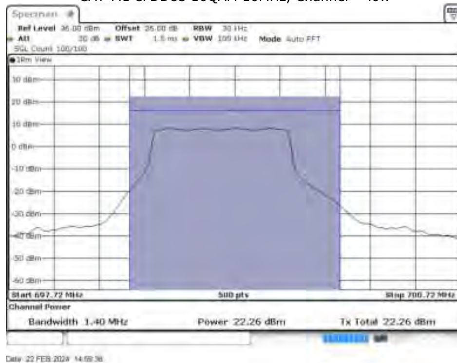
CAT-M1 eFDD85 16QAM 10MHz, Channel = low
