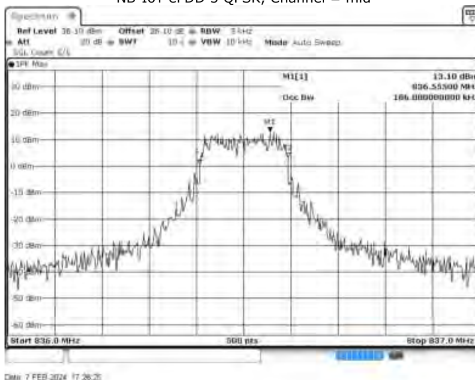
NB-IoT eFDD 5 QPSK, Channel = mid
