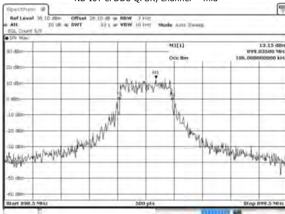
NB-IoT eFDD8 QPSK, channel = mid
