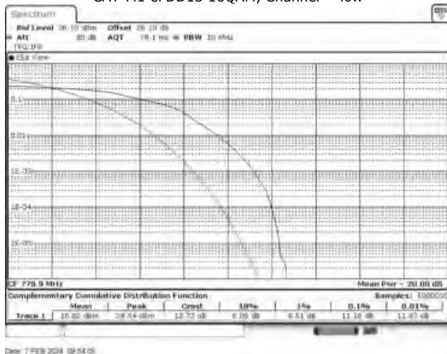
CAT-M1 eFDD13 16QAM, Channel = low
