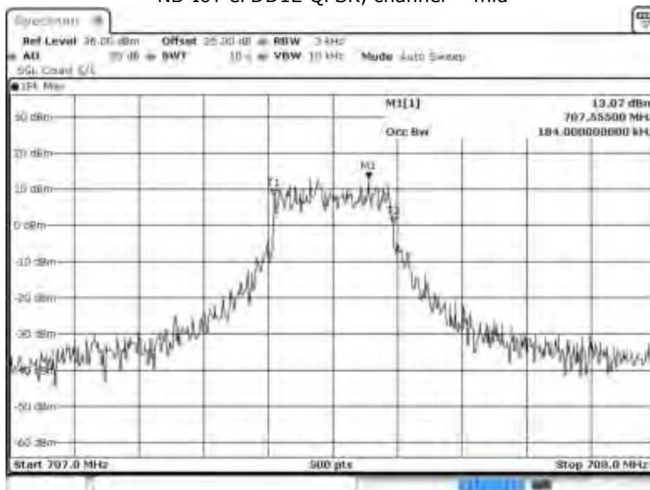
NB-IoT eFDD12 QPSK, channel = mid
