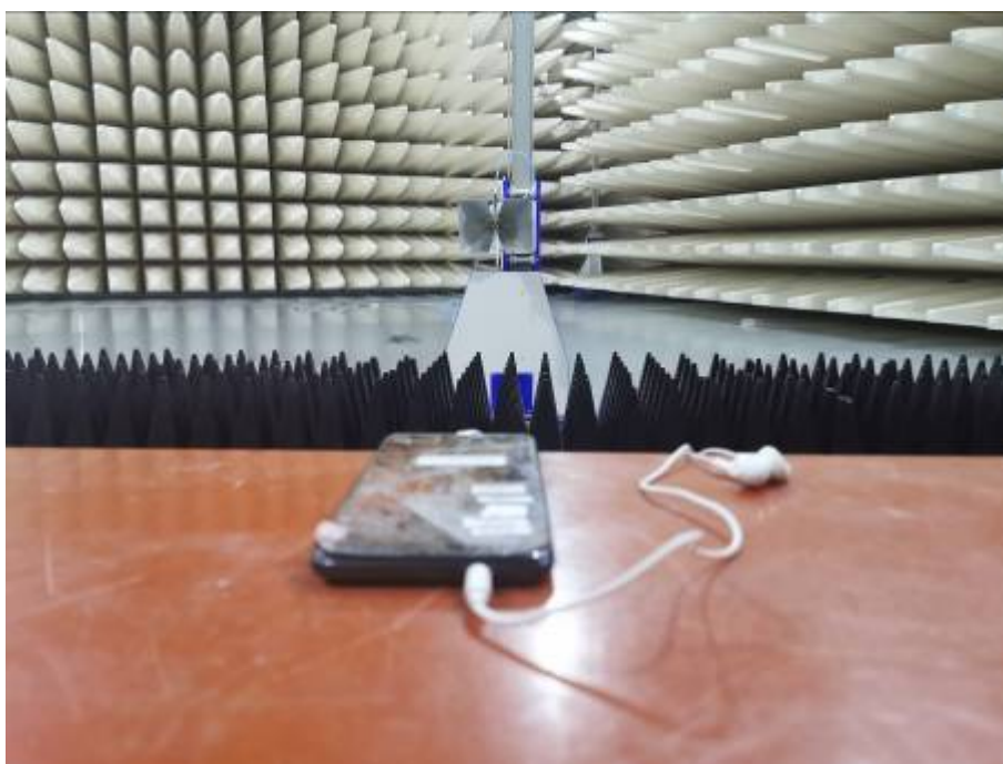
Radiated Emissions Test Setup (with charger) (above 1GHz)
