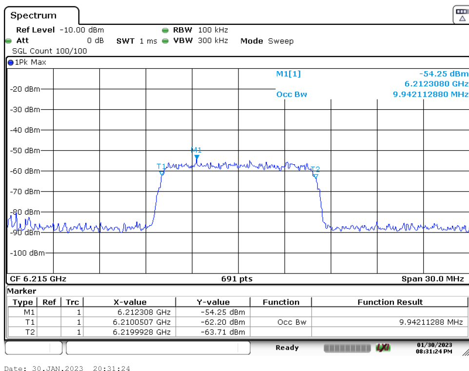
Plot 7-100. AWGN Signal (Demonstration)
