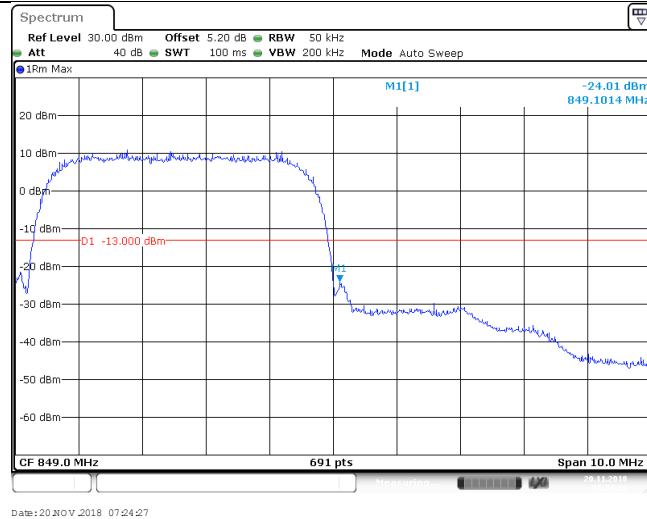
Band V_16QAM_4233
