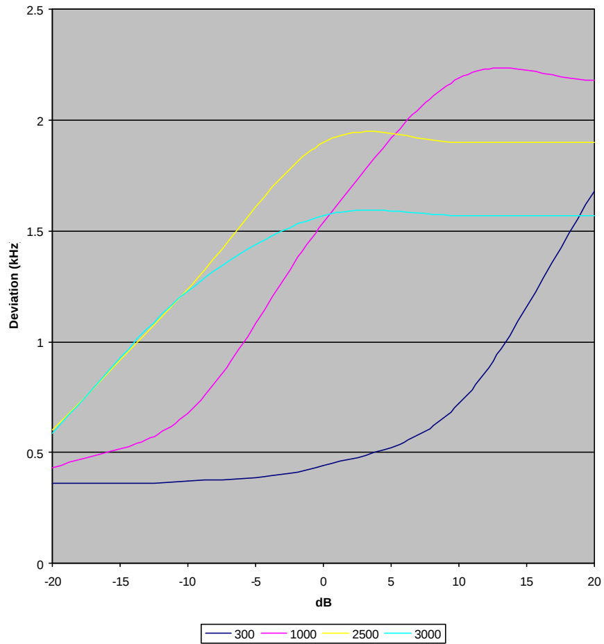
Modulation Limiting (467.525 MHz; 12.5 kHz channel spacing; Negative Peak)
